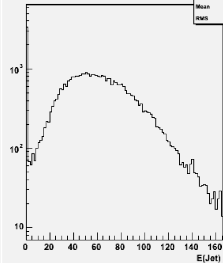
Jet energies(All jets)w101016 ddn2e2e1n1_o
