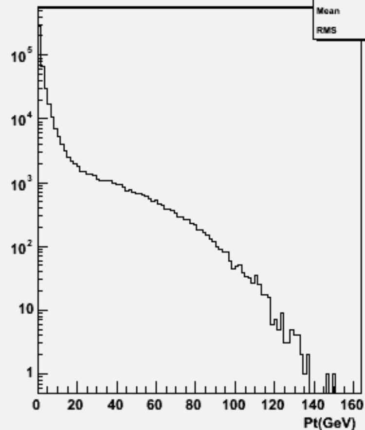
Start point Z : w101016 ddn2e2e1n1_o
