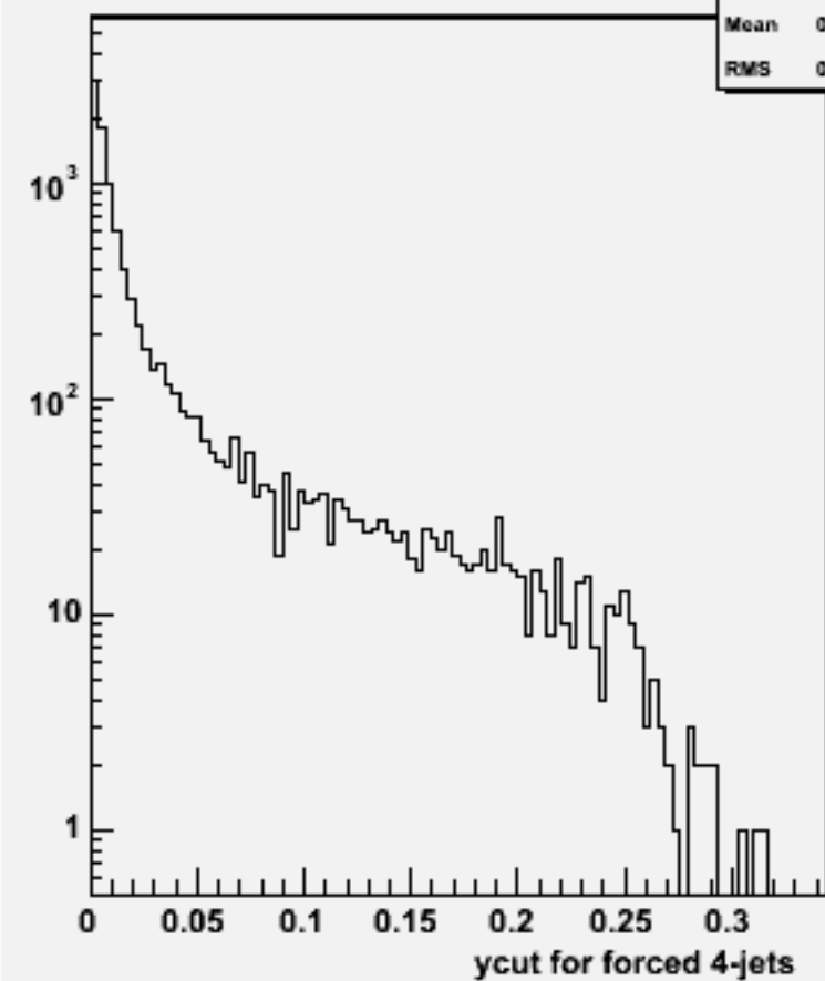
Ycut for 4-jets :w101016 ddn2e2e1n1_o
