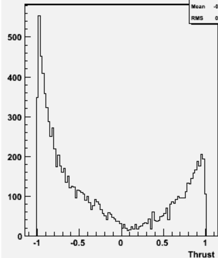
cos \Theta (thrust) w101016 ddn2e2e1n1_o
