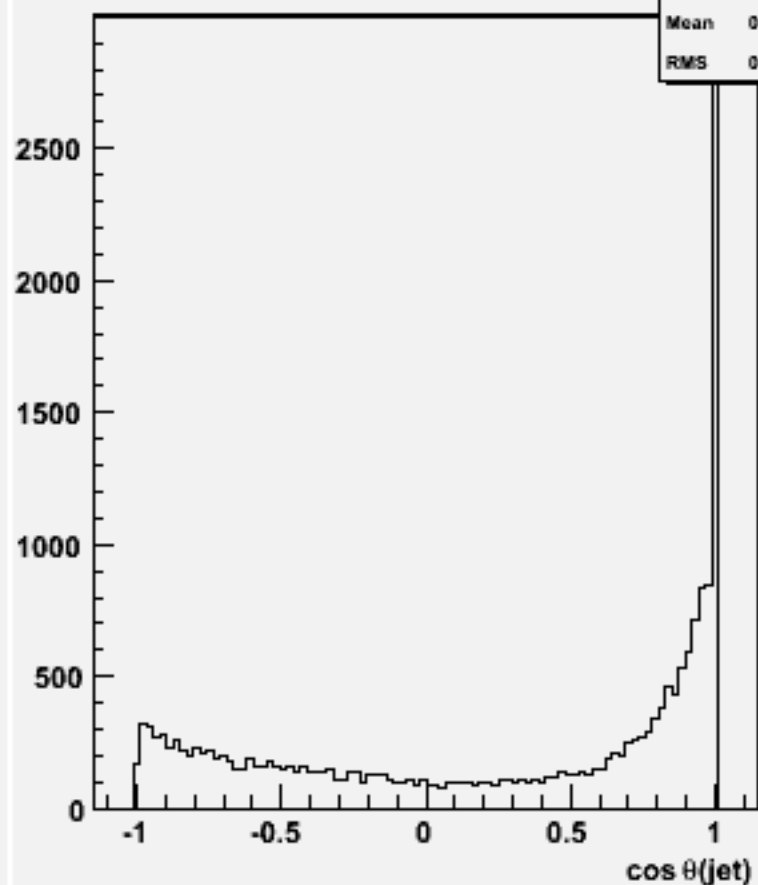
cos \theta for 2-jets :w101016 ddn2e2e1n1_o
