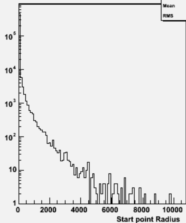
Start point R : w101016 ddn2e2e1n1_o
