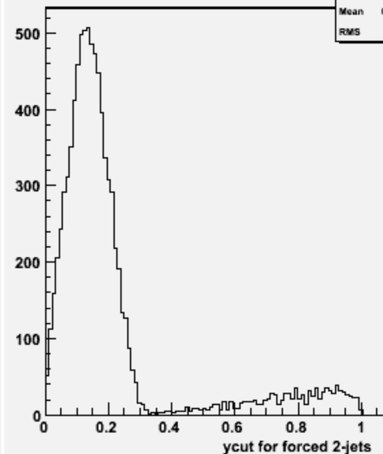
Ycut for 2-jets :w101016 ddn2e2e1n1_o
