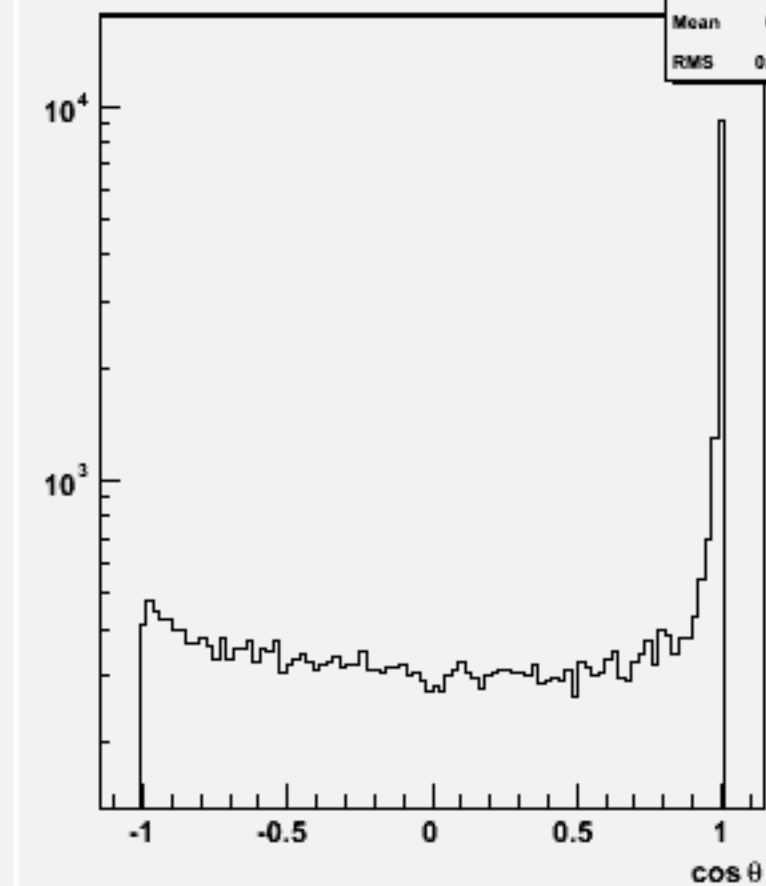
Jet cos \theta (All jets)w101016 ddn2e2e1n1_o
