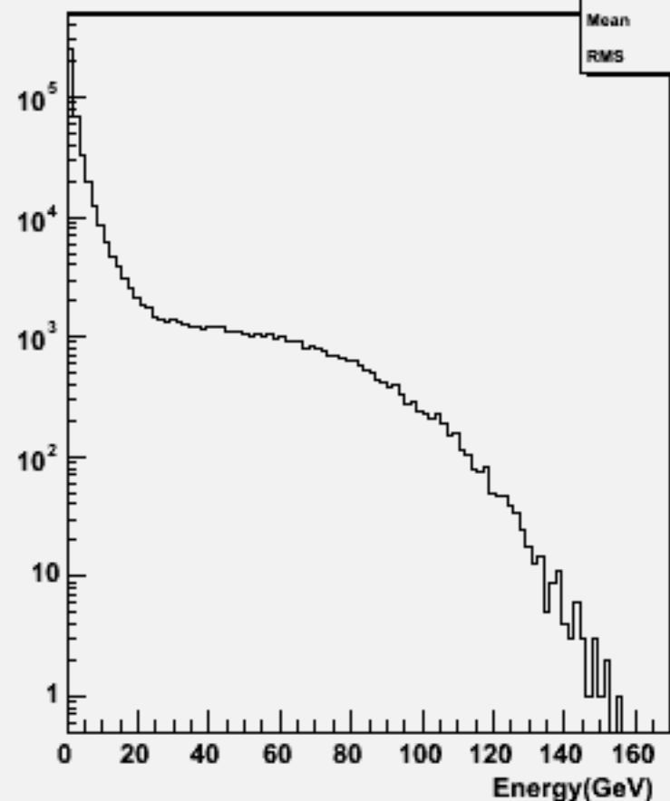
Start point R : w101016 ddn2e2e1n1_o
