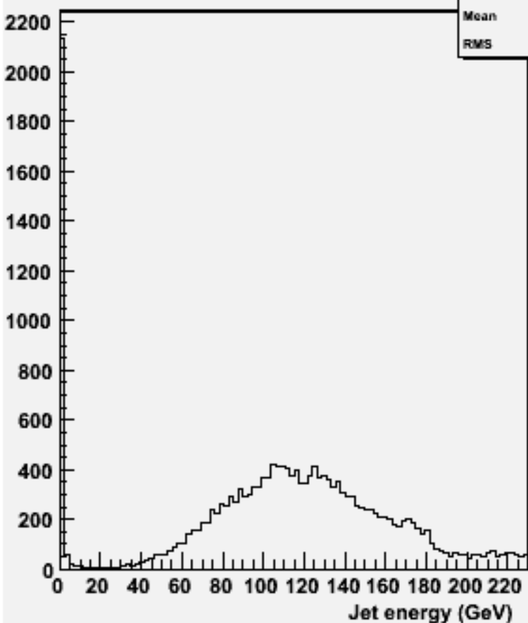
energy for 2-jets :w101016 ddn2e2e1n1_o
