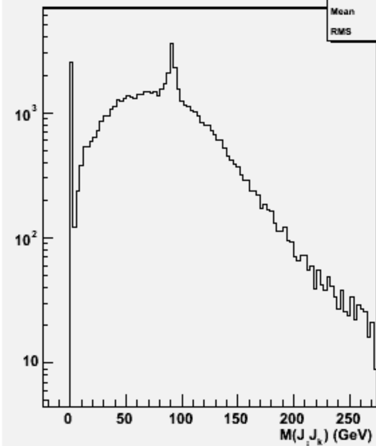
2jets mass(All comb)w101016 ddn2e2e1n1_o
