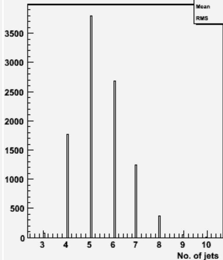
No. jets (ycut=0.001) : w101016 ddn2e2e1n1_o
