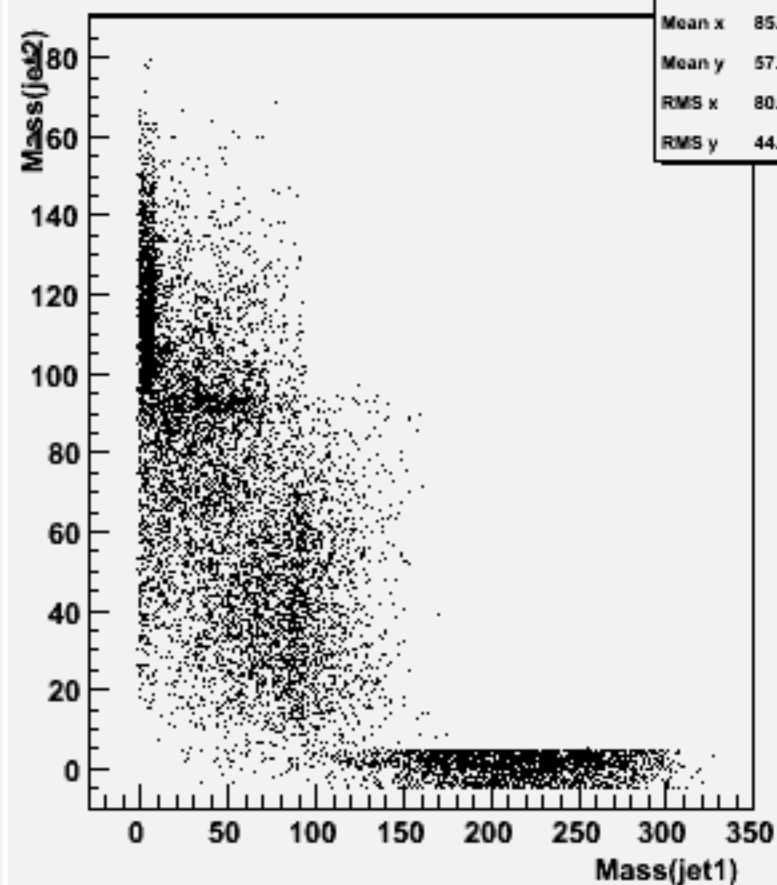
Jet mass for forced 2-jets : w101016 ddn2e2e1n1_o
