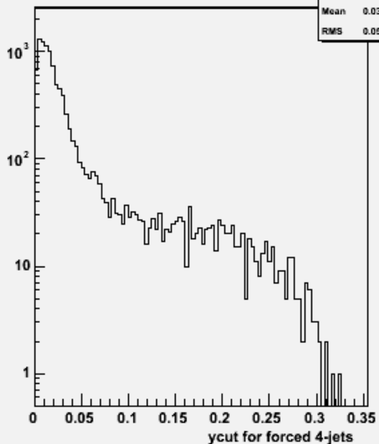
Ycut for 4-jets :w101013 ddn1e1sc_o
