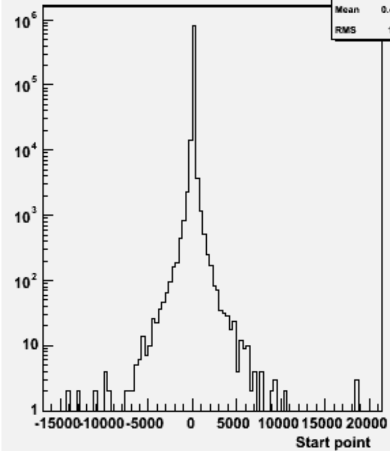
Start point Z : w101013 ddn1e1sc_o
