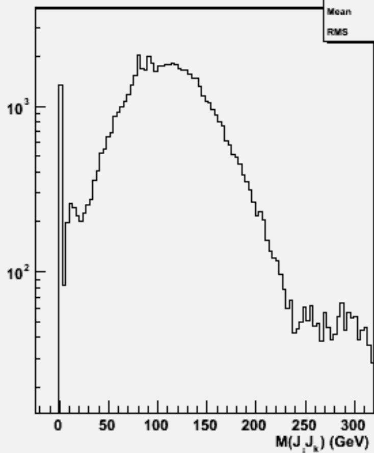
2jets mass(All comb)w101013 ddn1e1sc_o
