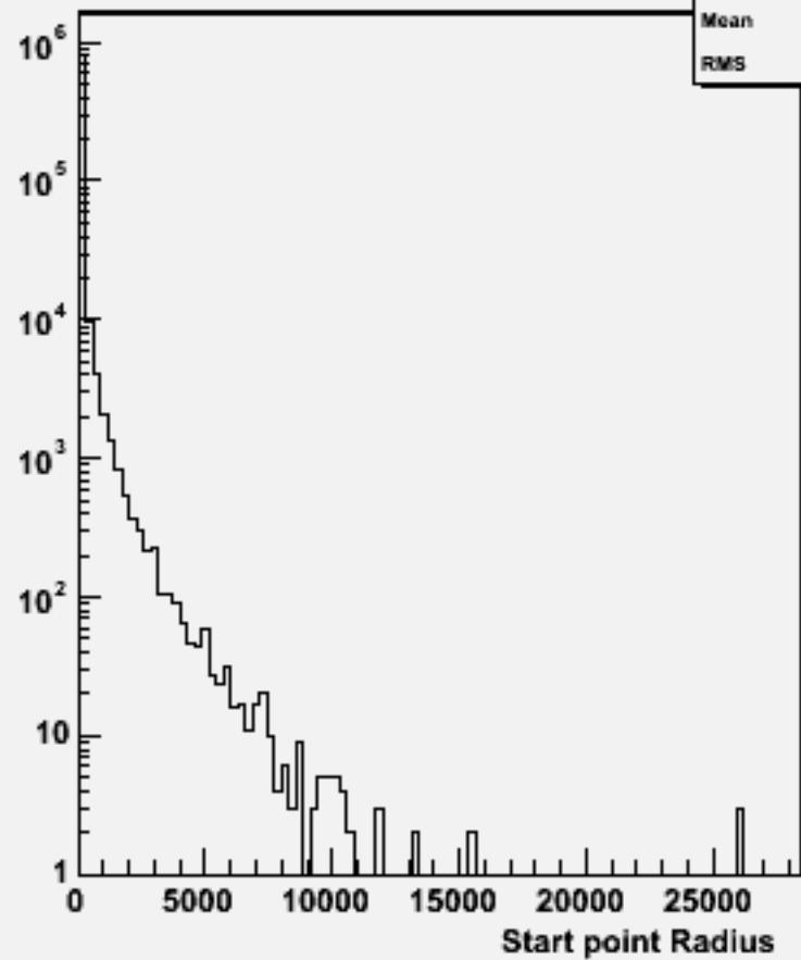
Start point R : w101013 ddn1e1sc_o
