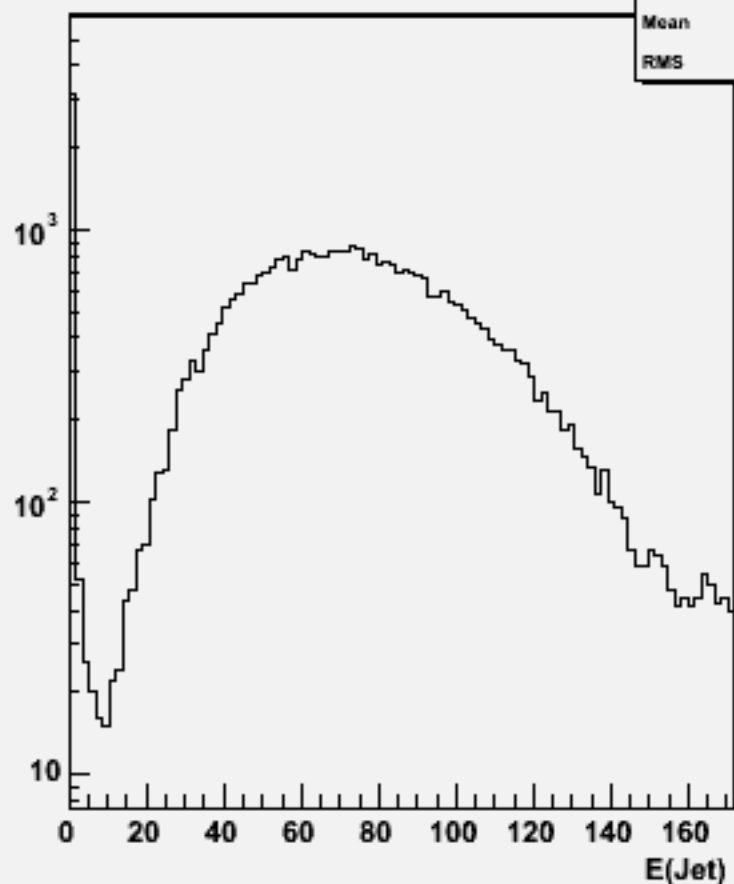
Jet energies(All jets)w101013 ddn1e1sc_o
