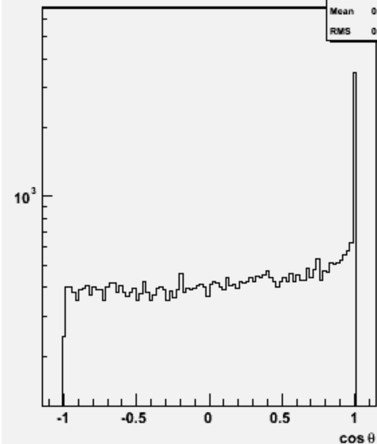
Jet cos \theta (All jets)w101013 ddn1e1sc_o
