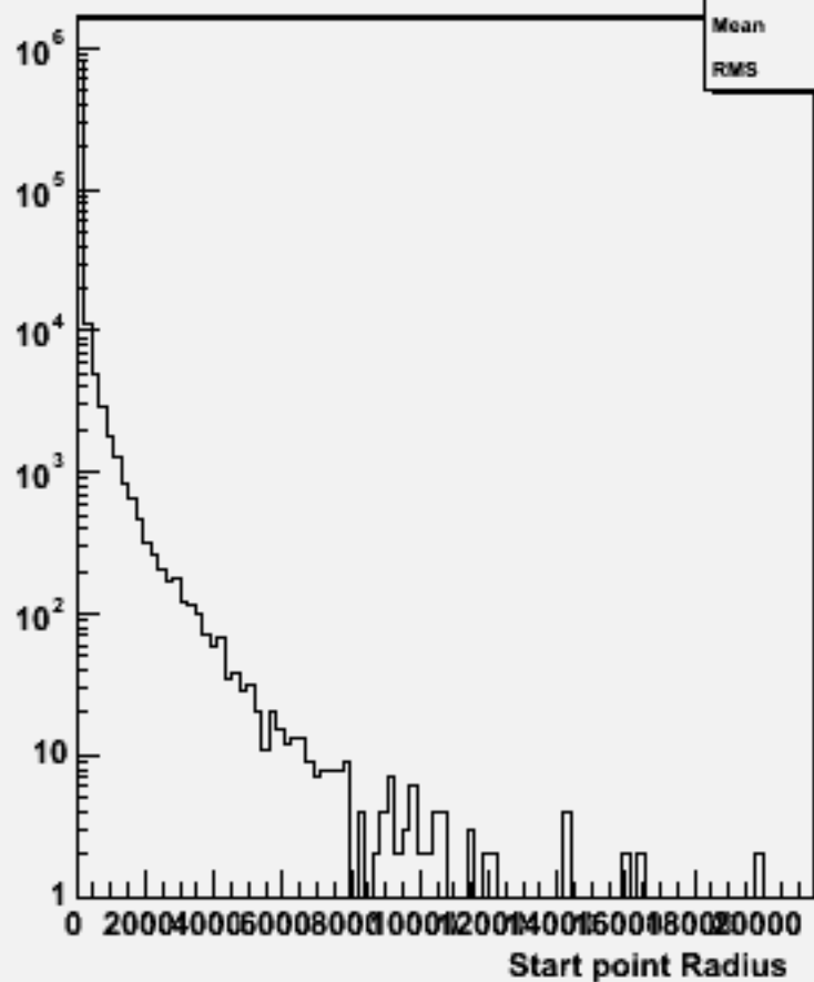
Start point R : w101012 ddn1e1sc_o
