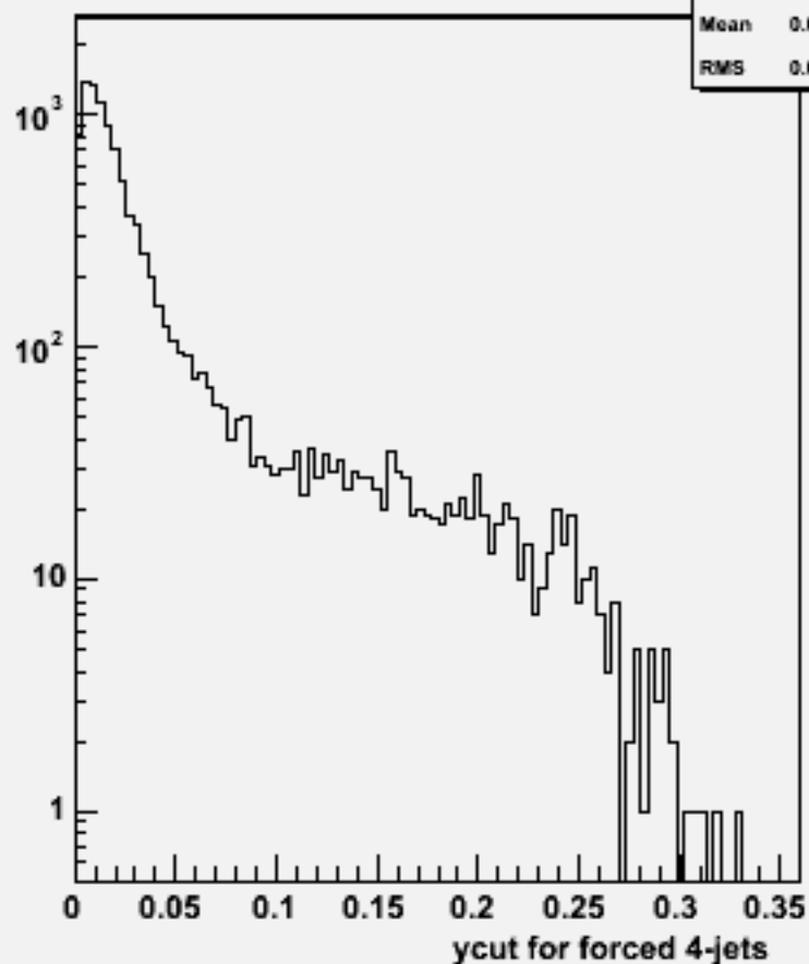
Ycut for 4-jets :w101012 ddn1e1sc_o
