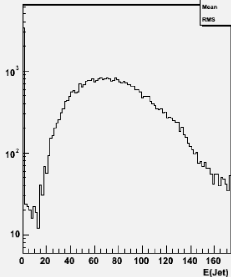
Jet energies(All jets)w101012 ddn1e1sc_o
