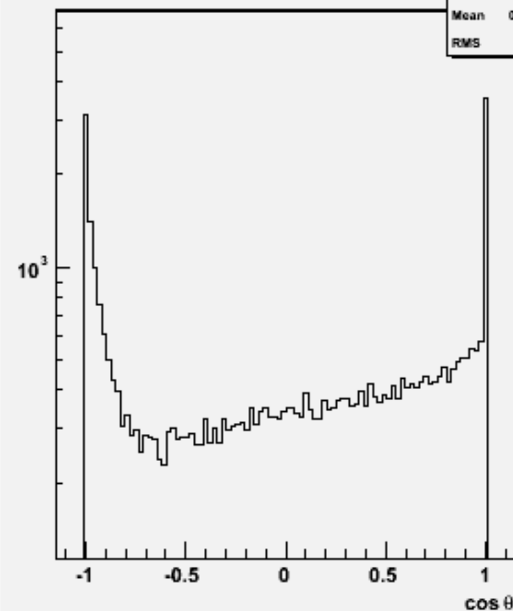
Jet cos \theta (All jets)w101012 ddn1e1sc_o
