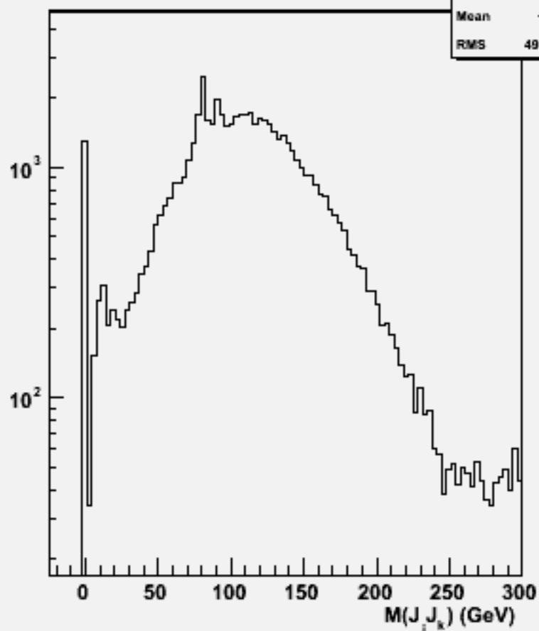
2jets mass(All comb)w101012 ddn1e1sc_o
