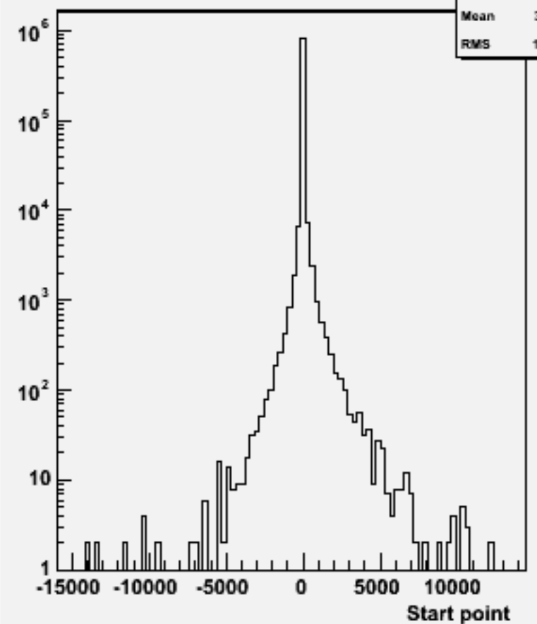
Start point Z : w101012 ddn1e1sc_o
