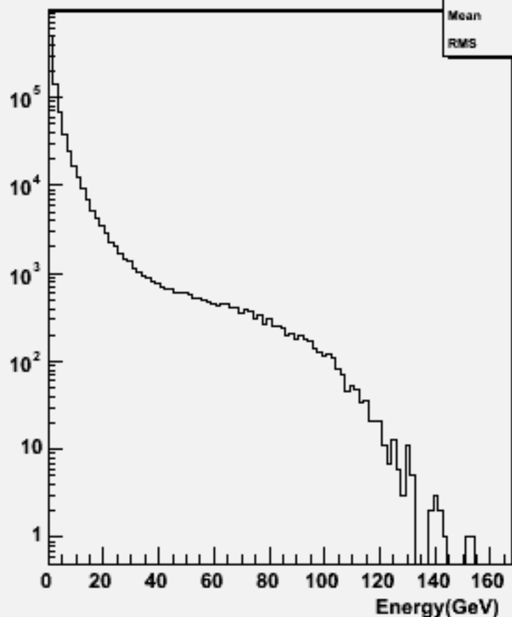
Particle Energy : w101012 ddn1e1sc_o
