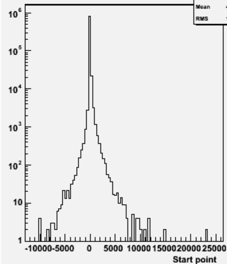
Start point Z : w101011 ddn1e1sc_o
