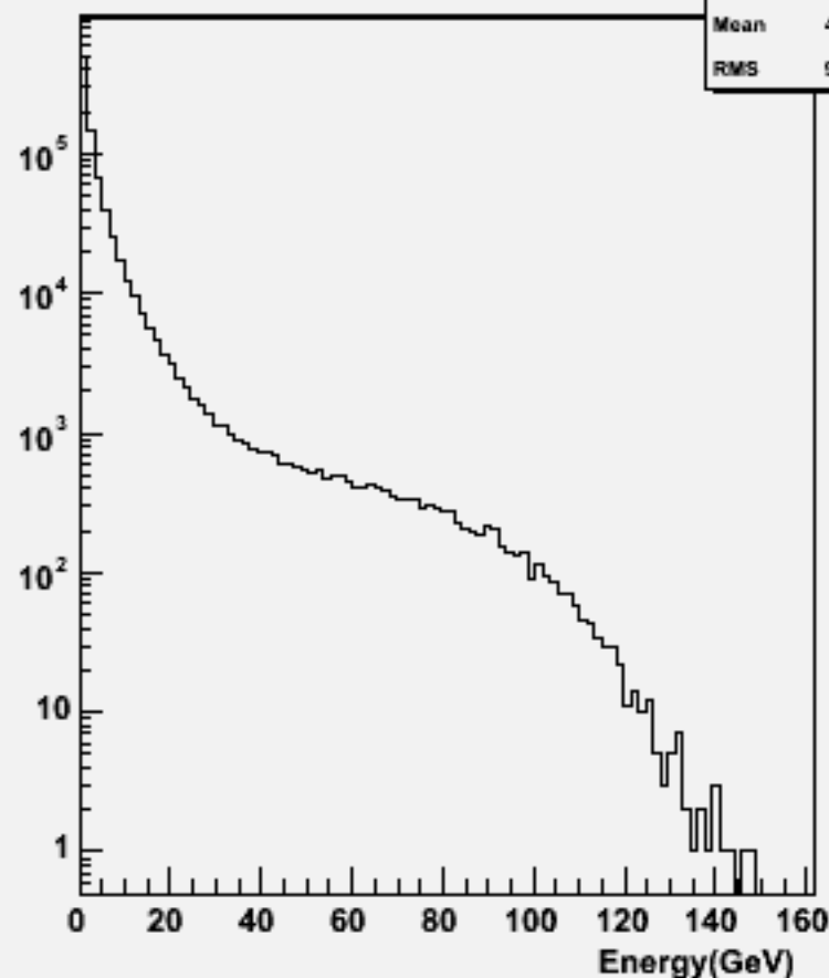
Particle Energy : w101011 ddn1e1sc_o
