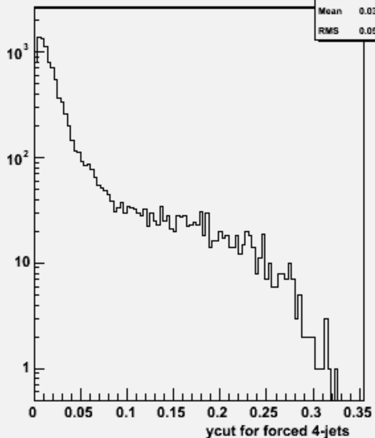
Ycut for 4-jets :w101011 ddn1e1sc_o
