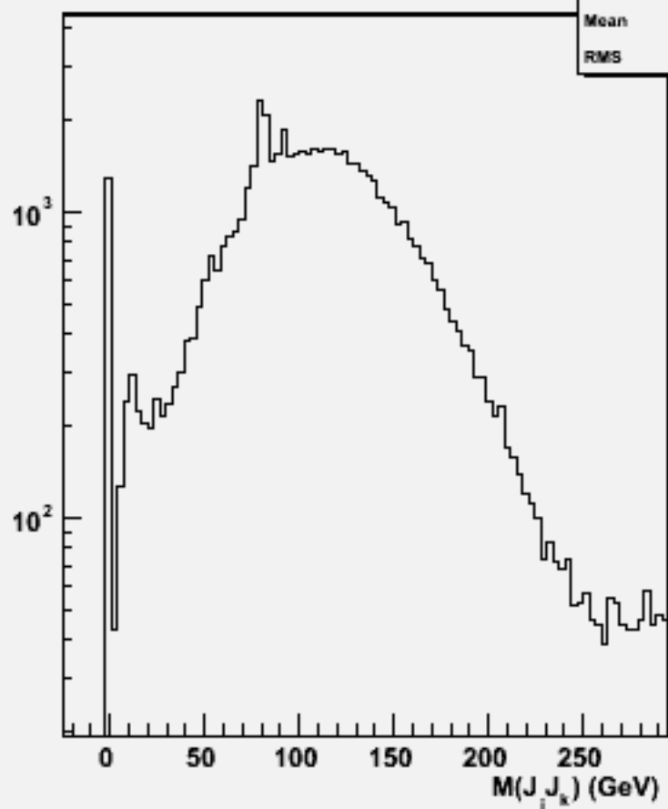
2jets mass(All comb)w101011 ddn1e1sc_o
