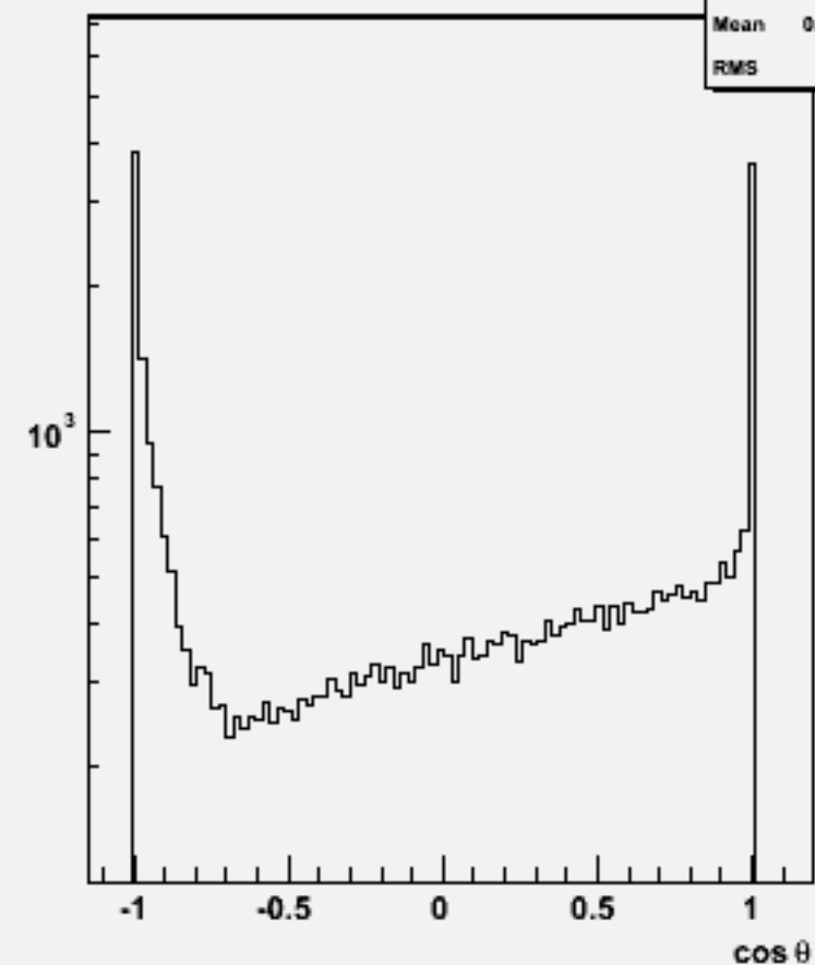
Jet cos \theta (All jets)w101011 ddn1e1sc_o
