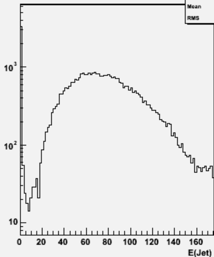
Jet energies(All jets)w101011 ddn1e1sc_o
