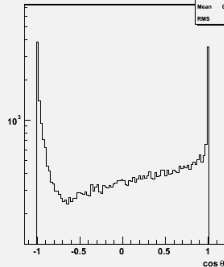
Jet cos \theta (All jets)w101007 ddn1e1du_o
