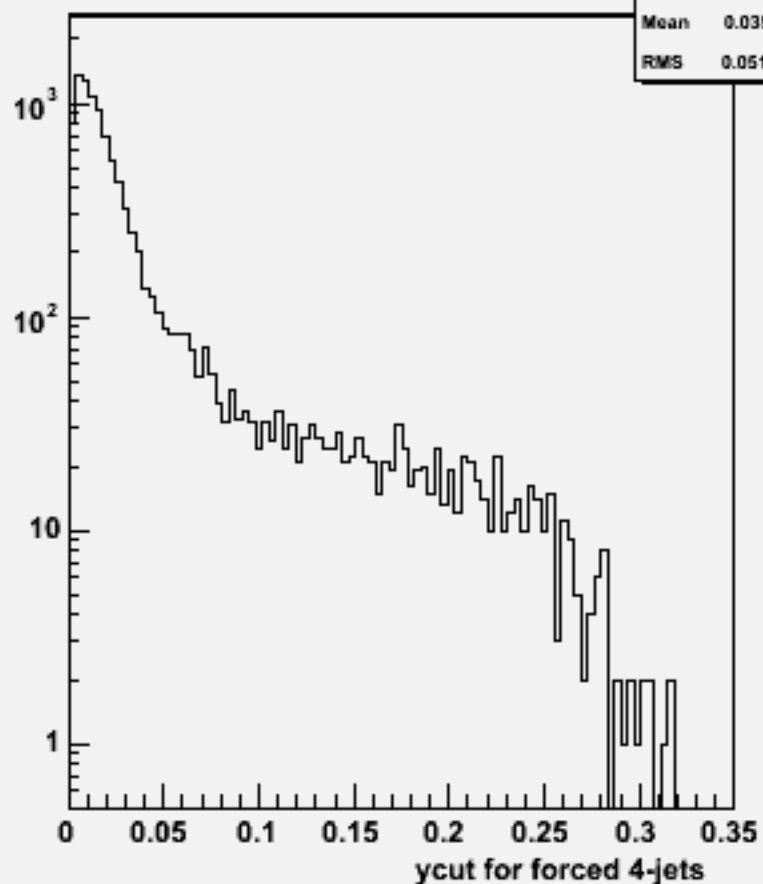
Ycut for 4-jets :w101007 ddn1e1du_o
