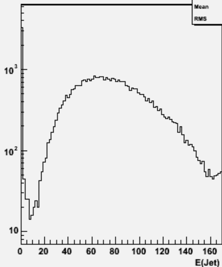
Jet energies(All jets)w101007 ddn1e1du_o
