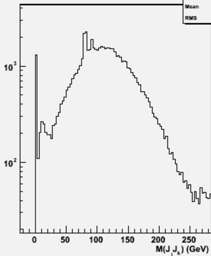
2jets mass(All comb)w101007 ddn1e1du_o
