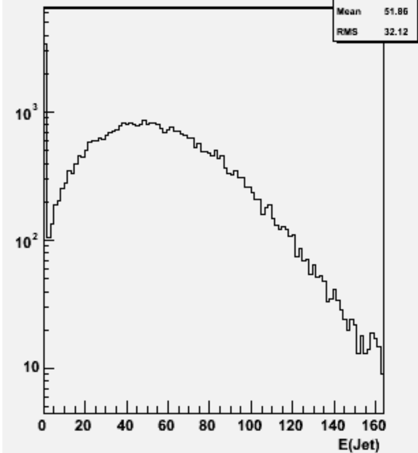
Jet energies(All jets)w101004 ddn1e1e3n3_o
