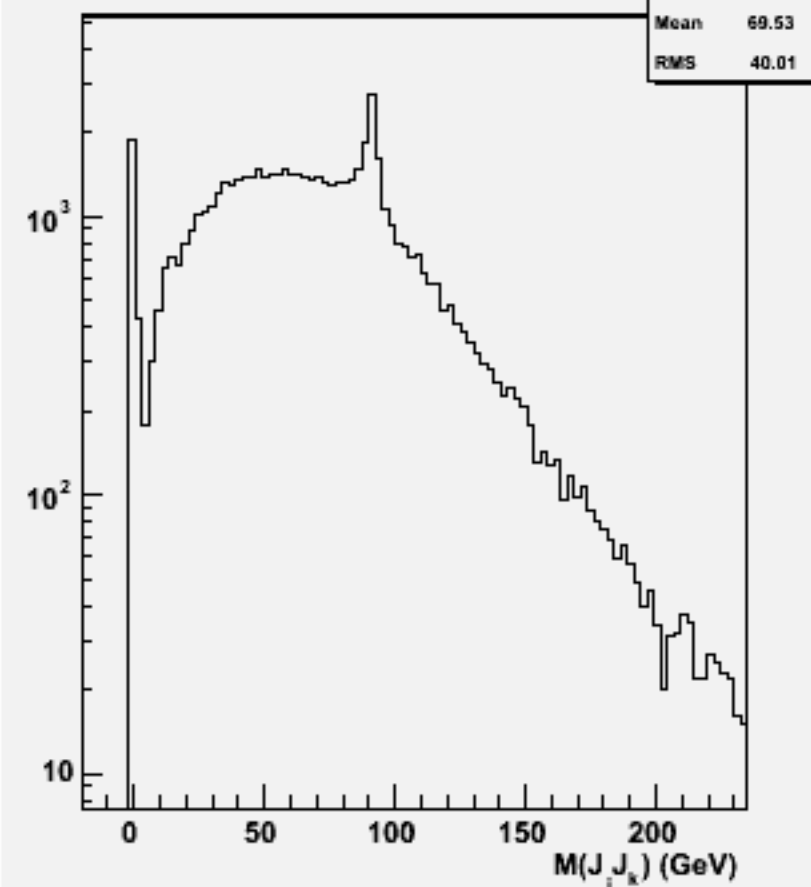
2jets mass(All comb)w101004 ddn1e1e3n3_o
