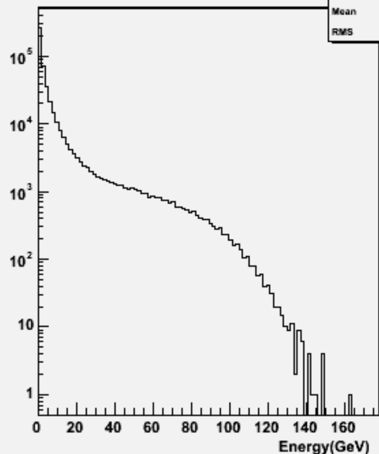
Particle Energy : w101004 ddn1e1e3n3_o
