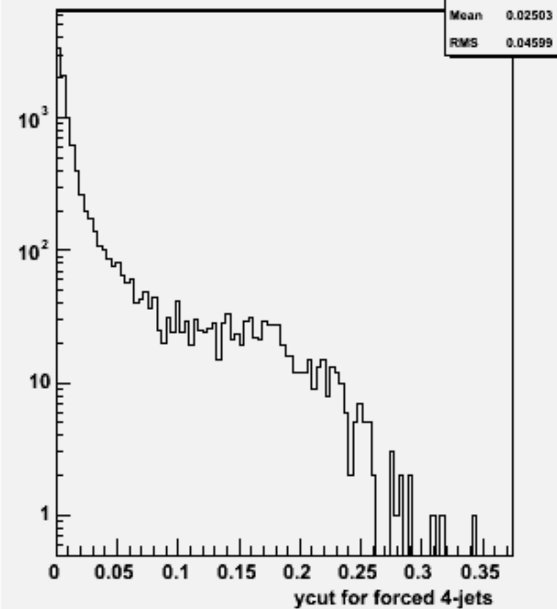
Ycut for 4-jets :w101004 ddn1e1e3n3_o
