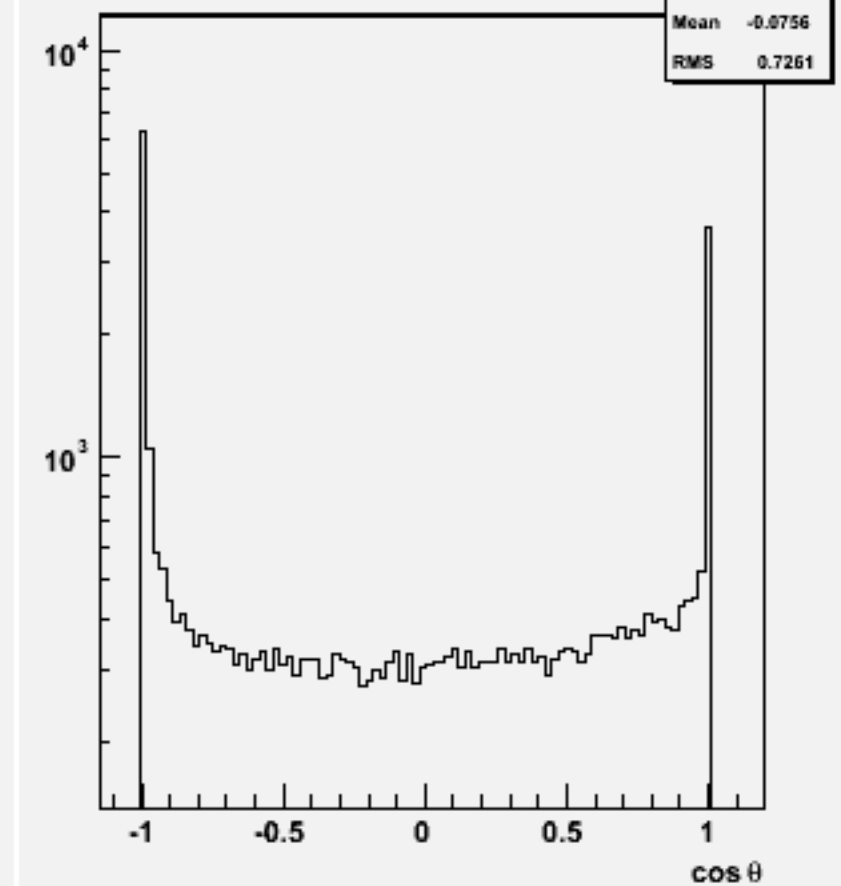
Jet cos \theta (All jets)w101004 ddn1e1e3n3_o
