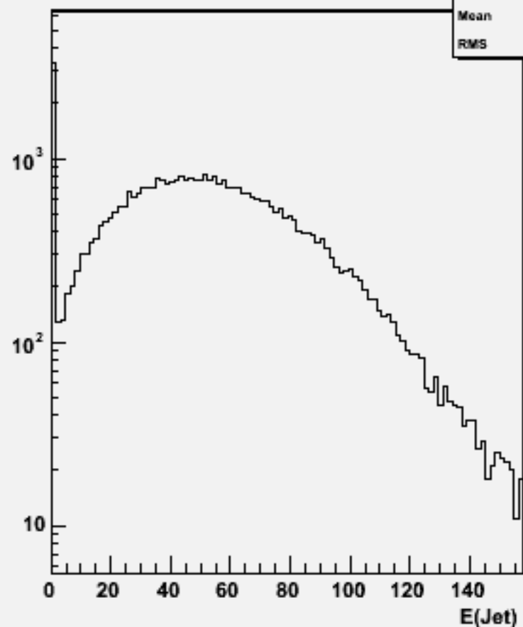
Jet energies(All jets)w101003 ddn1e1e3n3_o
