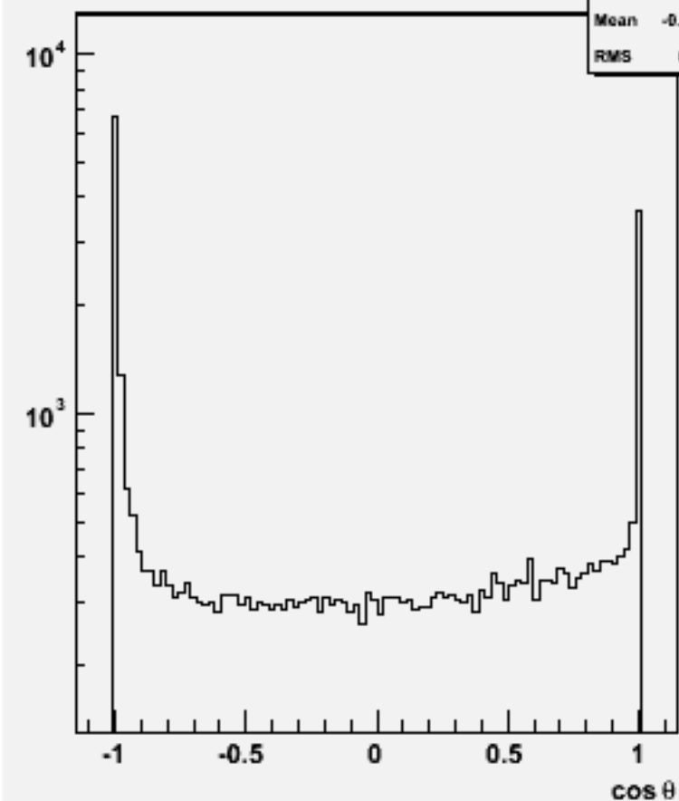
Jet cos \theta (All jets)w101003 ddn1e1e3n3_o
