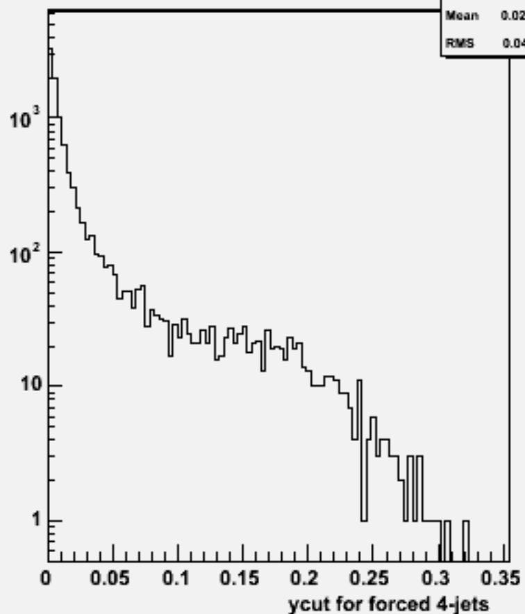
Ycut for 4-jets :w101003 ddn1e1e3n3_o
