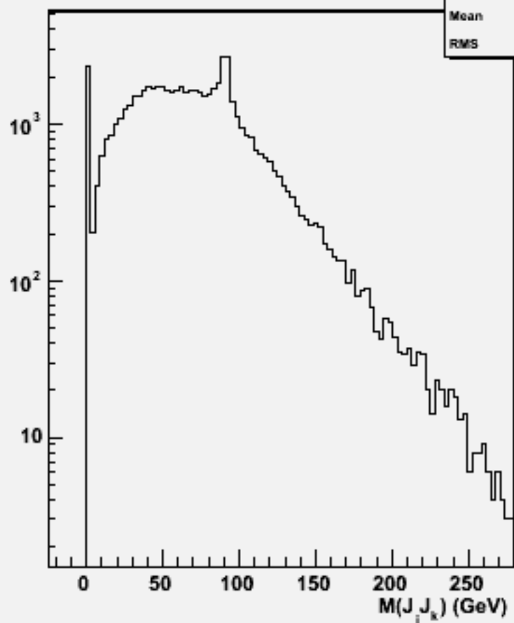
2jets mass(All comb)w101003 ddn1e1e3n3_o
