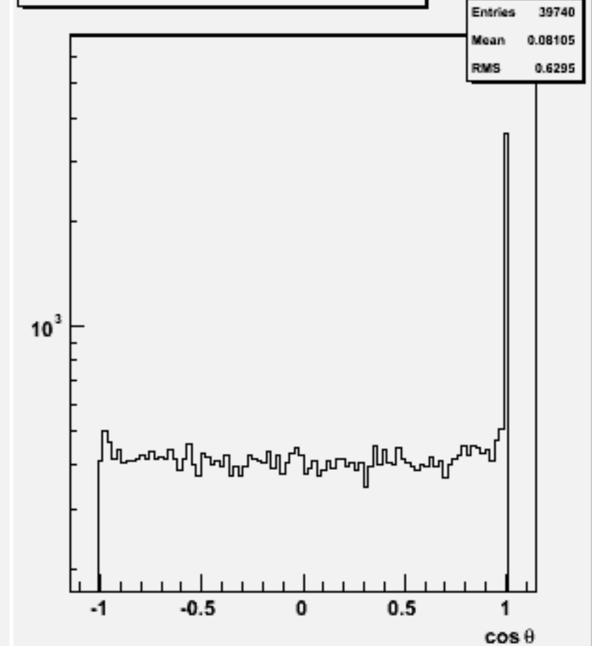
Jet cos \theta (All jets)w101001 ddn1e1e2n2_o
