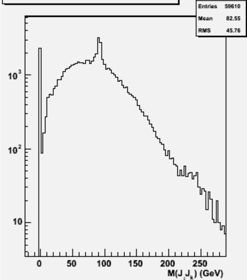
2jets mass(All comb)w101001 ddn1e1e2n2_o
