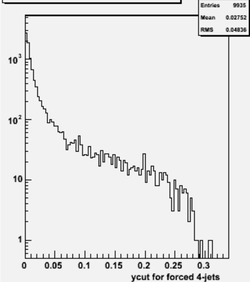
Ycut for 4-jets :w101001 ddn1e1e2n2_o
