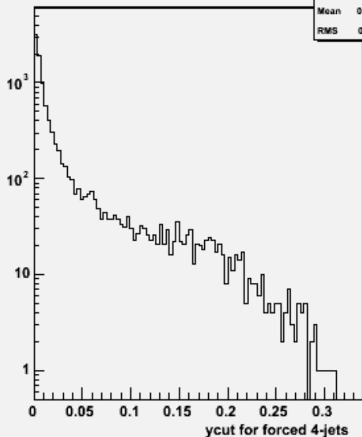
Ycut for 4-jets :w100999 ddn1e1e2n2_o
