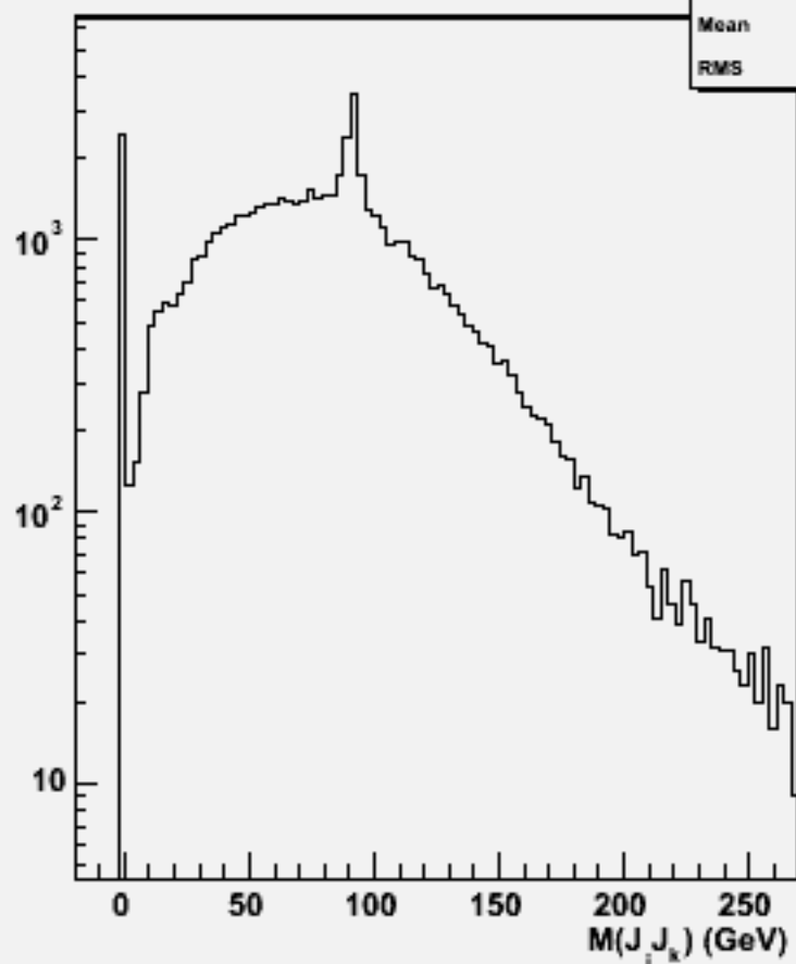
2jets mass(All comb)w100999 ddn1e1e2n2_o
