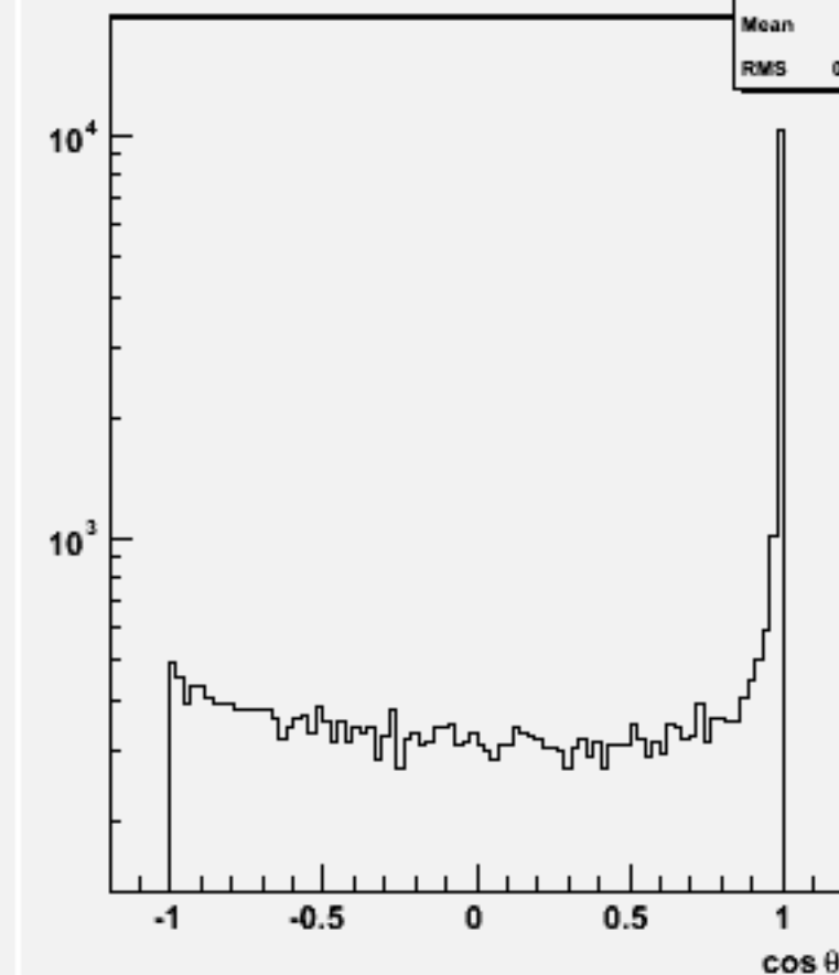
Jet cos \theta (All jets)w100998 ddn1e1e1n1_o
