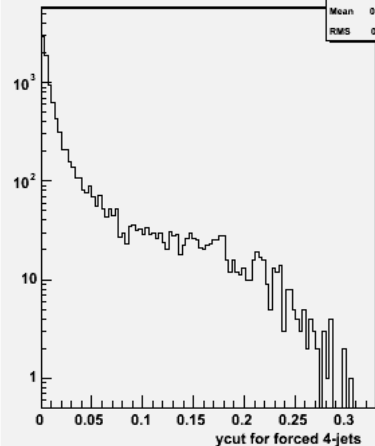
Ycut for 4-jets :w100998 ddn1e1e1n1_o
