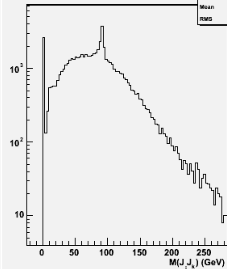
2jets mass(All comb)w100998 ddn1e1e1n1_o
