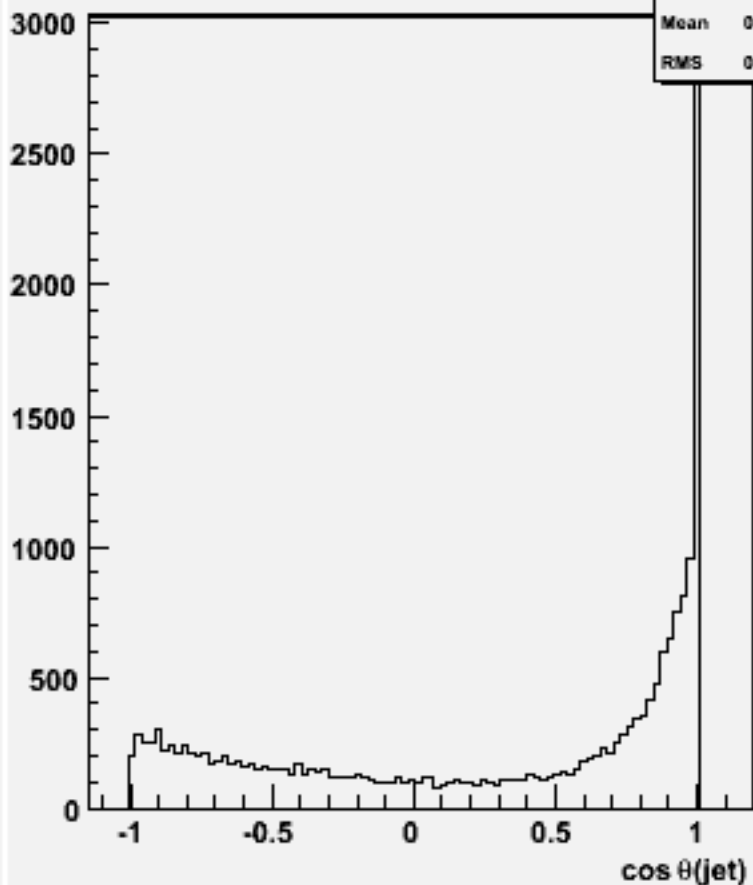
cos \theta for 2-jets :w100998 ddn1e1e1n1_o
