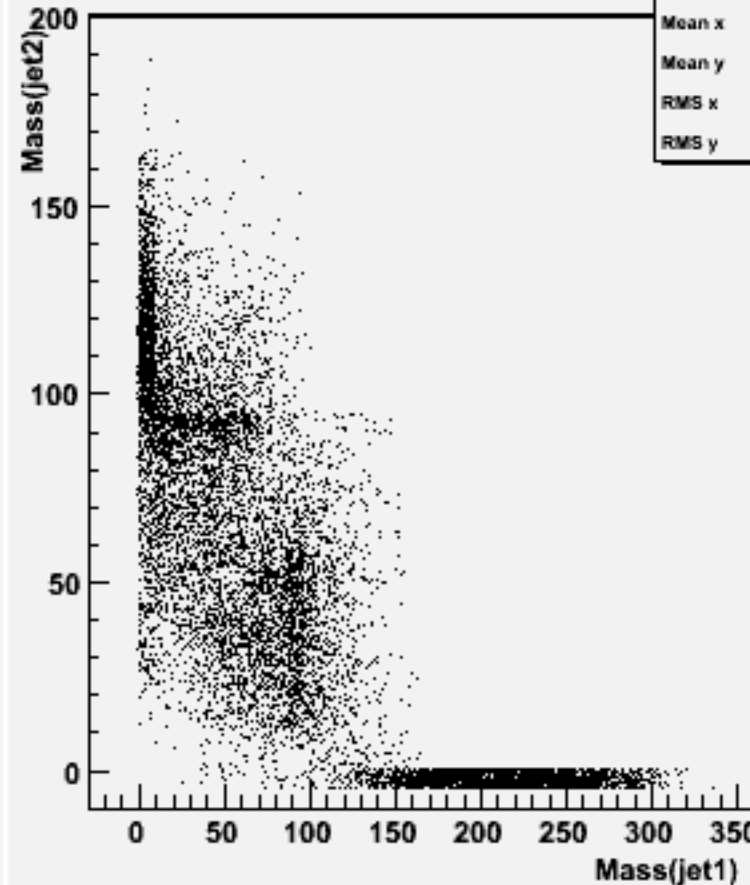
Jet mass for forced 2-jets : w100998 ddn1e1e1n1_o
