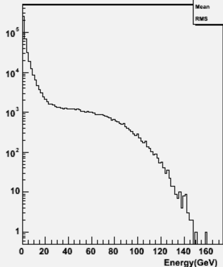
Start point R : w100998 ddn1e1e1n1_o
