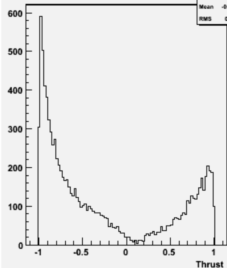
cos \Theta (thrust) w100998 ddn1e1e1n1_o
