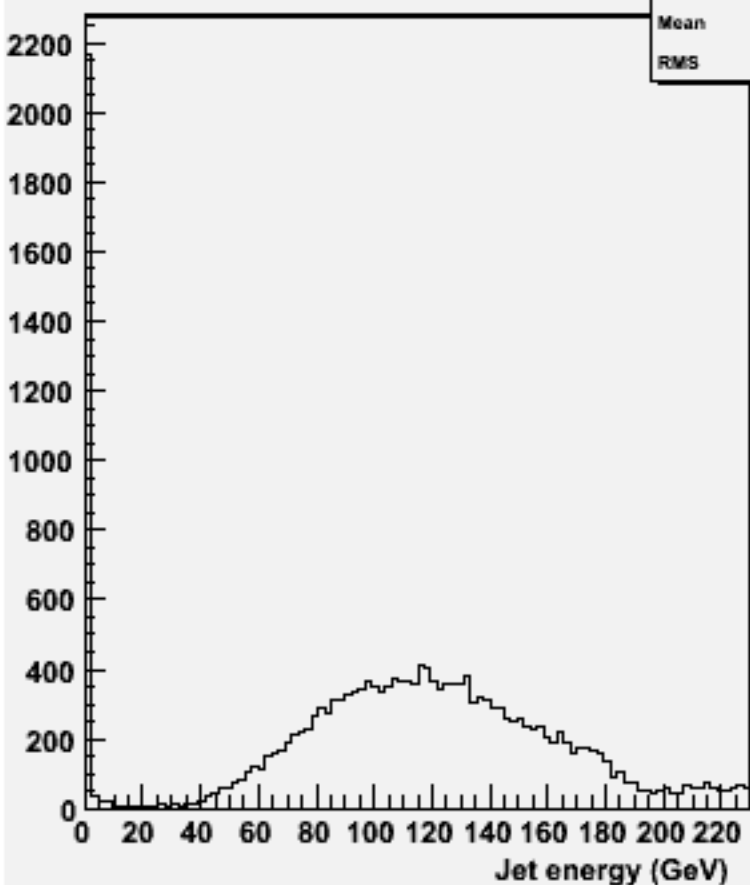
energy for 2-jets :w100998 ddn1e1e1n1_o
