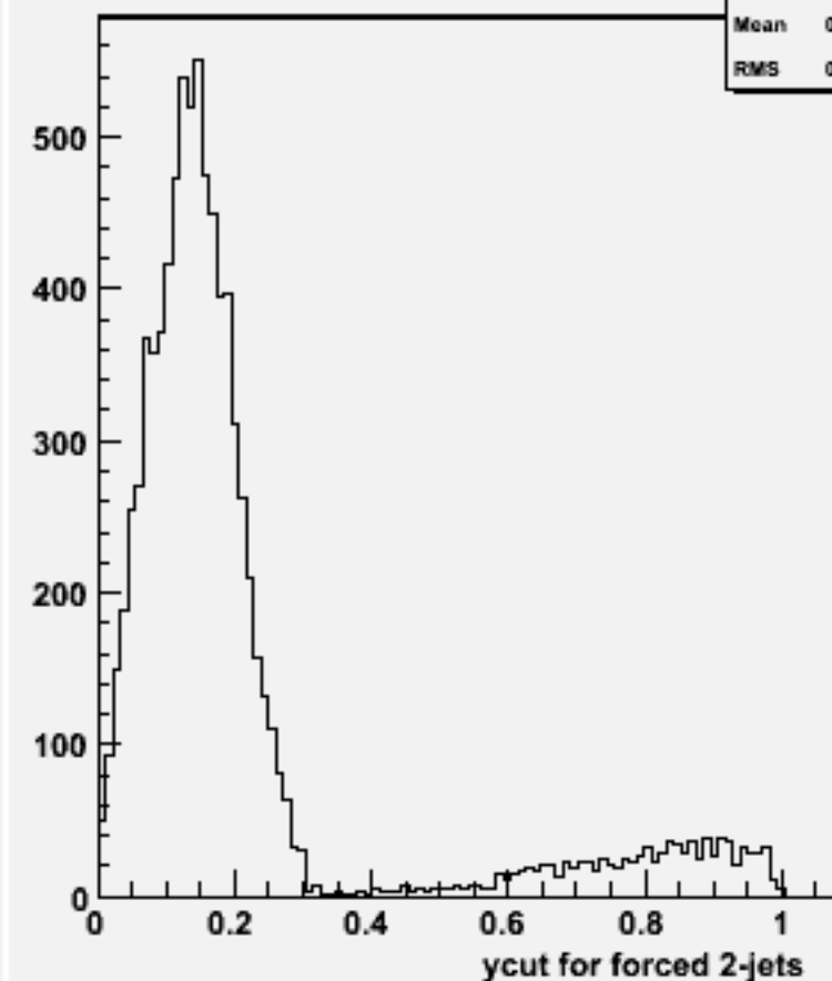
Ycut for 2-jets :w100998 ddn1e1e1n1_o
