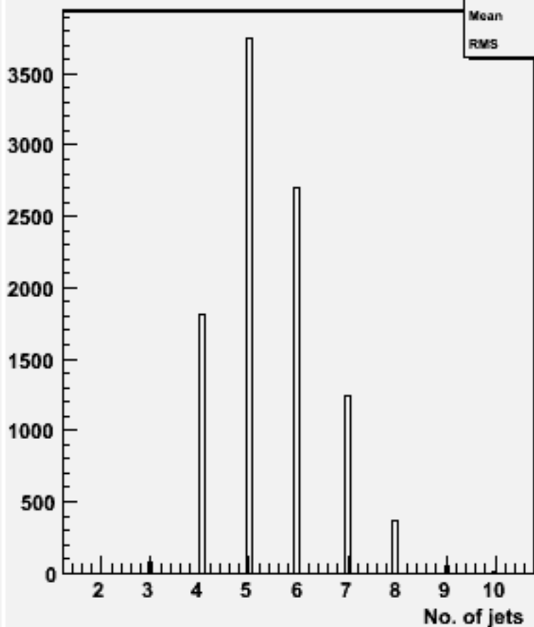
No. jets (ycut=0.001) : w100998 ddn1e1e1n1_o
