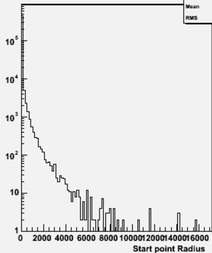
Start point R : w100998 ddn1e1e1n1_o
