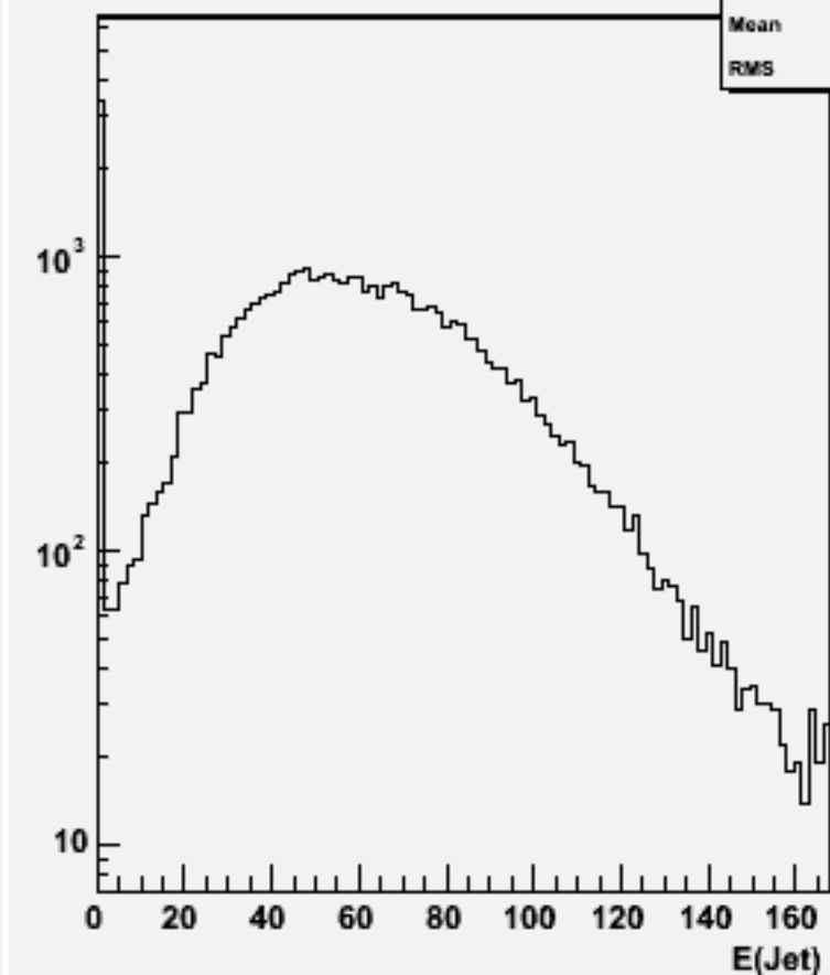
Jet energies(All jets)w100998 ddn1e1e1n1_o
