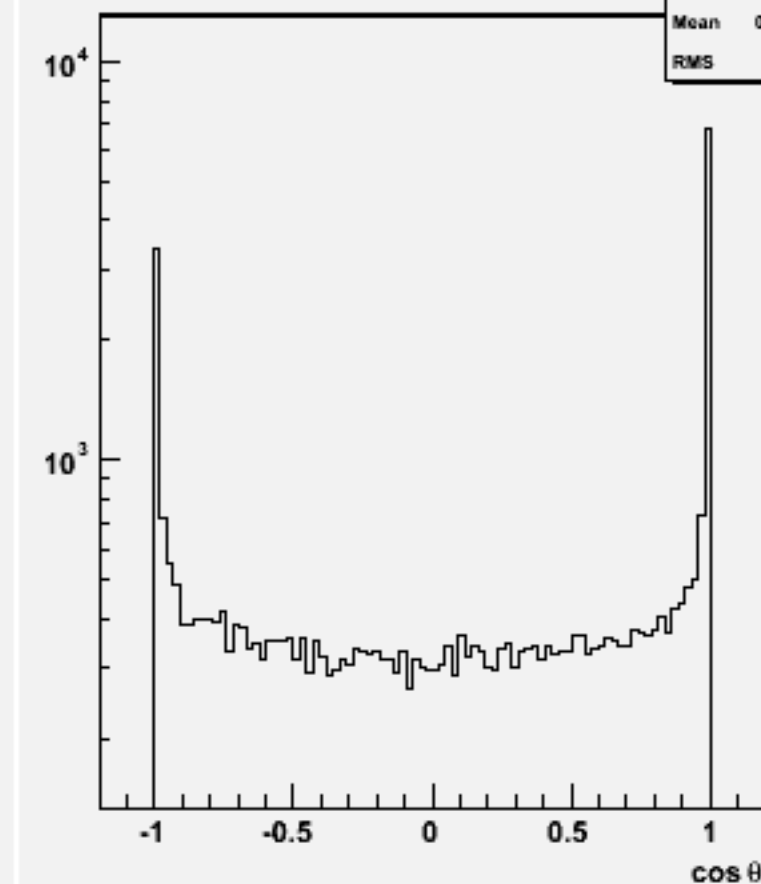
Jet cos \theta (All jets)w100996 ddn1e1e1n1_o
