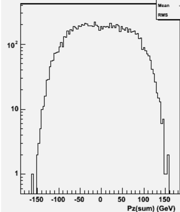
Pz Sum: w100996 ddn1e1e1n1_o
