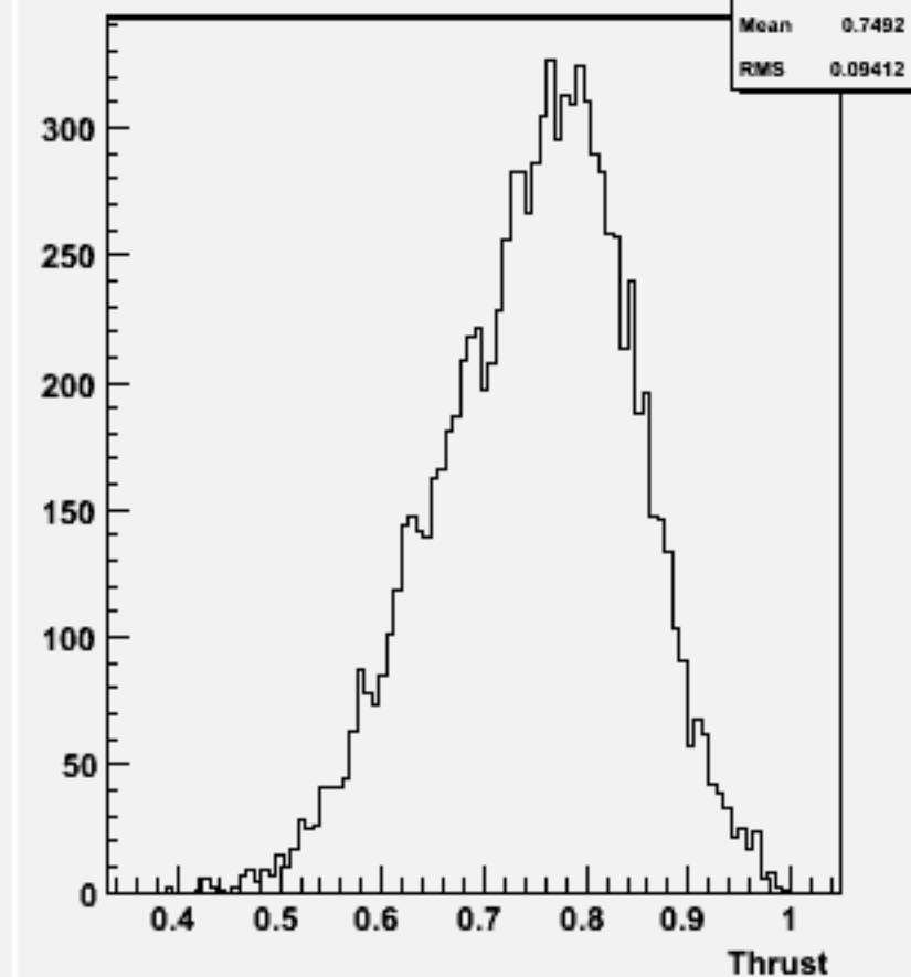
Thrust w100996 ddn1e1e1n1_o
