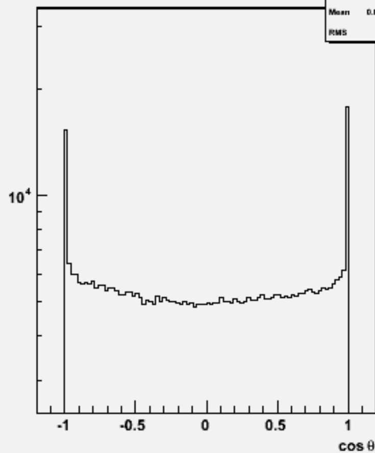
Particle cosθ : w100996 ddn1e1e1n1_o
