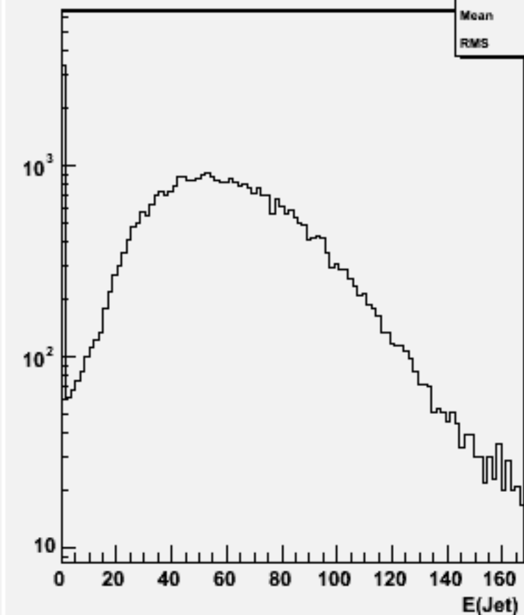
Jet energies(All jets)w100996 ddn1e1e1n1_o
