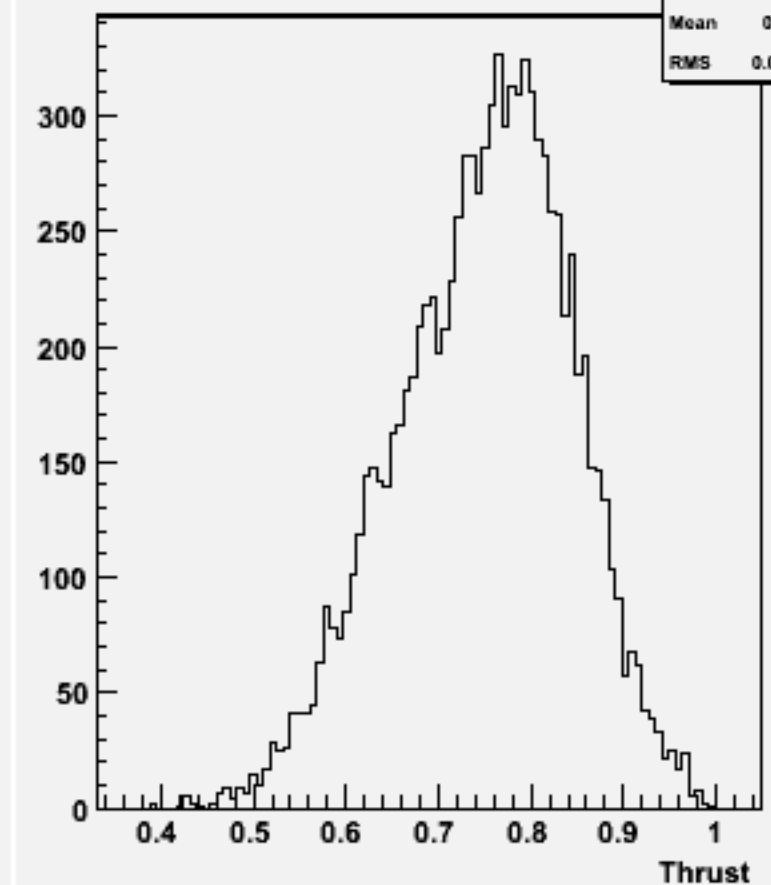
Thrust w100996 ddn1e1e1n1_o
