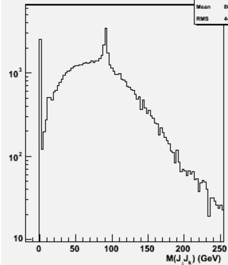
2jets mass(All comb)w100996 ddn1e1e1n1_o
