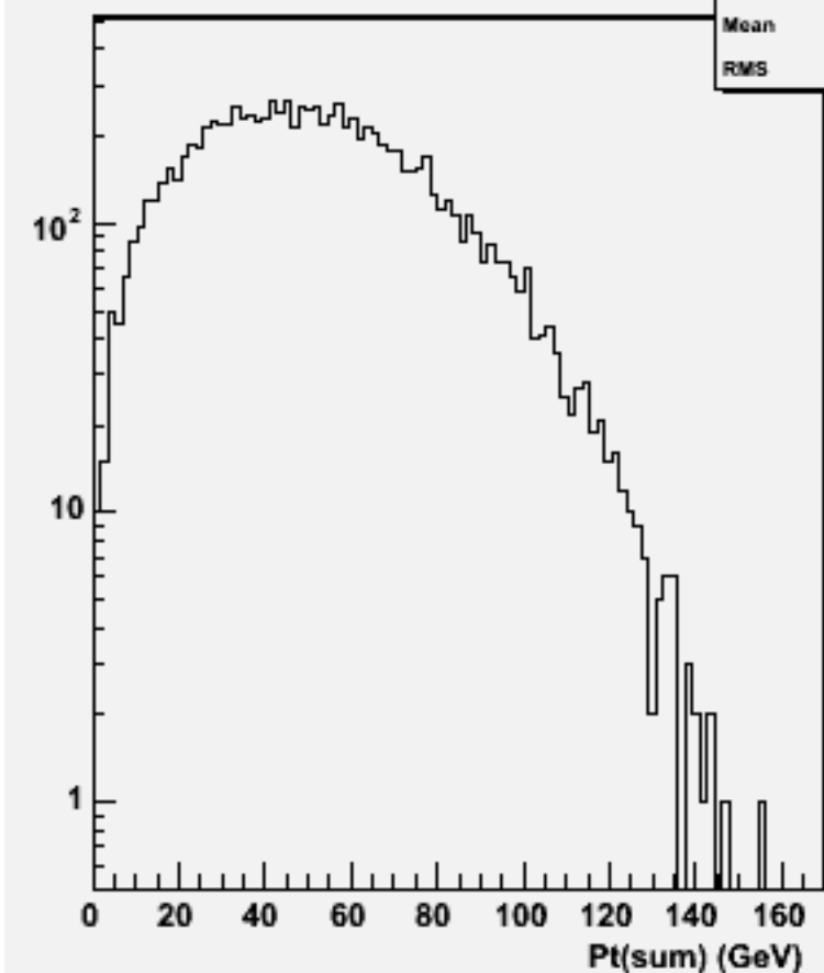
Pt Sum: w100996 ddn1e1e1n1_o
