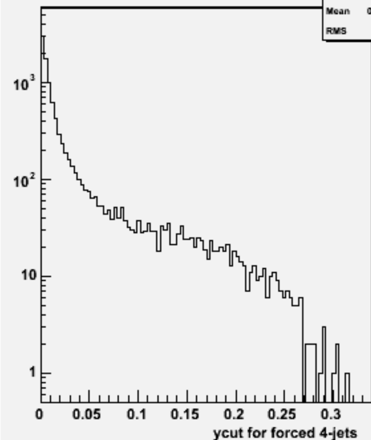
Ycut for 4-jets :w100996 ddn1e1e1n1_o
