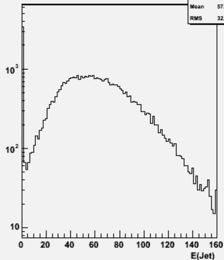
Jet energies(All jets)w100995 ddn1e1e1n1_o
