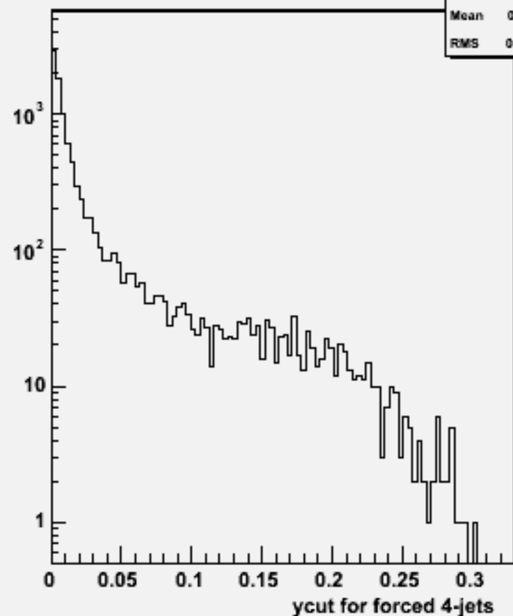
Ycut for 4-jets :w100995 ddn1e1e1n1_o
