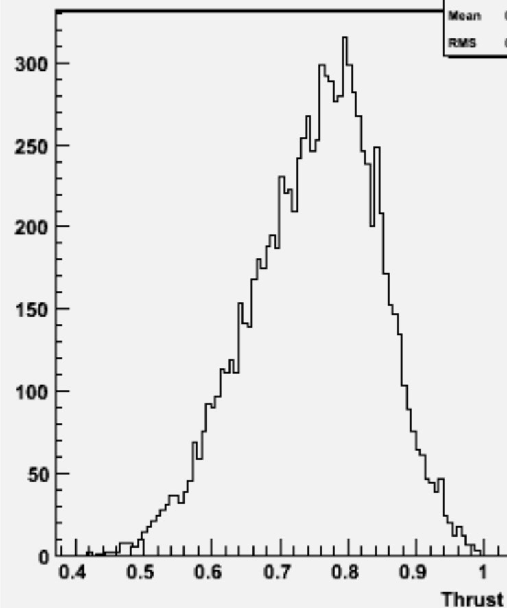
Thrust w100995 ddn1e1e1n1_o
