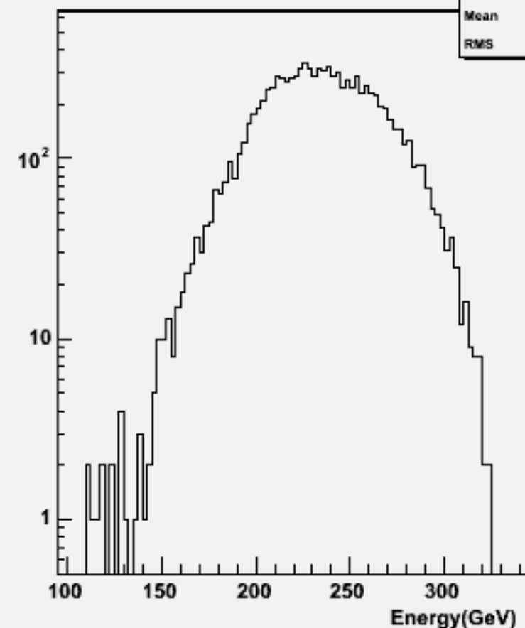
Thrust w100995 ddn1e1e1n1_o
