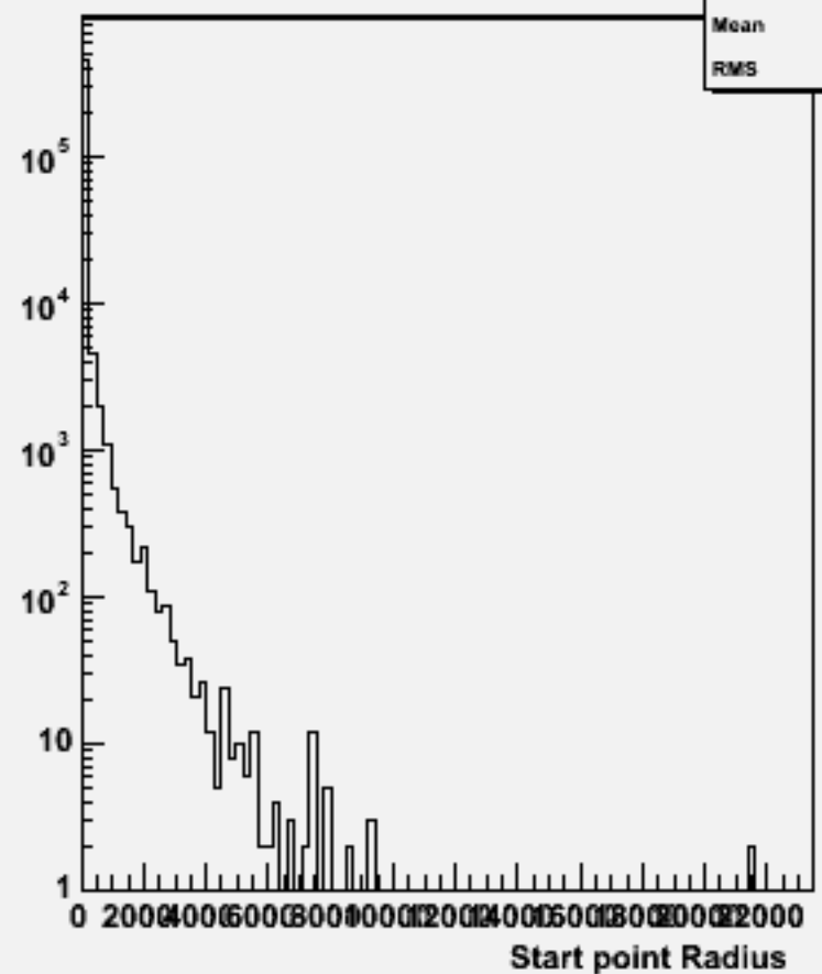
Start point R : w100995 ddn1e1e1n1_o
