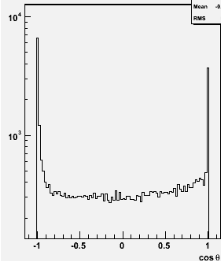
Jet cos \theta (All jets)w100995 ddn1e1e1n1_o
