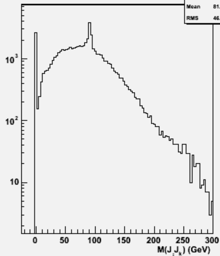
2jets mass(All comb)w100995 ddn1e1e1n1_o
