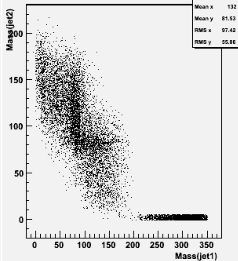
Jet mass for forced 2-jets : w100992 e3e3cssc_o
