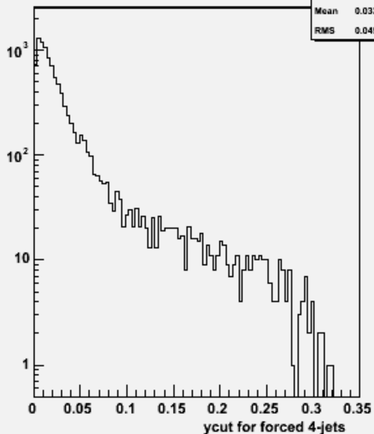
Ycut for 4-jets :w100989 e3e3csdu_o
