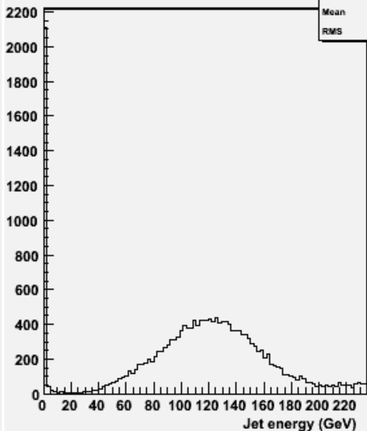
energy for 2-jets :w100978 e3e3cse1n1_o
