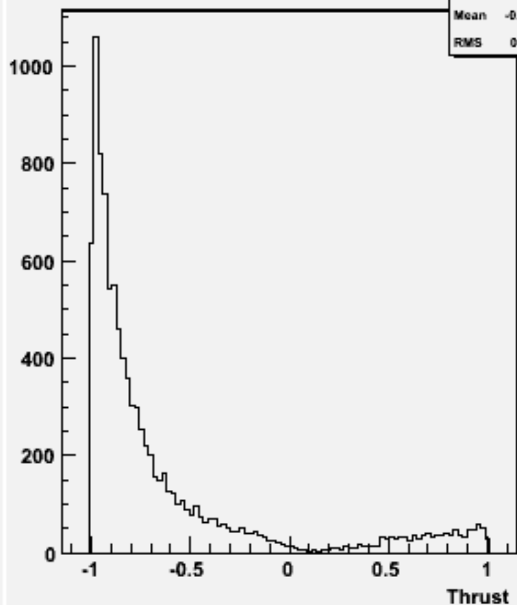
cos \Theta (thrust) w100978 e3e3cse1n1_o
