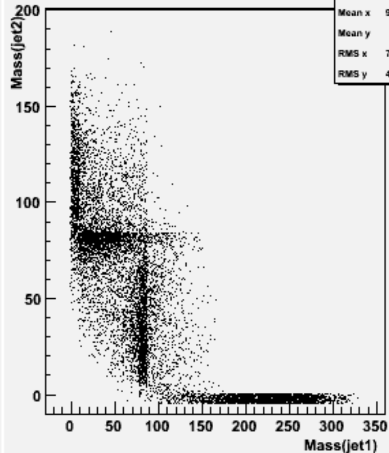
Jet mass for forced 2-jets : w100978 e3e3cse1n1_o
