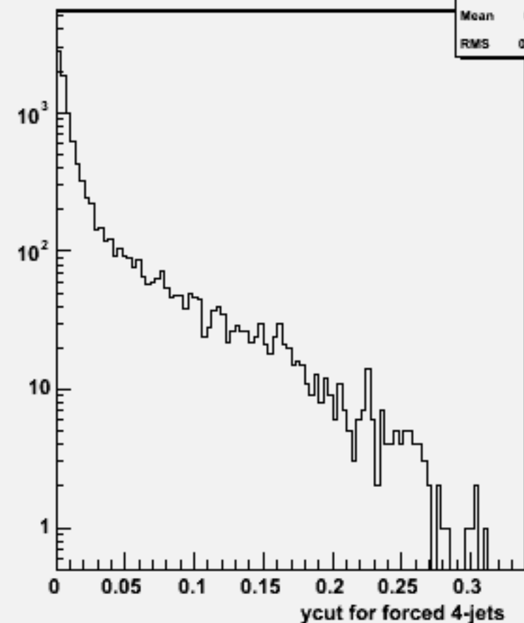
Ycut for 4-jets :w100978 e3e3cse1n1_o
