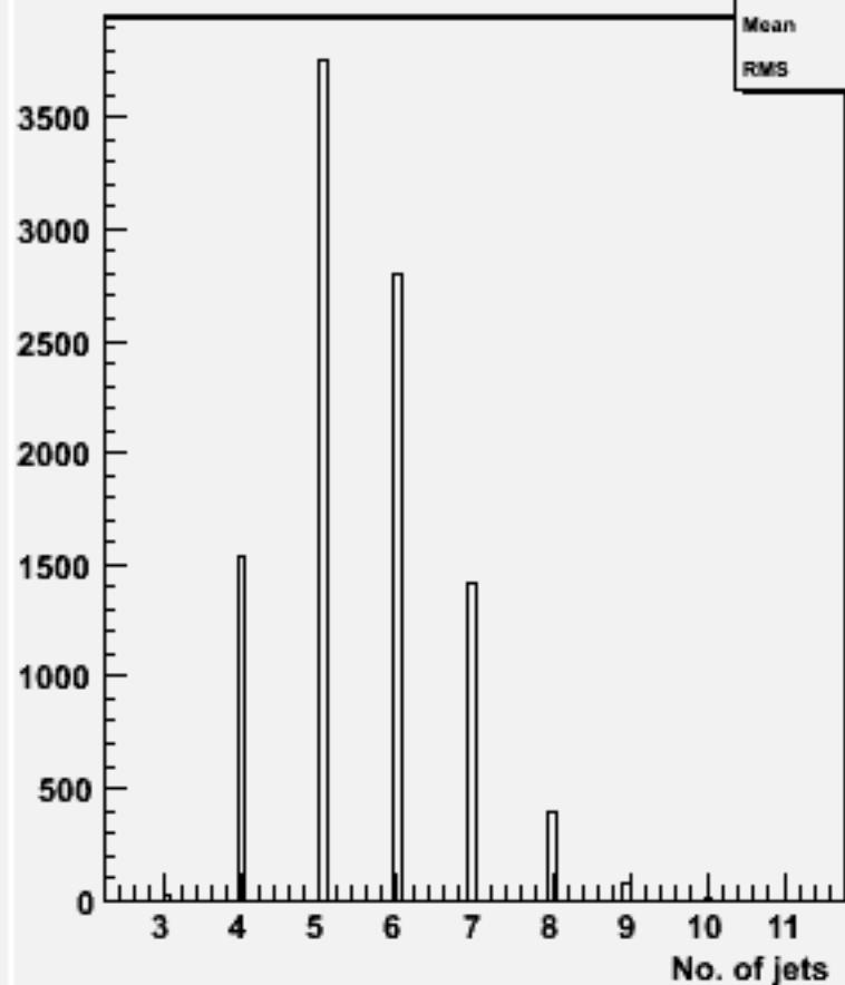
No. jets (ycut=0.001) : w100978 e3e3cse1n1_o
