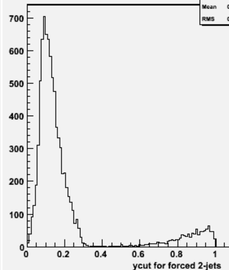
Ycut for 2-jets :w100978 e3e3cse1n1_o
