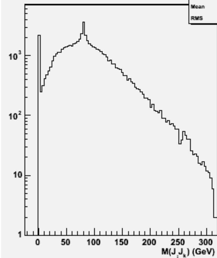
2jets mass(All comb)w100977 e3e3cse1n1_o
