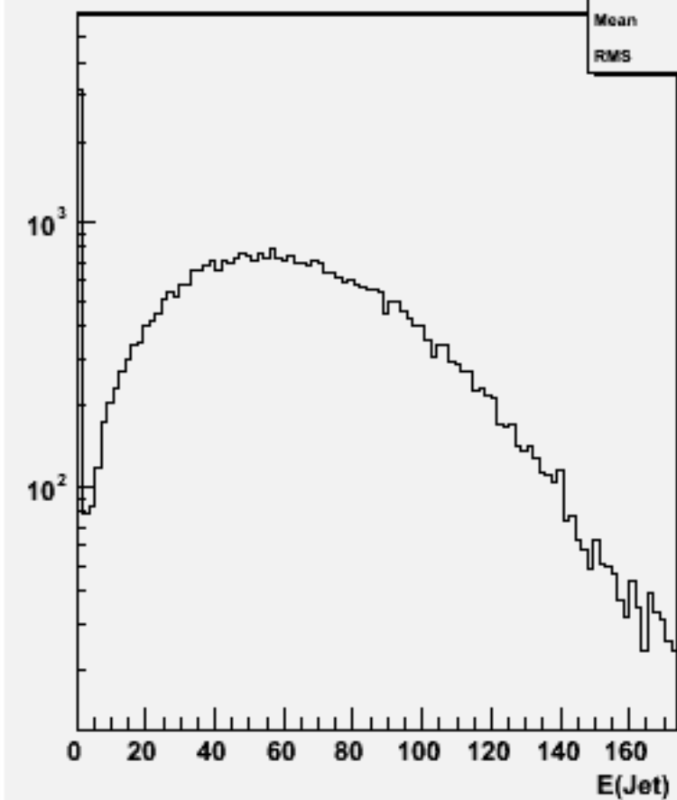
Jet energies(All jets)w100977 e3e3cse1n1_o
