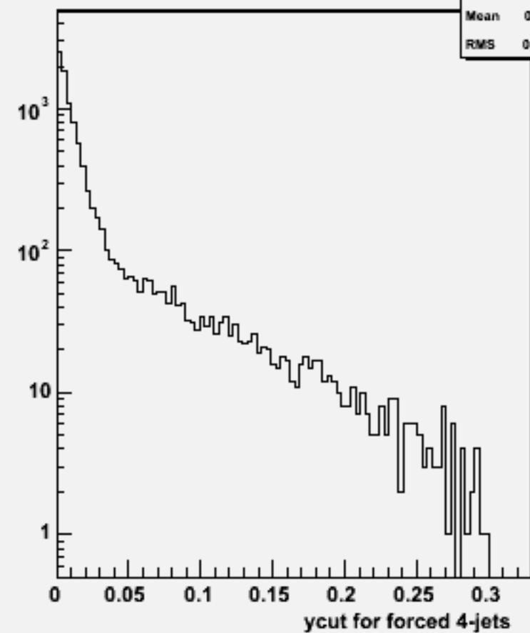
Ycut for 4-jets :w100977 e3e3cse1n1_o
