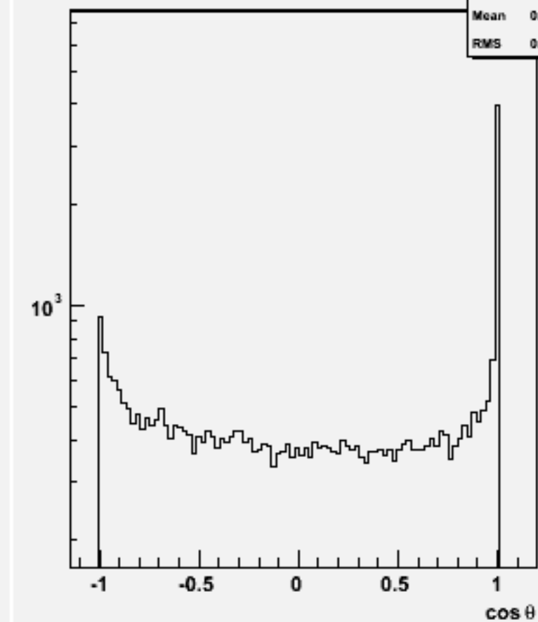
Jet cos \theta (All jets)w100977 e3e3cse1n1_o
