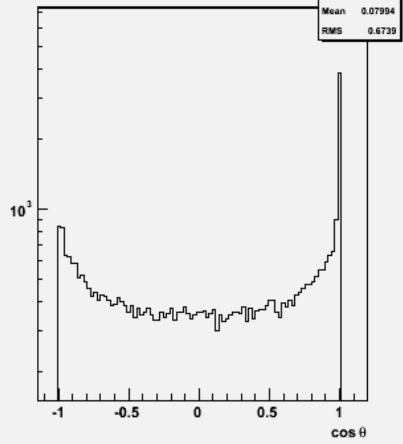
Jet cosθ (All jets)w100969 e3e3uddu_o
