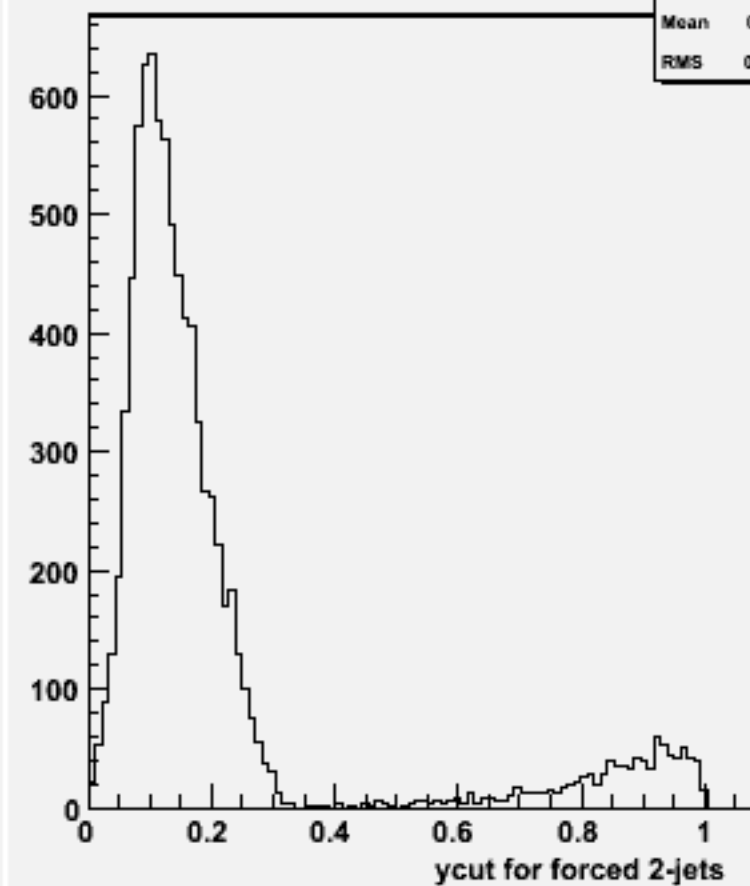
Ycut for 2-jets :w100957 e3e3ude1n1_o
