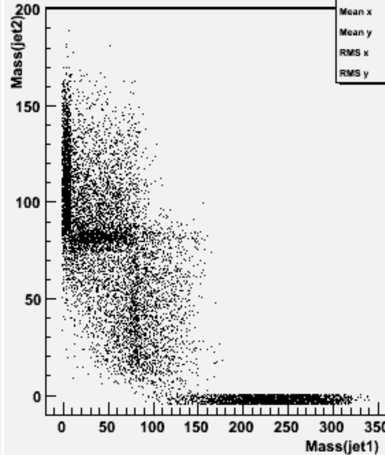
Jet mass for forced 2-jets : w100957 e3e3ude1n1_o
