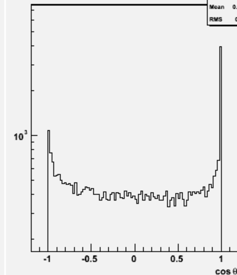
Jet cos \theta (All jets)w100957 e3e3ude1n1_o
