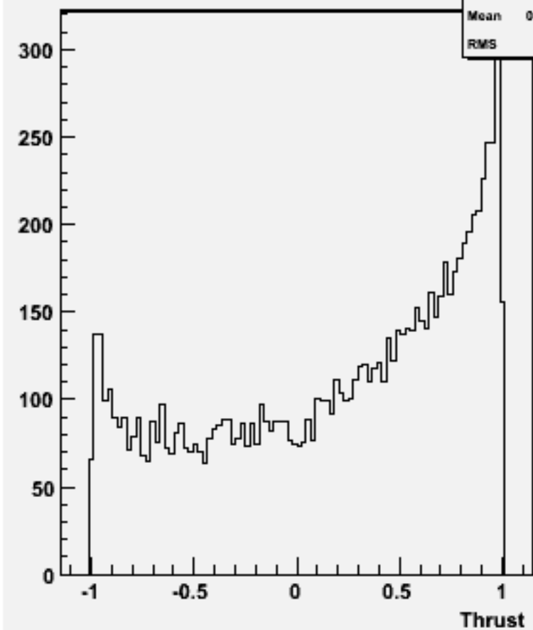
cos \Theta (thrust) w100957 e3e3ude1n1_o
