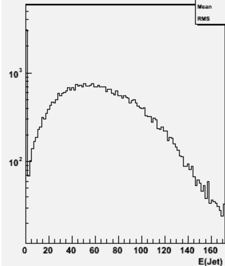
Jet energies(All jets)w100957 e3e3ude1n1_o
