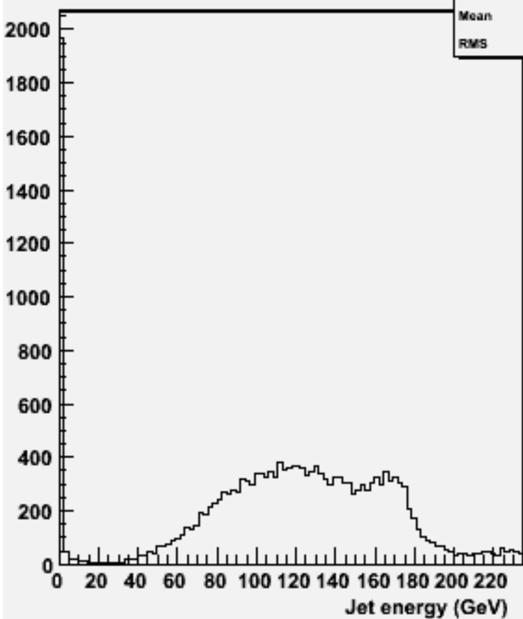
energy for 2-jets :w100957 e3e3ude1n1_o
