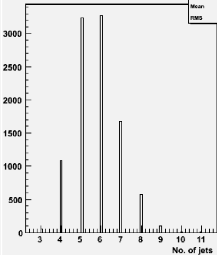
No. jets (ycut=0.001) : w100957 e3e3ude1n1_o
