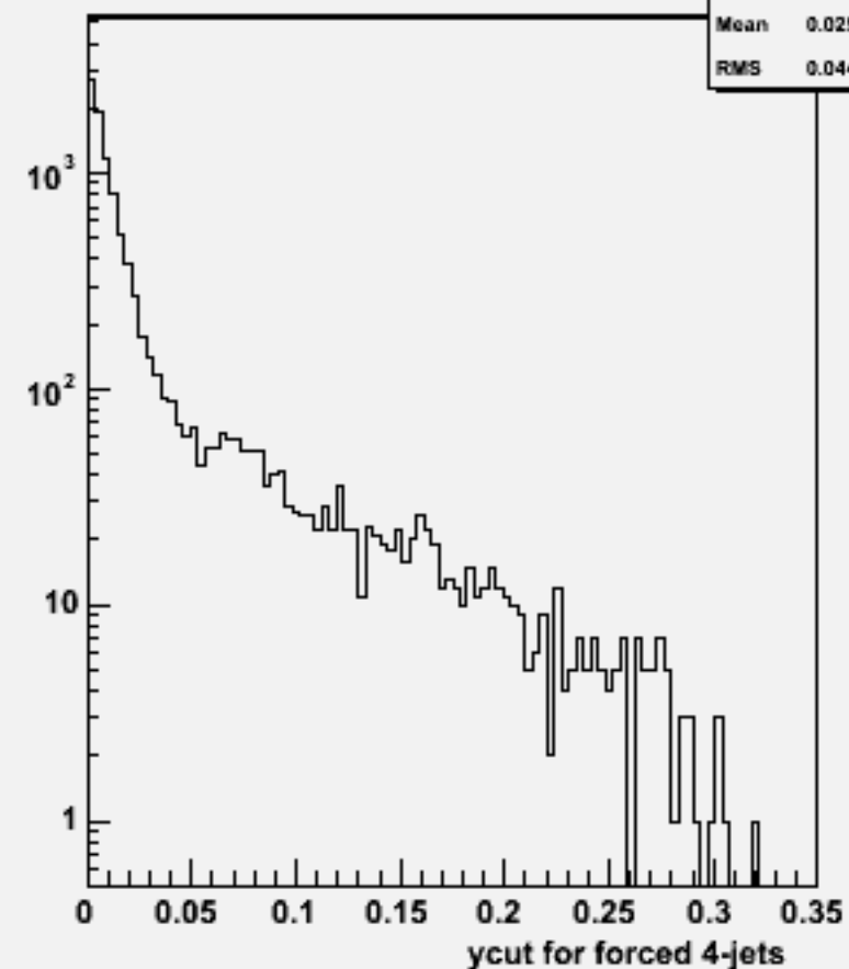
Ycut for 4-jets :w100957 e3e3ude1n1_o
