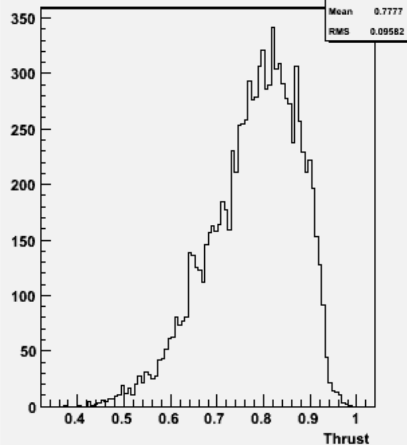
Thrust w100957 e3e3ude1n1_o
