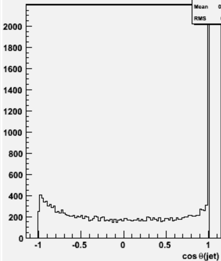
cos \theta for 2-jets :w100957 e3e3ude1n1_o
