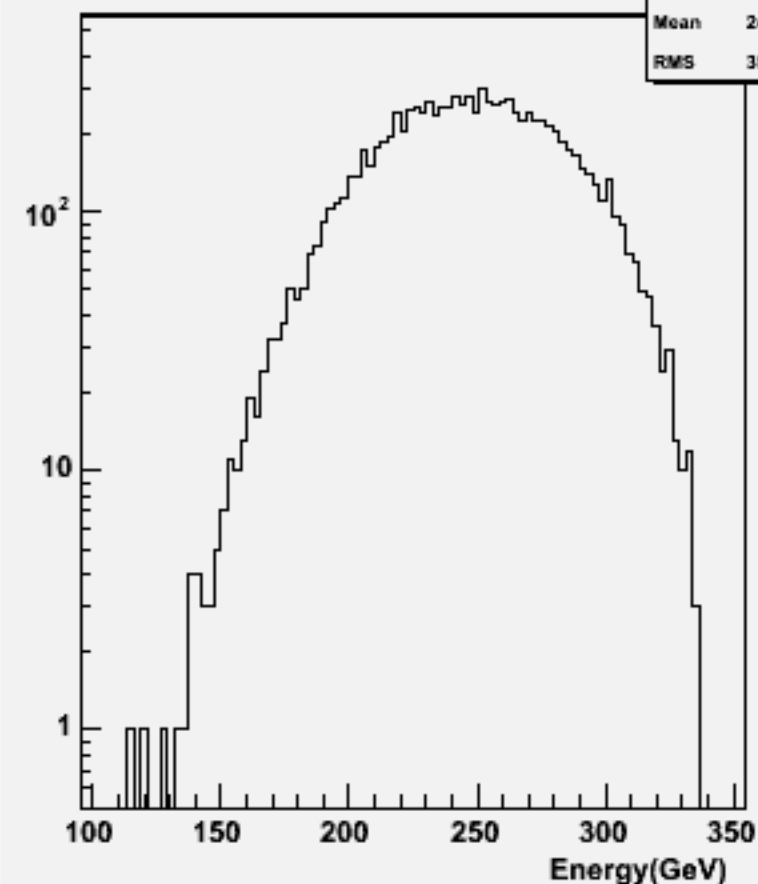
Thrust w100957 e3e3ude1n1_o
