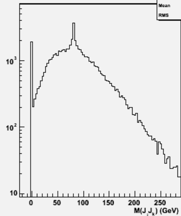
2jets mass(All comb)w100957 e3e3ude1n1_o
