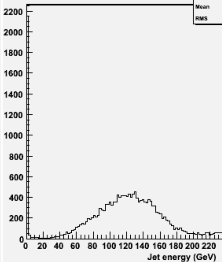
energy for 2-jets :w100956 e3e3ude1n1_o
