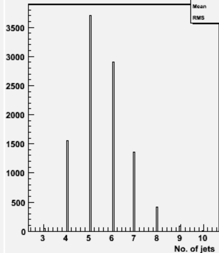
No. jets (ycut=0.001) : w100956 e3e3ude1n1_o
