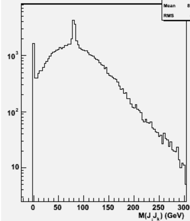
2jets mass(All comb)w100956 e3e3ude1n1_o
