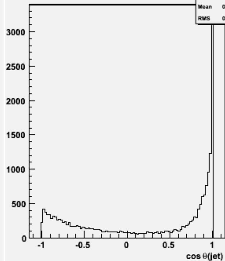
cos \theta for 2-jets :w100956 e3e3ude1n1_o
