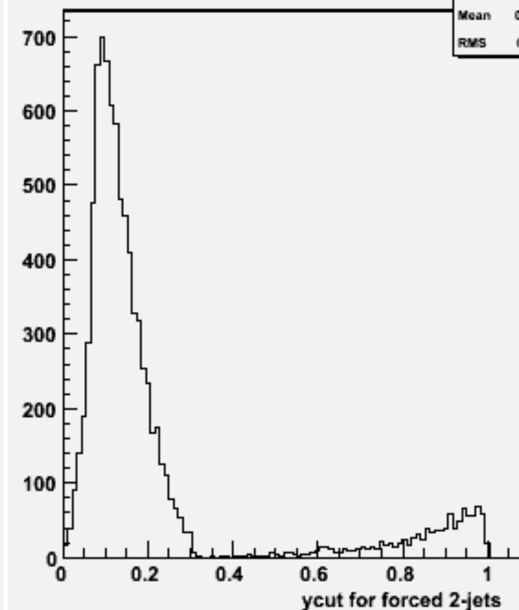
Ycut for 2-jets :w100956 e3e3ude1n1_o
