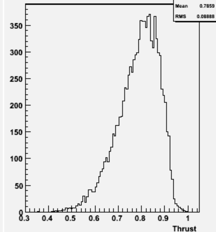
Thrust w100956 e3e3ude1n1_o
