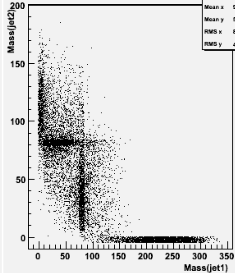
Jet mass for forced 2-jets : w100956 e3e3ude1n1_o
