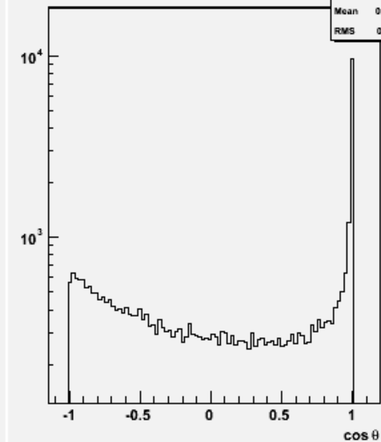
Jet cos \theta (All jets)w100956 e3e3ude1n1_o
