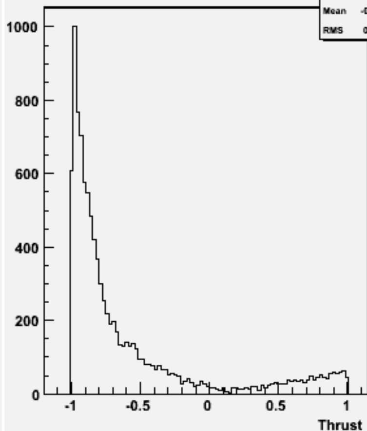
cos \Theta (thrust) w100956 e3e3ude1n1_o
