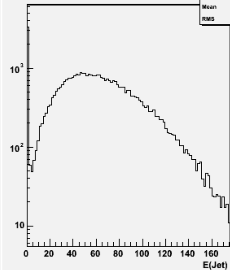
Jet energies(All jets)w100956 e3e3ude1n1_o
