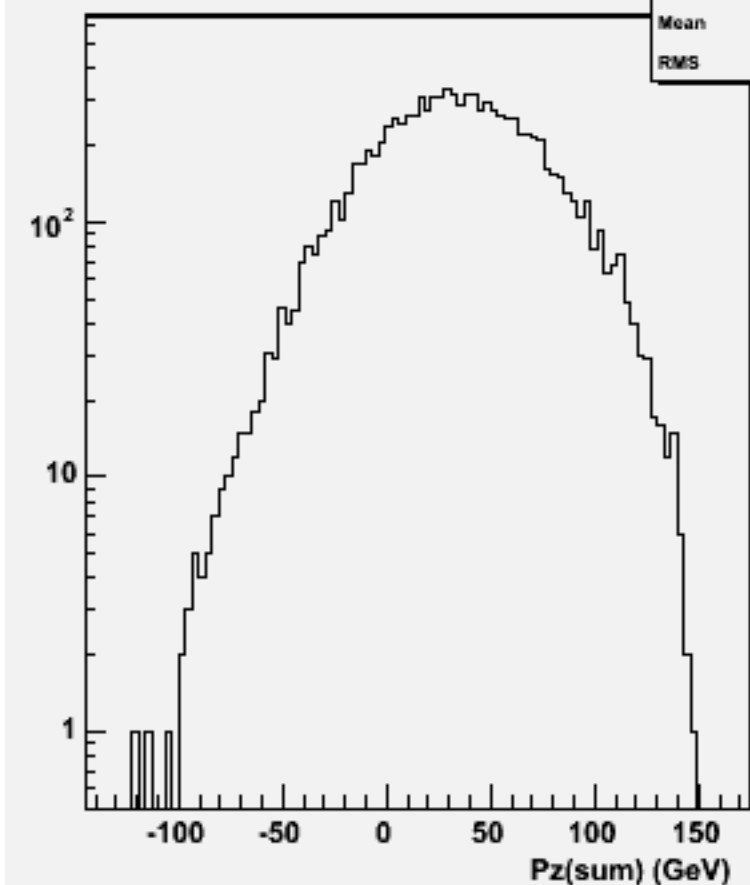
Pz Sum: w100956 e3e3ude1n1_o
