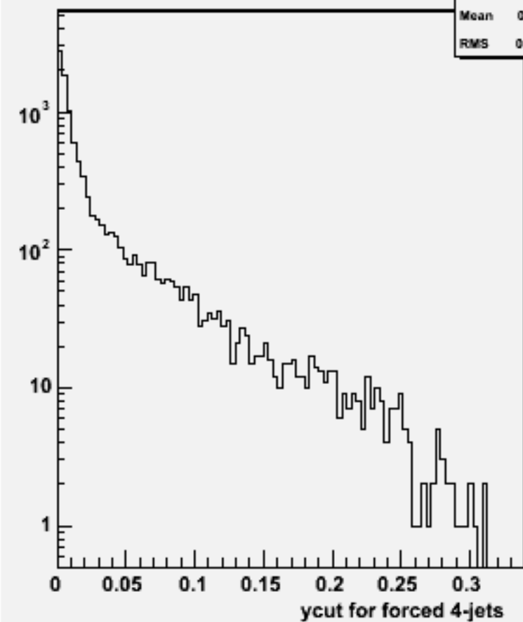
Ycut for 4-jets :w100956 e3e3ude1n1_o
