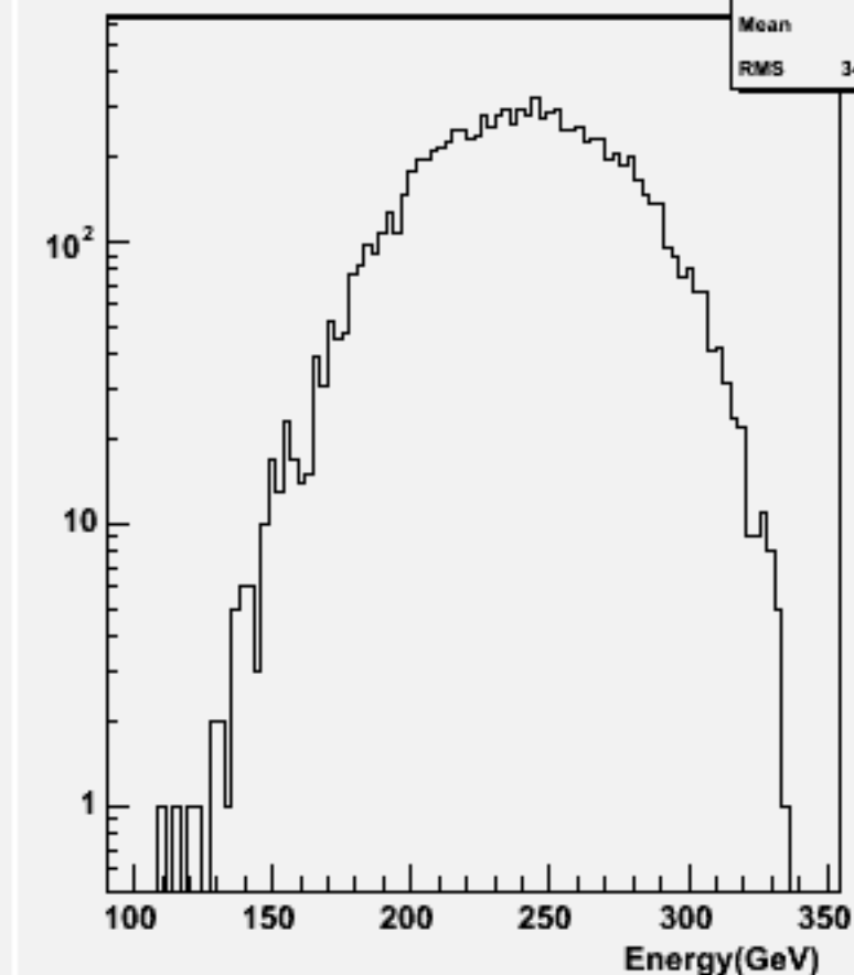
Thrust w100956 e3e3ude1n1_o
