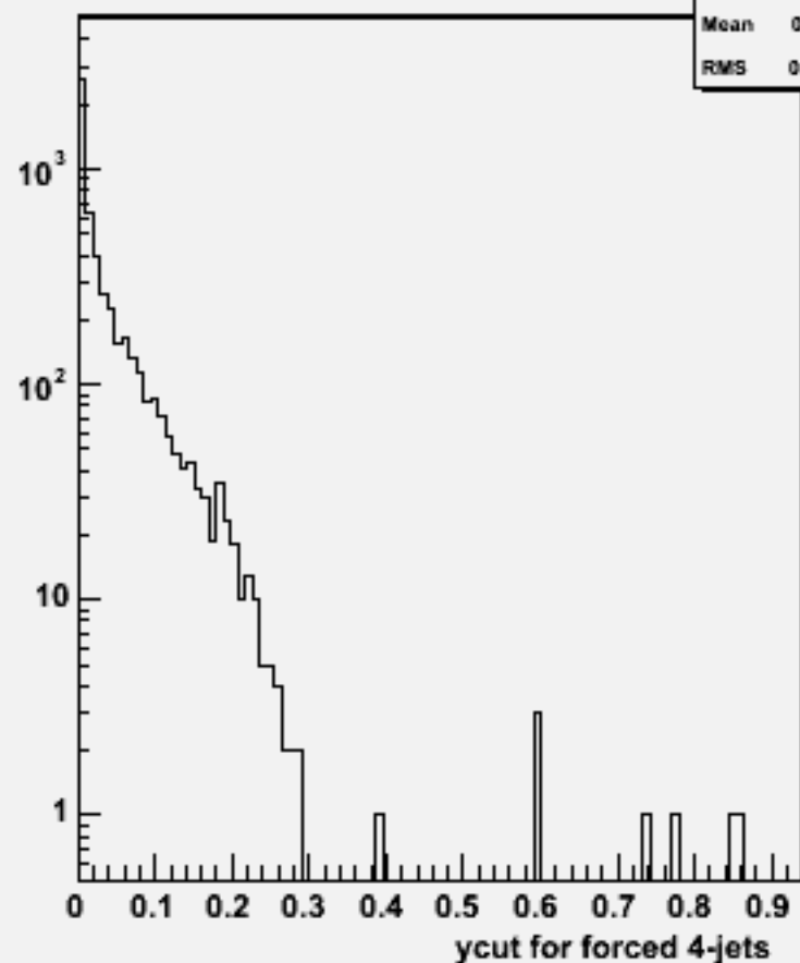
Ycut for 4-jets :w100938 e3e3n3e3e1n1_o
