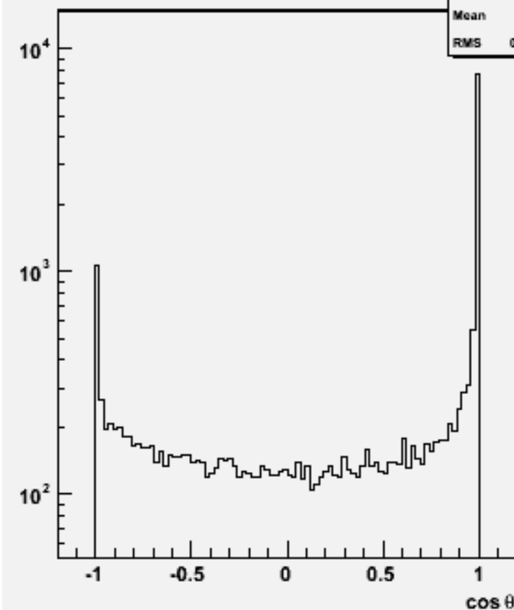
Jet cos \theta (All jets)w100938 e3e3n3e3e1n1_o
