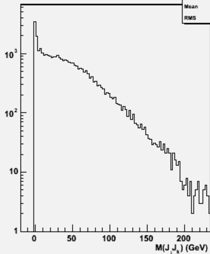
2jets mass(All comb)w100938 e3e3n3e3e1n1_o
