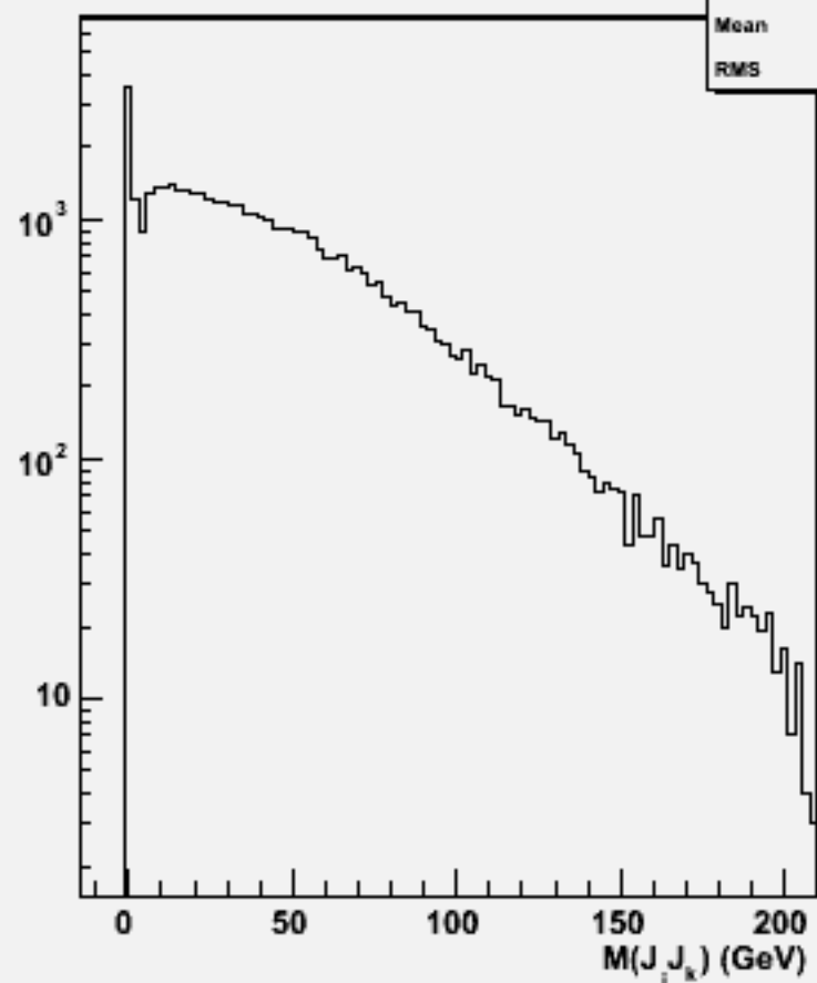
2jets mass(All comb)w100937 e3e3n3e3e1n1_o
