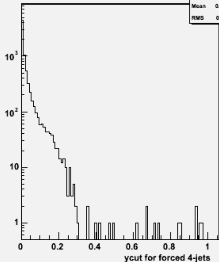
Ycut for 4-jets :w100937 e3e3n3e3e1n1_o
