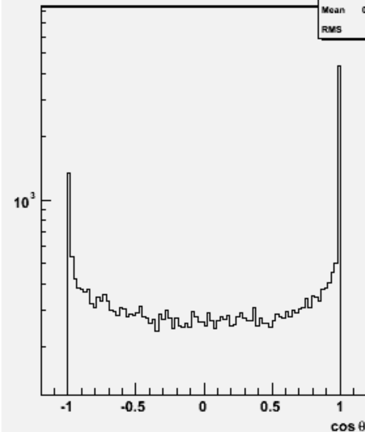
Jet cos \theta (All jets)w100937 e3e3n3e3e1n1_o
