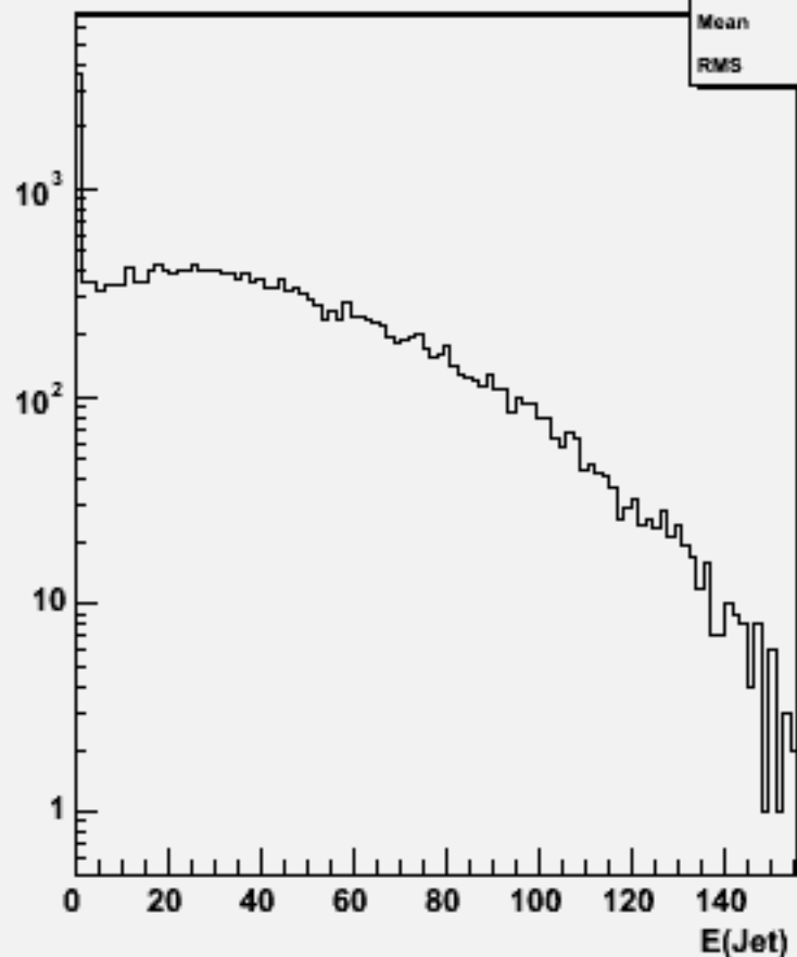
Jet energies(All jets)w100936 e3e3n3e3e1n1_o
