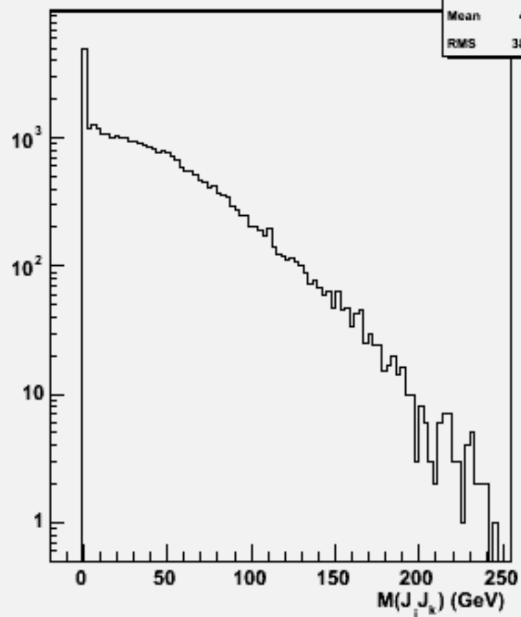
2jets mass(All comb)w100936 e3e3n3e3e1n1_o
