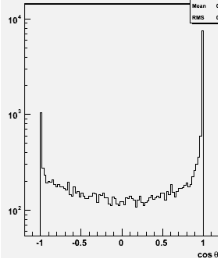
Jet cos \theta (All jets)w100936 e3e3n3e3e1n1_o
