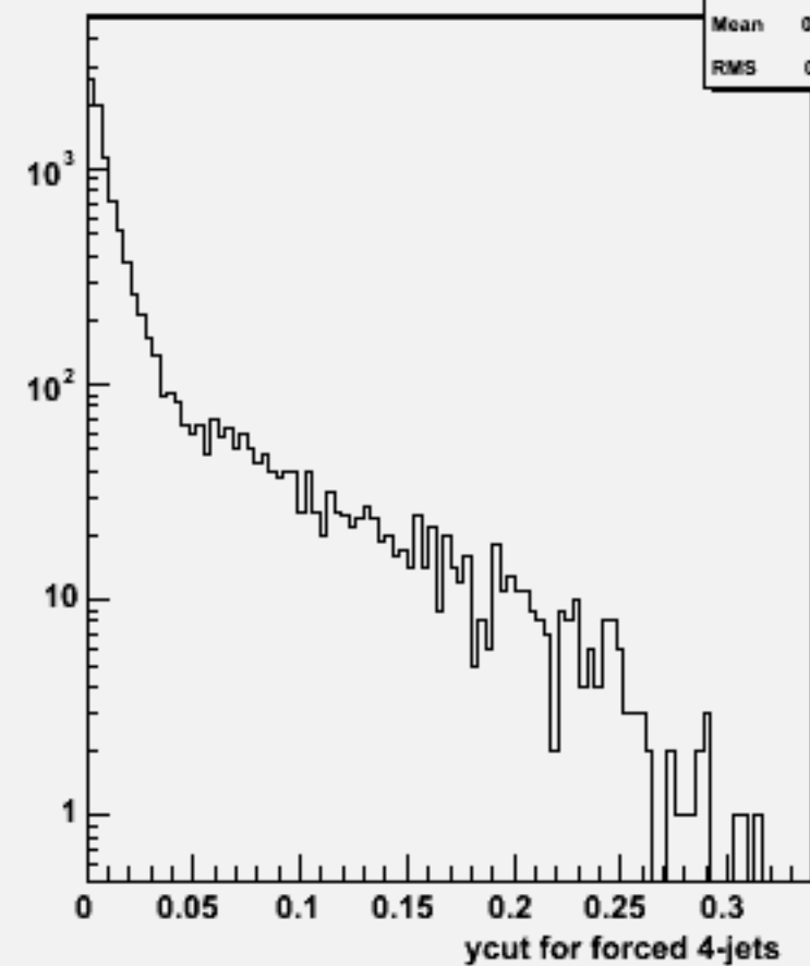
Ycut for 4-jets :w100933 e3e3n2e2sc_o
