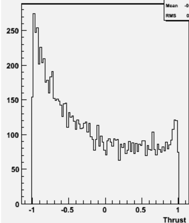
cos \Theta (thrust) w100933 e3e3n2e2sc_o
