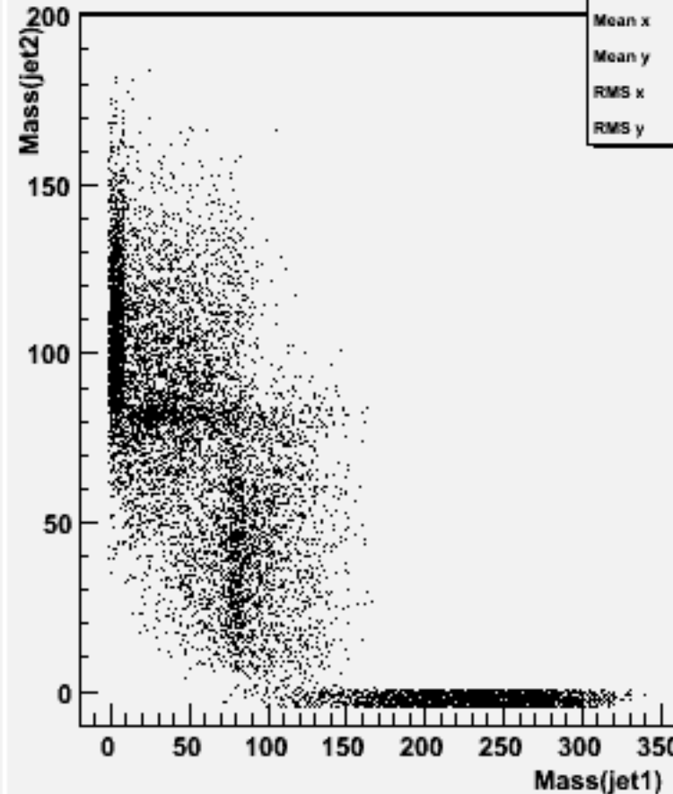
Jet mass for forced 2-jets : w100933 e3e3n2e2sc_o
