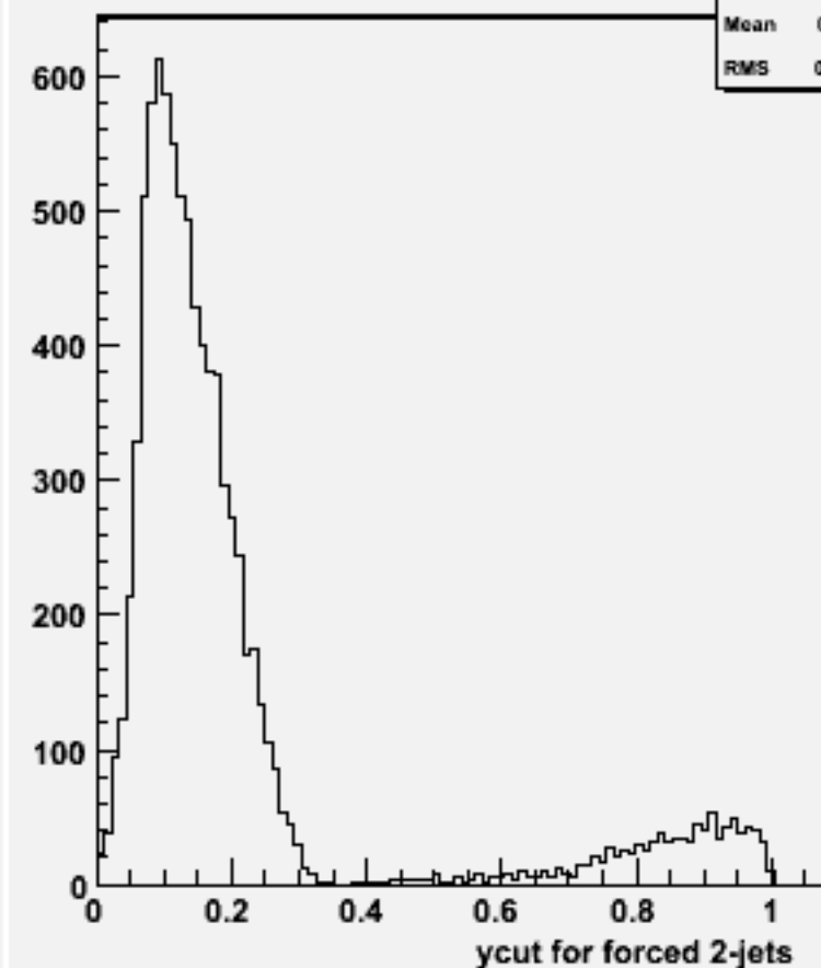
Ycut for 2-jets :w100933 e3e3n2e2sc_o
