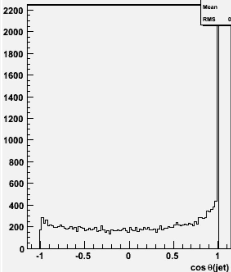
cos \theta for 2-jets :w100933 e3e3n2e2sc_o
