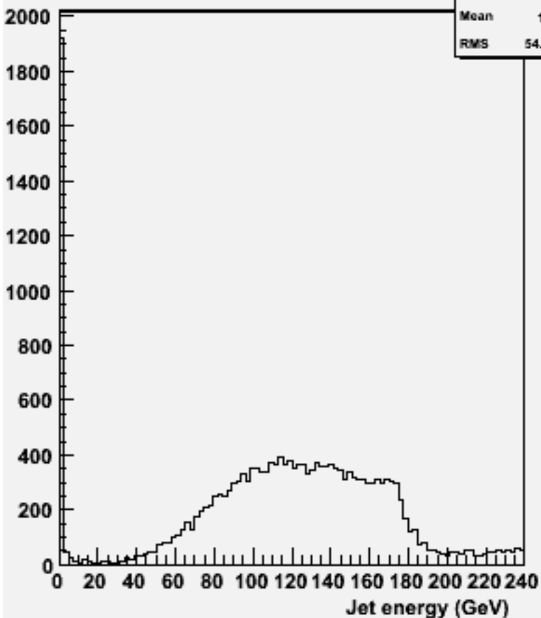
energy for 2-jets :w100933 e3e3n2e2sc_o
