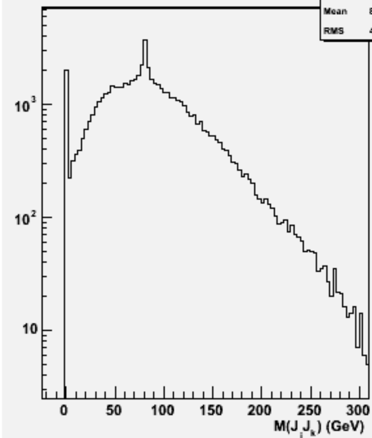
2jets mass(All comb)w100933 e3e3n2e2sc_o
