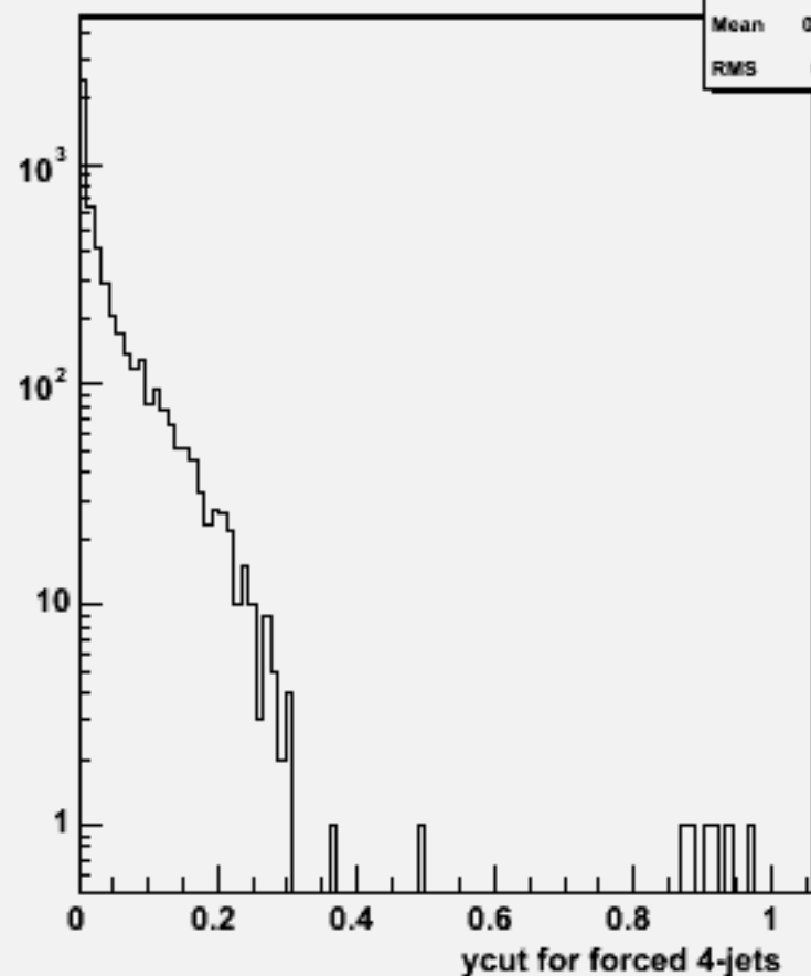
Ycut for 4-jets :w100918 e3e3n2e2e1n1_o
