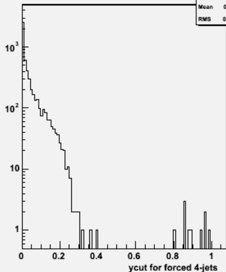
Ycut for 4-jets :w100916 e3e3n2e2e1n1_o
