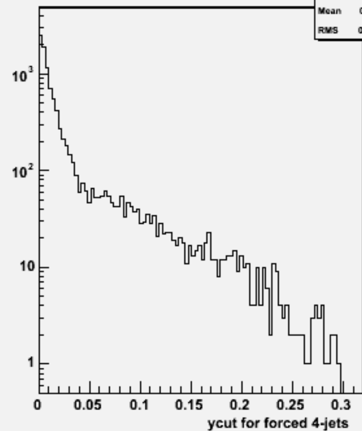
Ycut for 4-jets :w100913 e3e3n1e1sc_o
