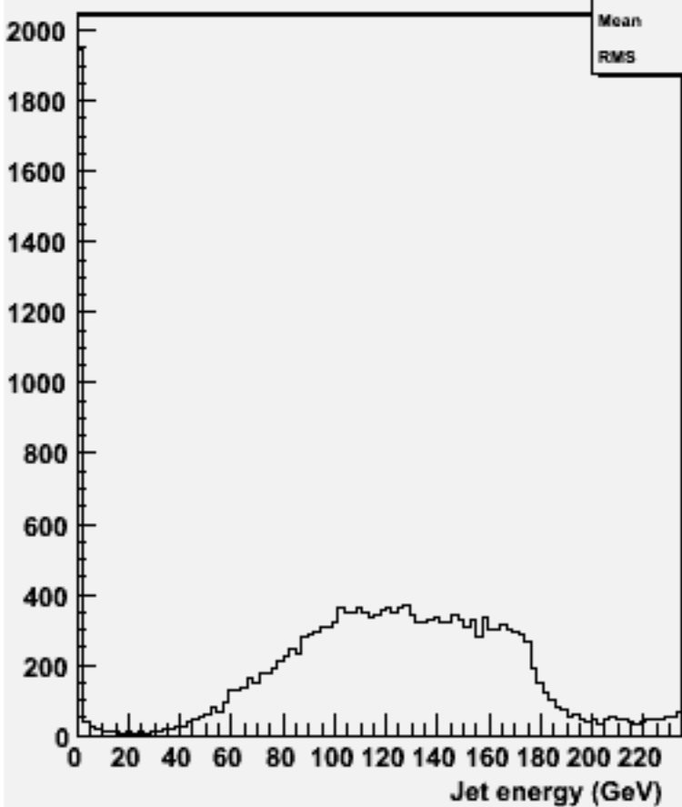
energy for 2-jets :w100913 e3e3n1e1sc_o
