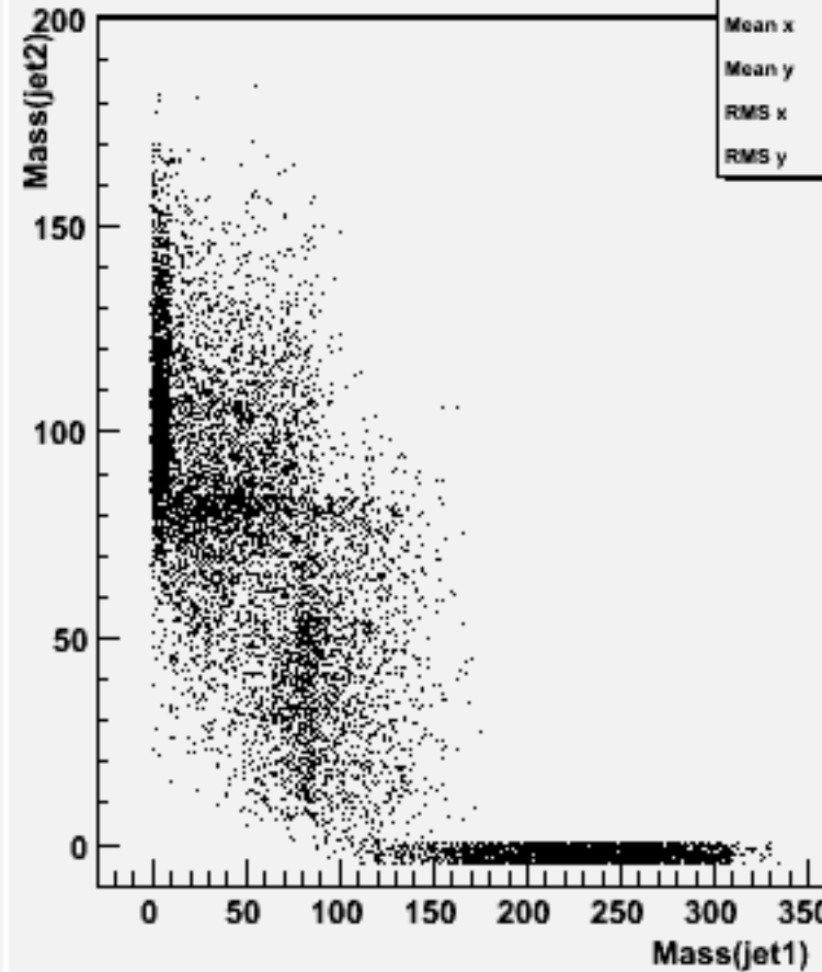
Jet mass for forced 2-jets : w100913 e3e3n1e1sc_o
