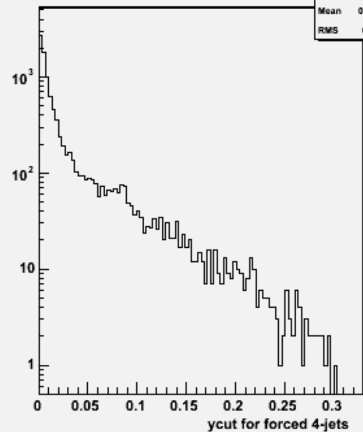
Ycut for 4-jets :w100912 e3e3n1e1sc_o
