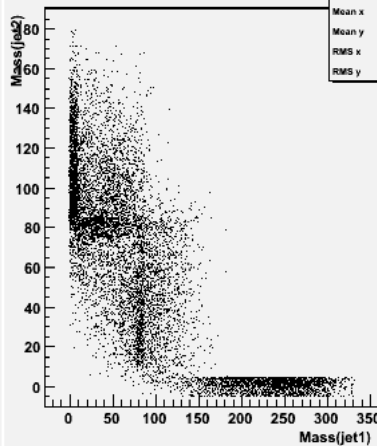
Jet mass for forced 2-jets : w100909 e3e3n1e1du_o
