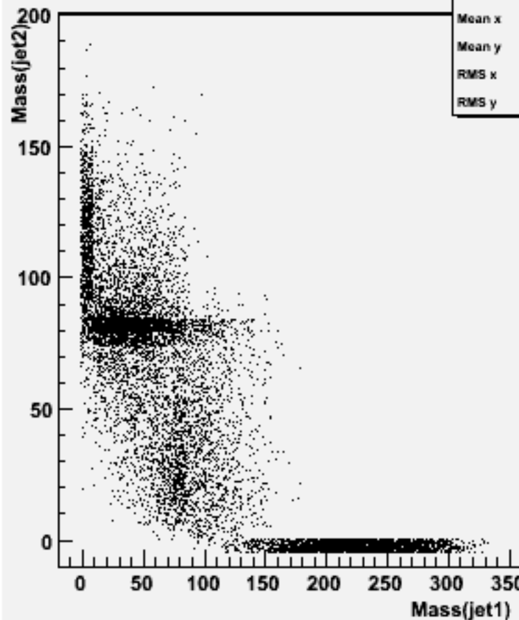
Jet mass for forced 2-jets : w100907 e3e3n1e1du_o
