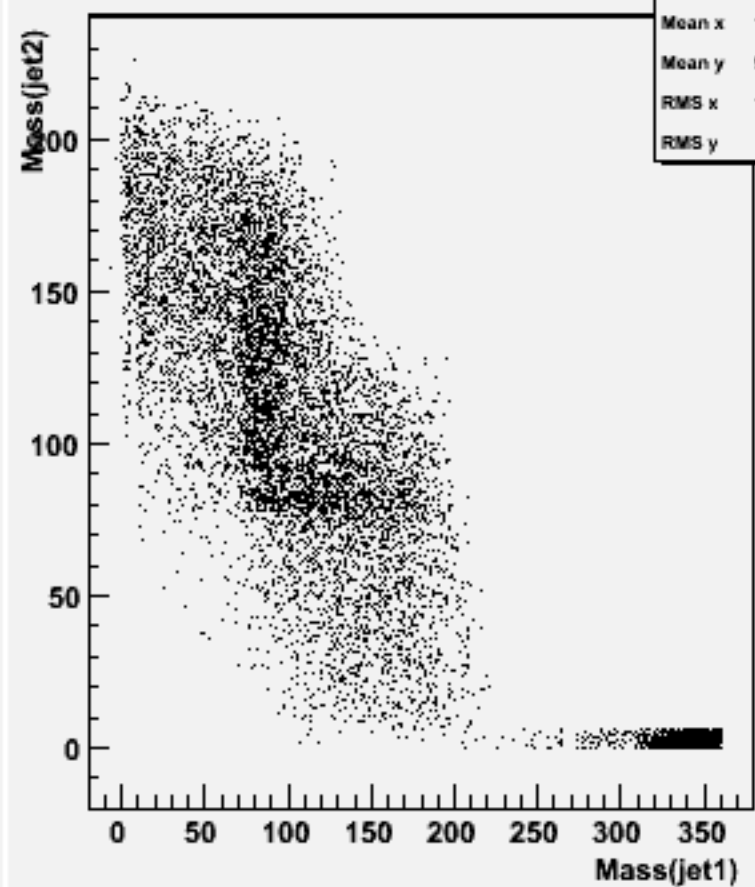
Jet mass for forced 2-jets : w100893 e2e2cssc_o
