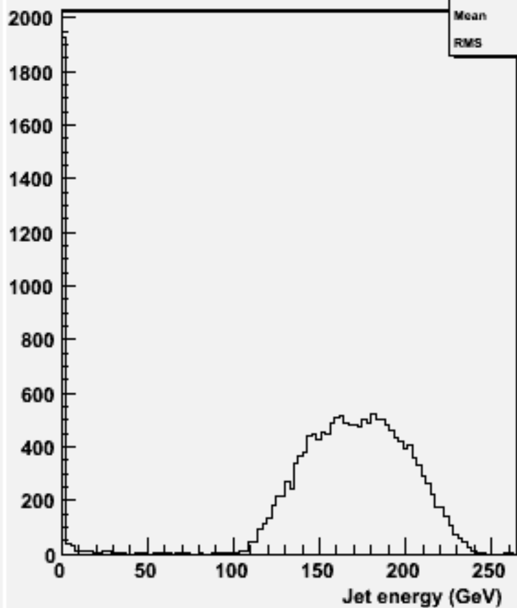
energy for 2-jets :w100893 e2e2cssc_o
