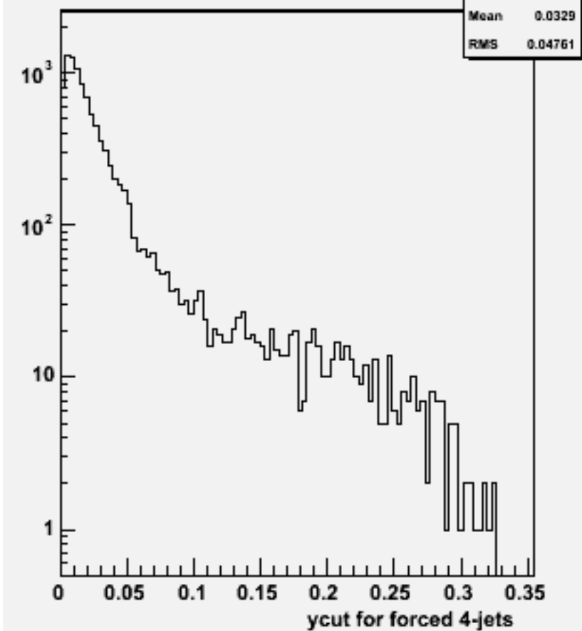
Ycut for 4-jets :w100893 e2e2cssc_o
