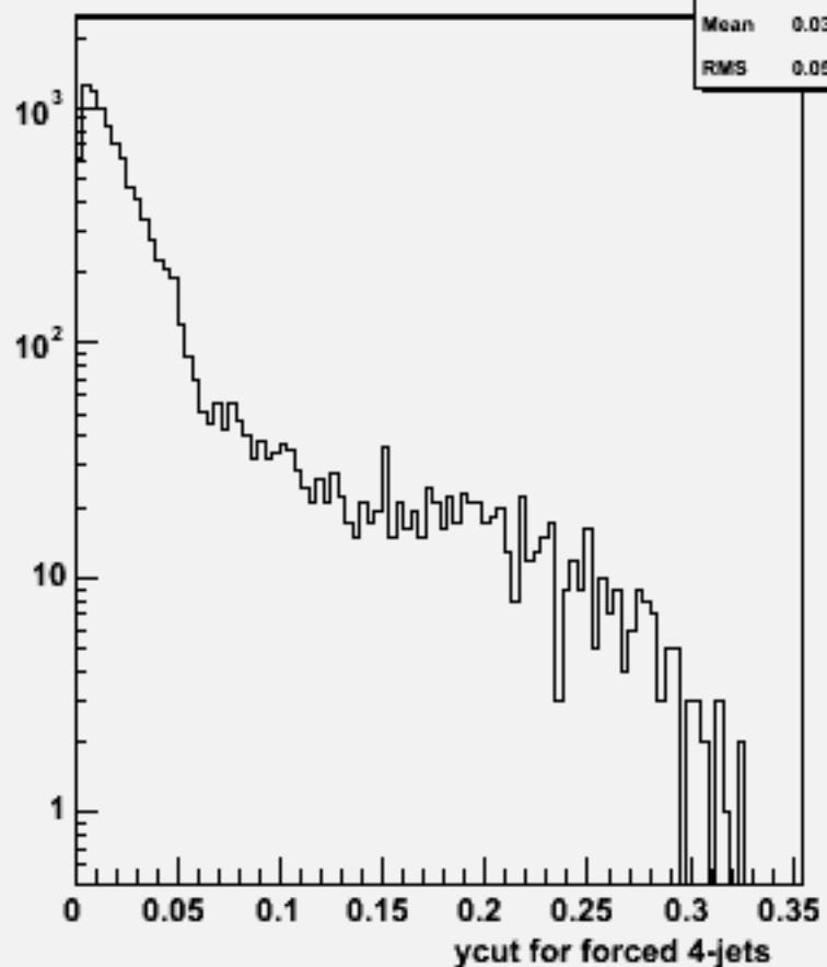
Ycut for 4-jets :w100892 e2e2cssc_o
