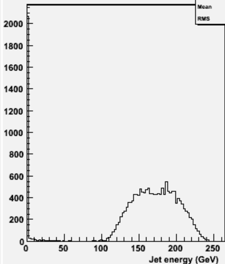
energy for 2-jets :w100892 e2e2cssc_o
