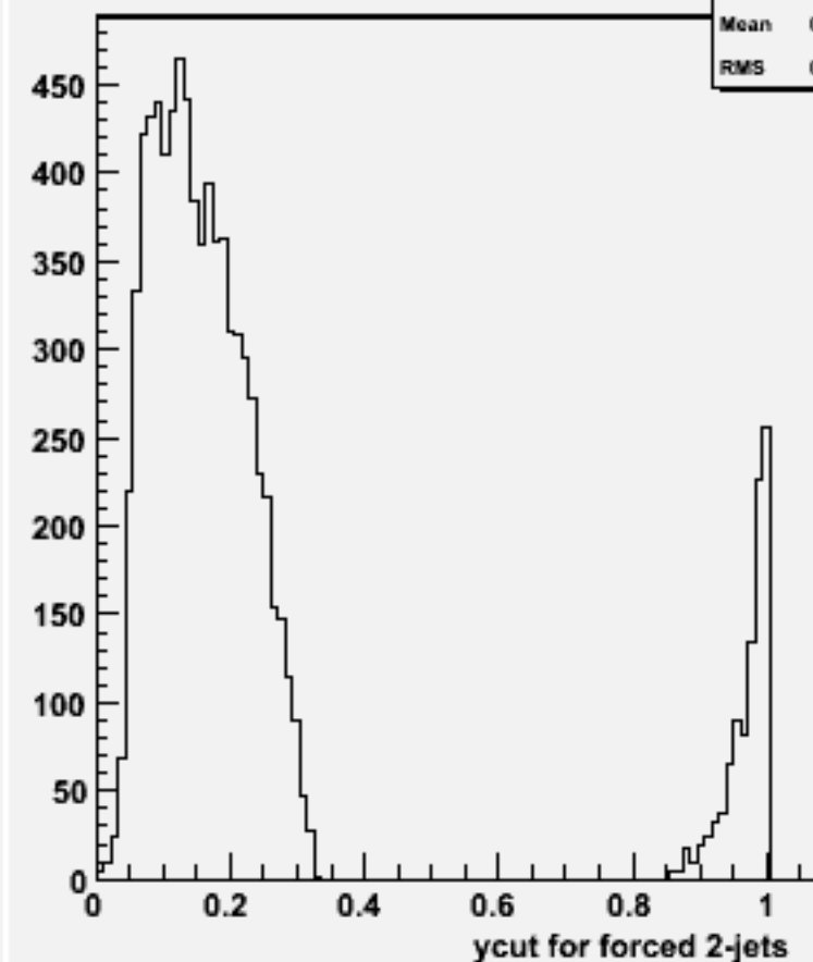
Ycut for 2-jets :w100892 e2e2cssc_o
