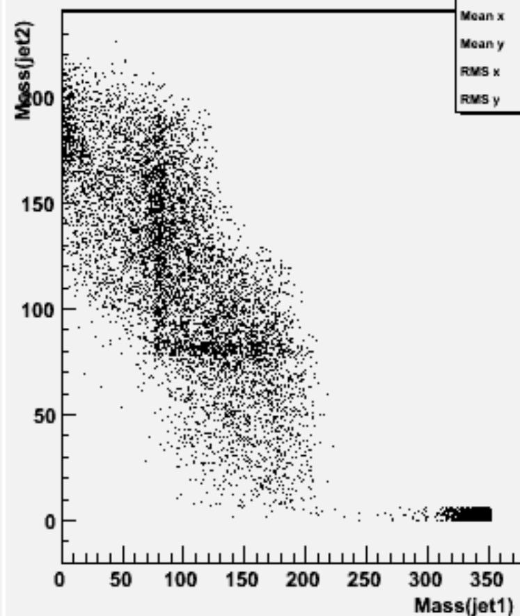
Jet mass for forced 2-jets : w100892 e2e2cssc_o
