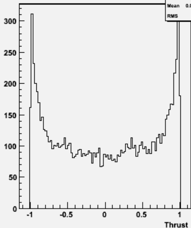
cos \Theta (thrust) w100892 e2e2cssc_o
