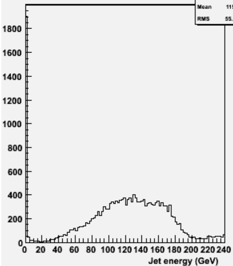
energy for 2-jets :w100885 e2e2cse3n3_o
