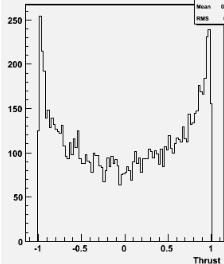
cos \Theta (thrust) w100885 e2e2cse3n3_o
