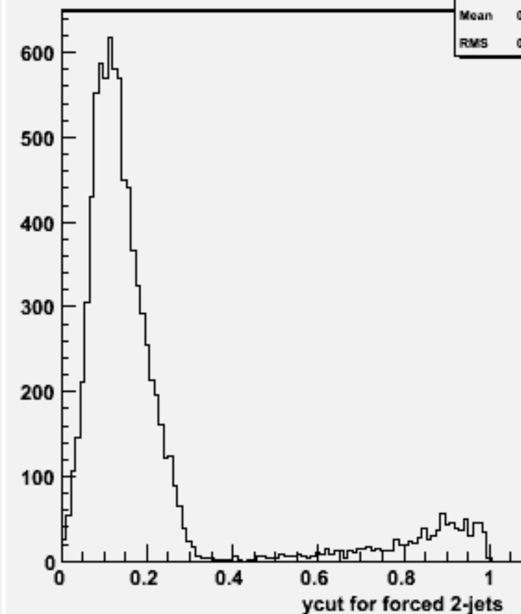
Ycut for 2-jets :w100885 e2e2cse3n3_o
