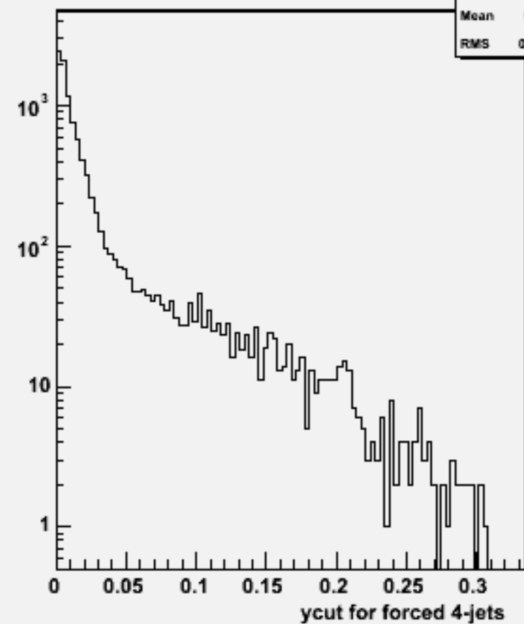
Ycut for 4-jets :w100885 e2e2cse3n3_o
