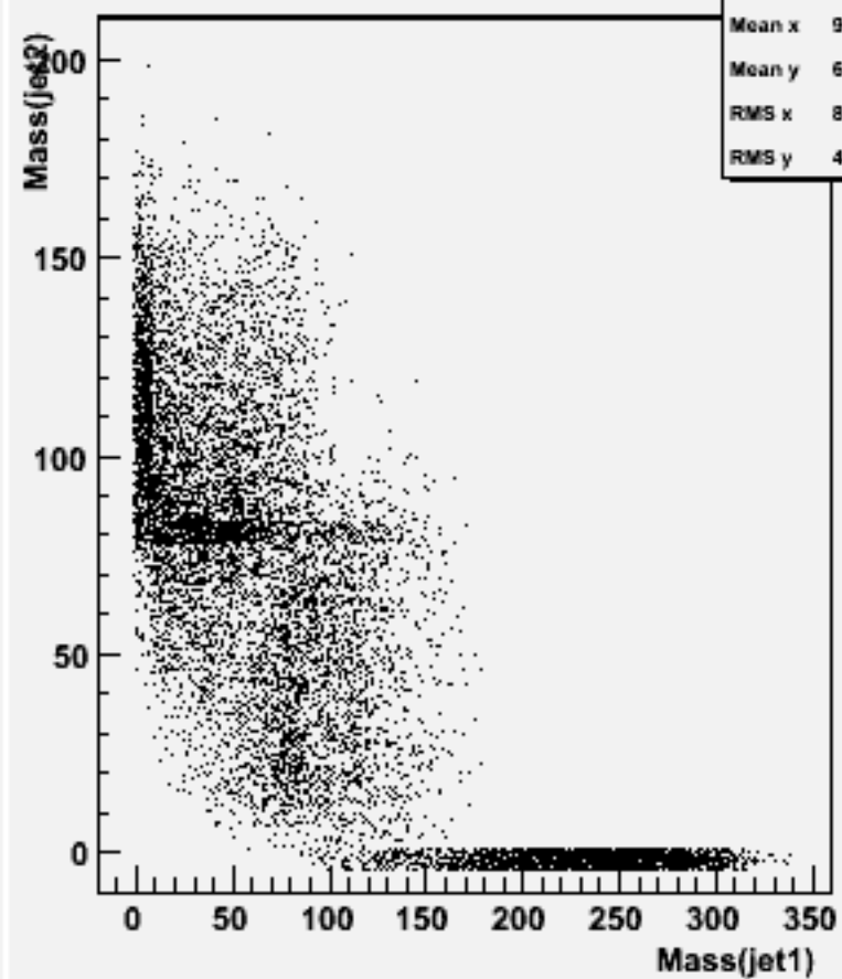
Jet mass for forced 2-jets : w100885 e2e2cse3n3_o
