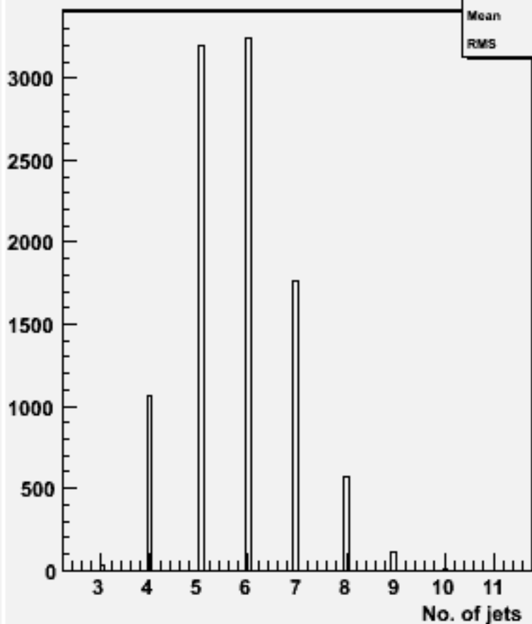
No. jets (ycut=0.001) : w100884 e2e2cse3n3_o
