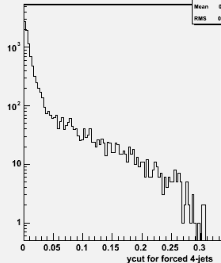
Ycut for 4-jets :w100884 e2e2cse3n3_o
