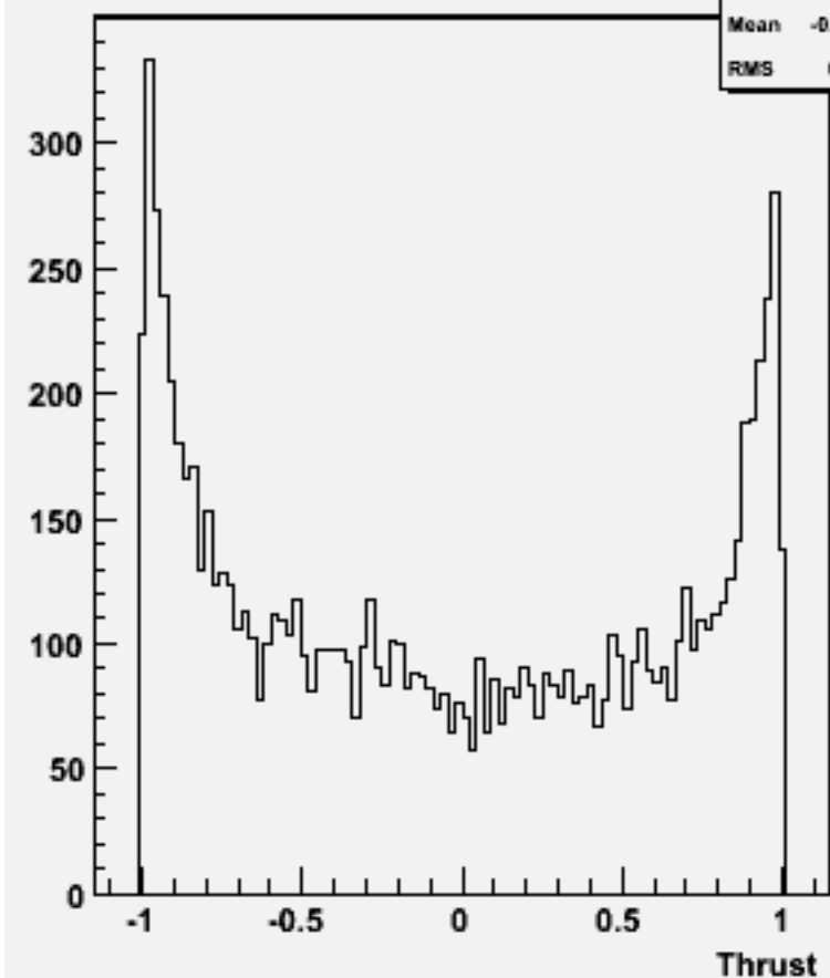
cos \Theta (thrust) w100884 e2e2cse3n3_o
