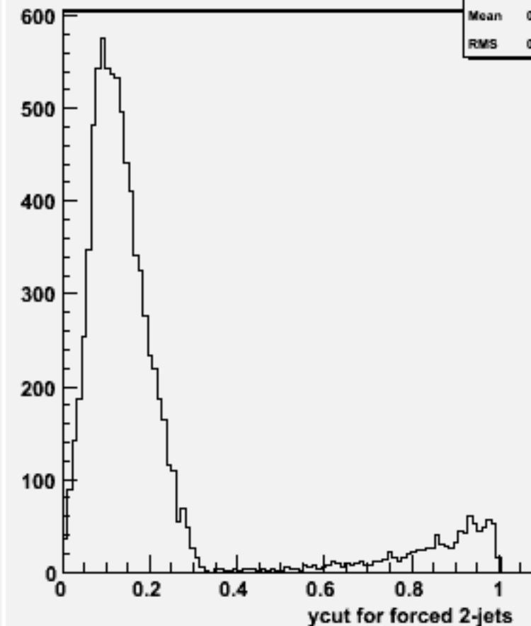
Ycut for 2-jets :w100884 e2e2cse3n3_o
