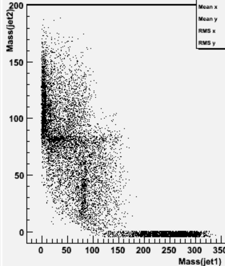
Jet mass for forced 2-jets : w100884 e2e2cse3n3_o
