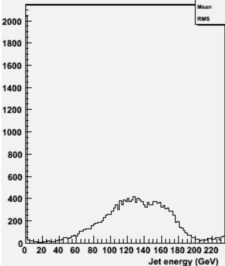
energy for 2-jets :w100884 e2e2cse3n3_o
