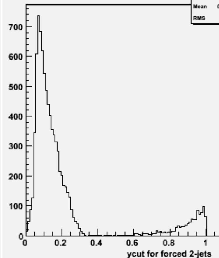
Ycut for 2-jets :w100876 e2e2cse1n1_o
