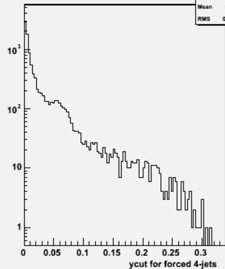
Ycut for 4-jets :w100876 e2e2cse1n1_o
