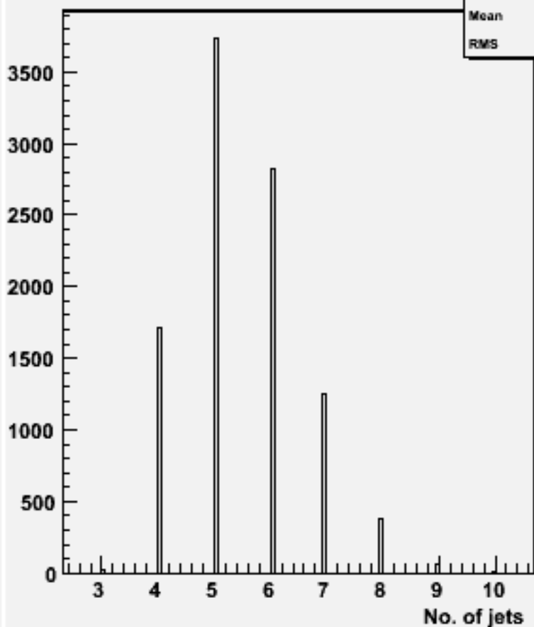
No. jets (ycut=0.001) : w100876 e2e2cse1n1_o
