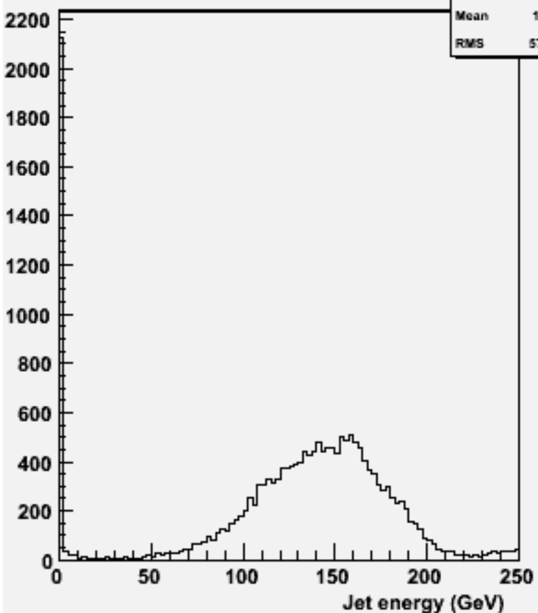
energy for 2-jets :w100876 e2e2cse1n1_o
