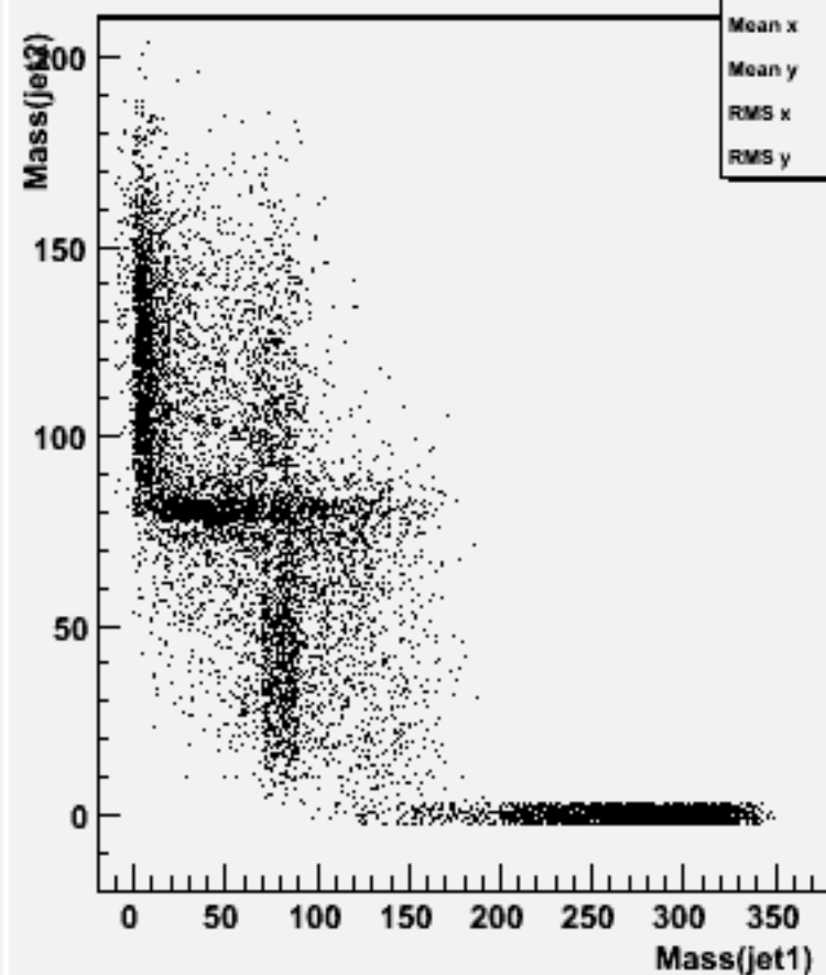
Jet mass for forced 2-jets : w100876 e2e2cse1n1_o
