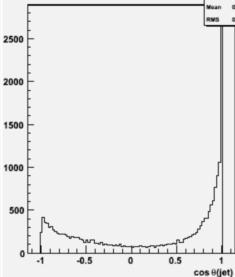
cos \theta for 2-jets :w100876 e2e2cse1n1_o
