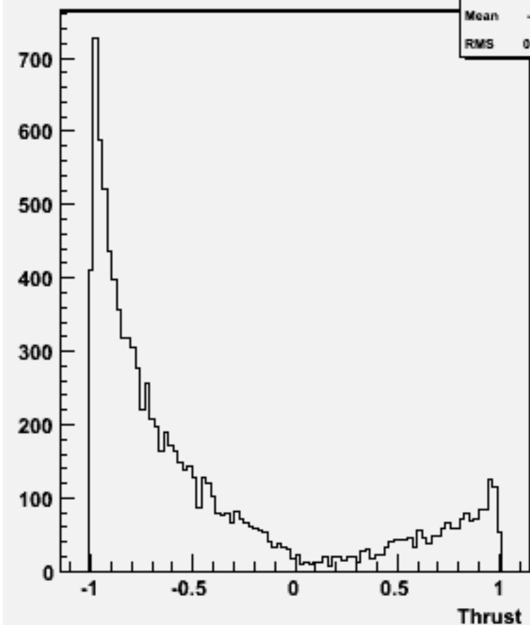
cos \Theta (thrust) w100876 e2e2cse1n1_o
