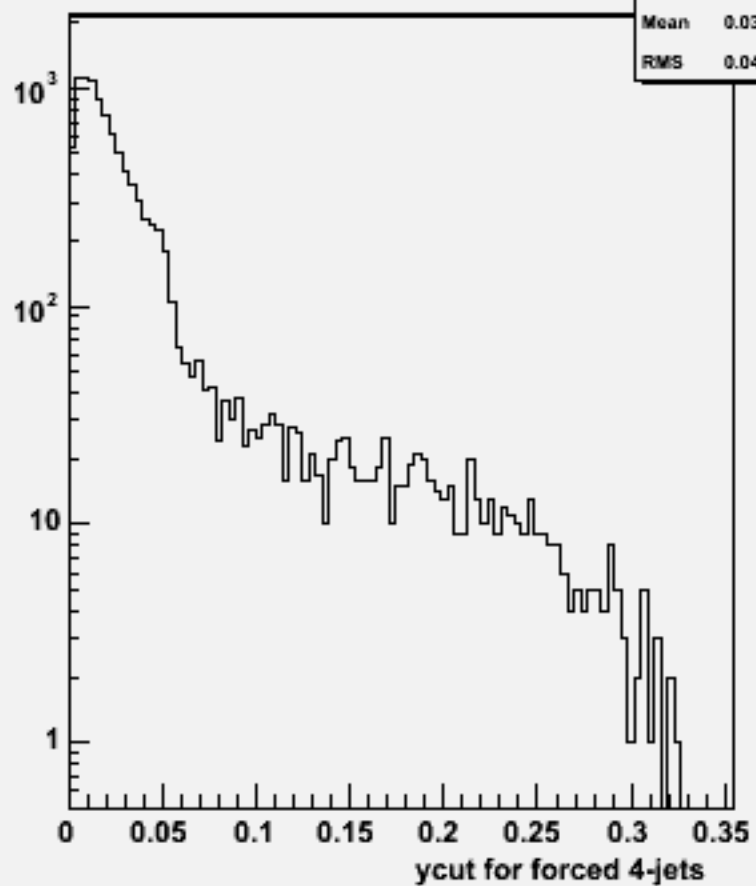
Ycut for 4-jets :w100873 e2e2udsc_o
