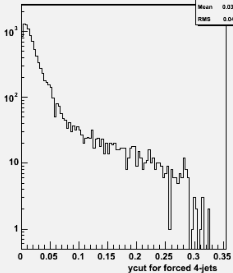
Ycut for 4-jets :w100869 e2e2uddu_o
