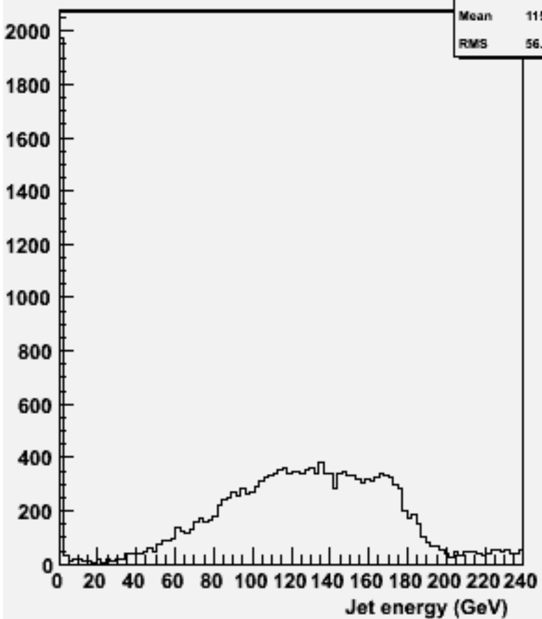
energy for 2-jets :w100865 e2e2ude3n3_o
