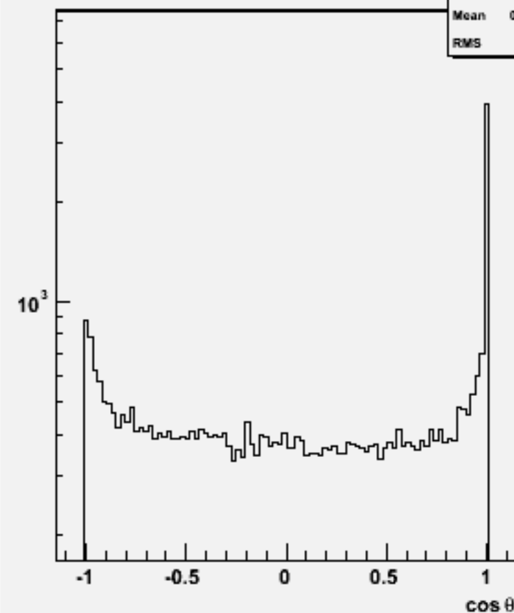
Jet cos \theta (All jets)w100865 e2e2ude3n3_o
