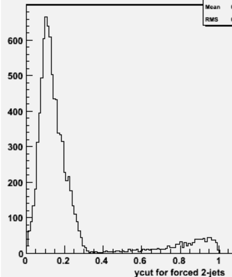
Ycut for 2-jets :w100865 e2e2ude3n3_o
