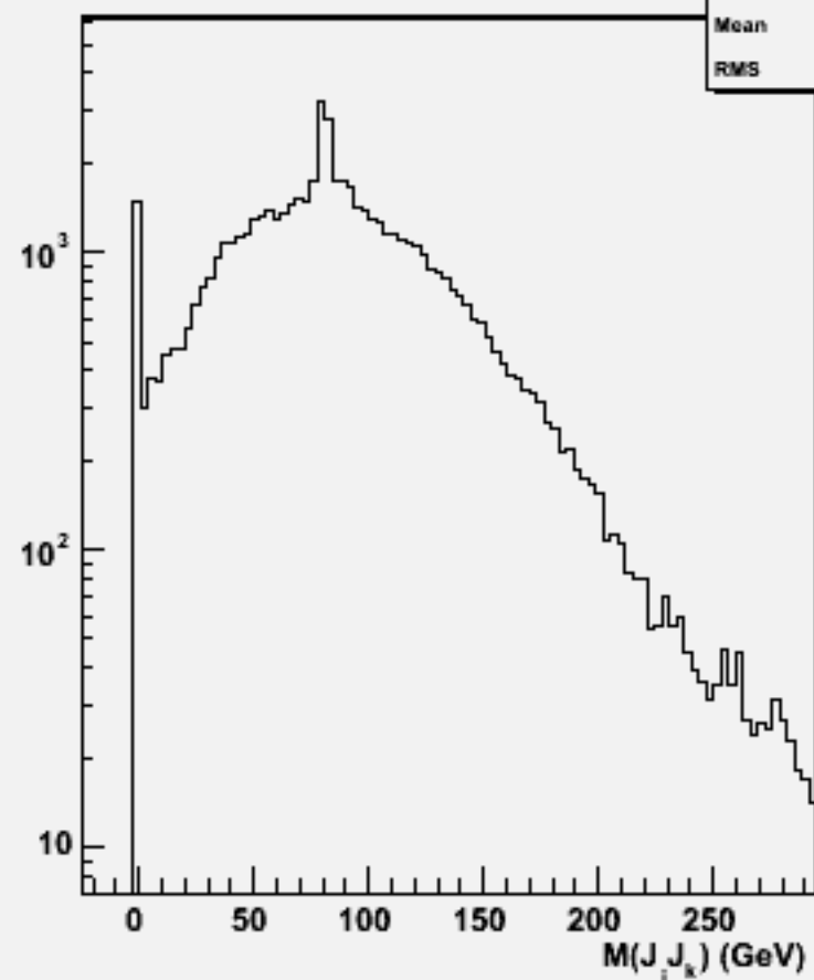
2jets mass(All comb)w100865 e2e2ude3n3_o
