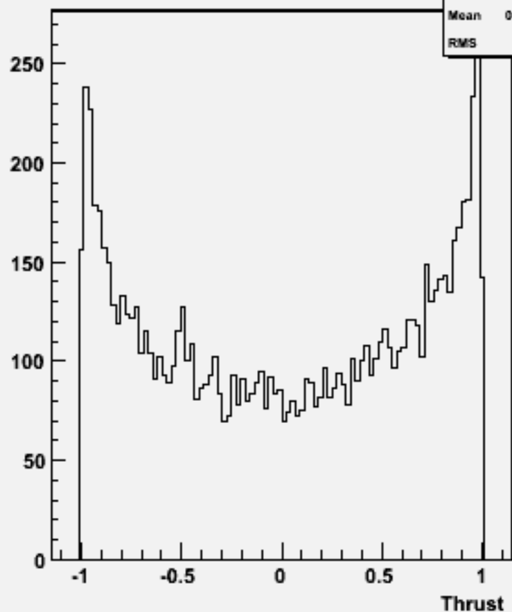
cos \Theta (thrust) w100865 e2e2ude3n3_o
