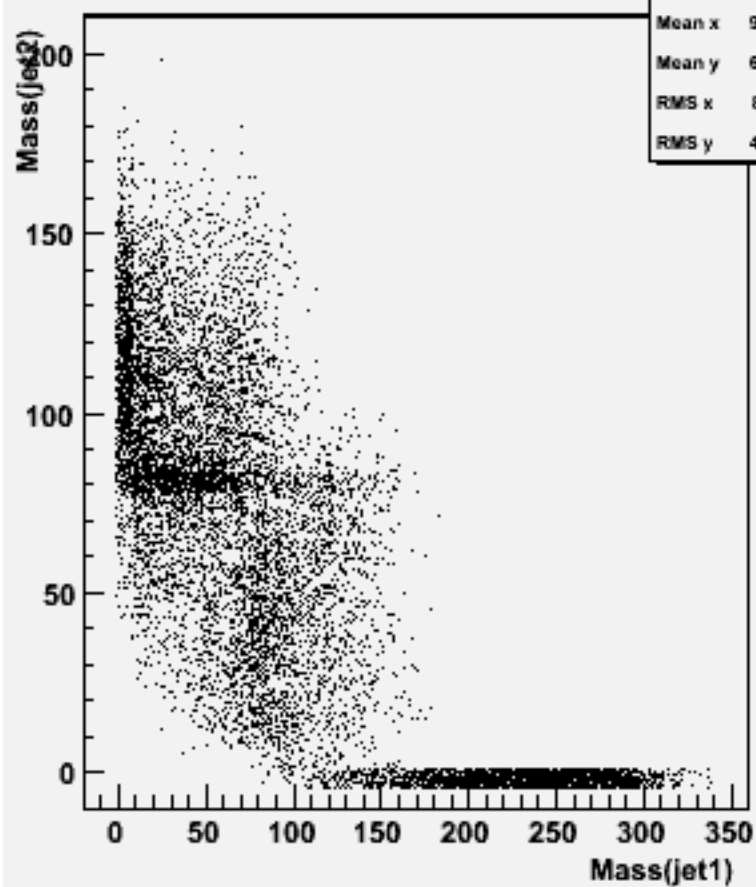
Jet mass for forced 2-jets : w100865 e2e2ude3n3_o
