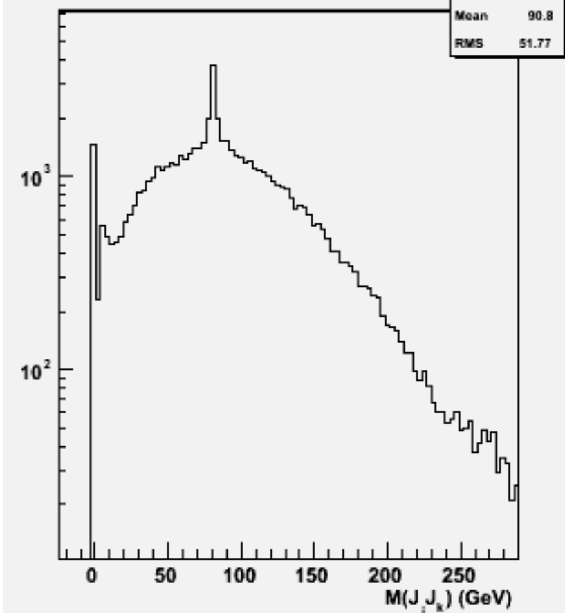
2jets mass(All comb)w100864 e2e2ude3n3_o
