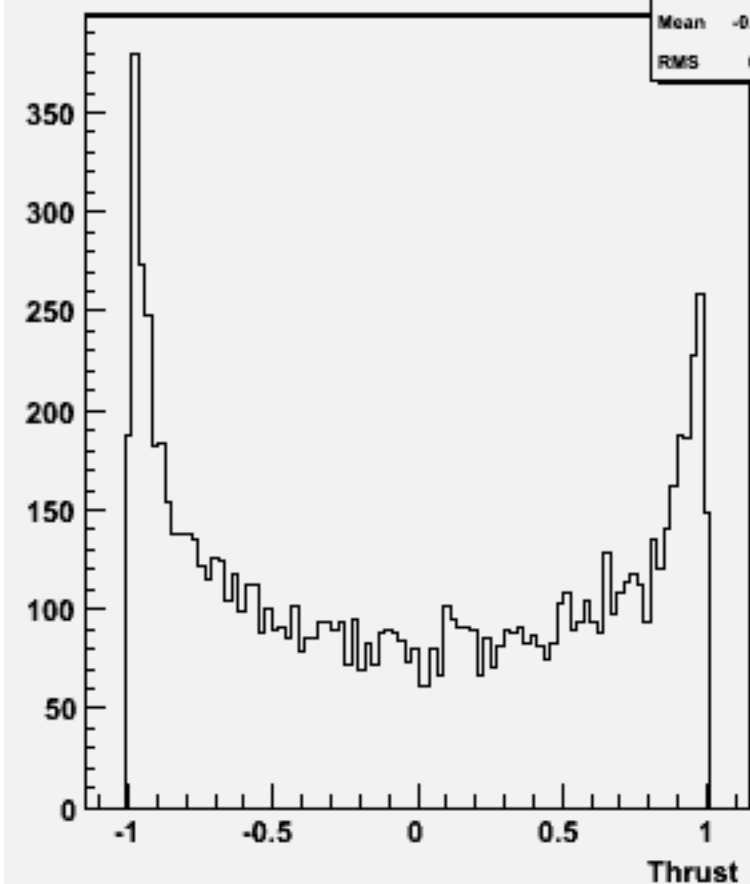
cos \Theta (thrust) w100864 e2e2ude3n3_o
