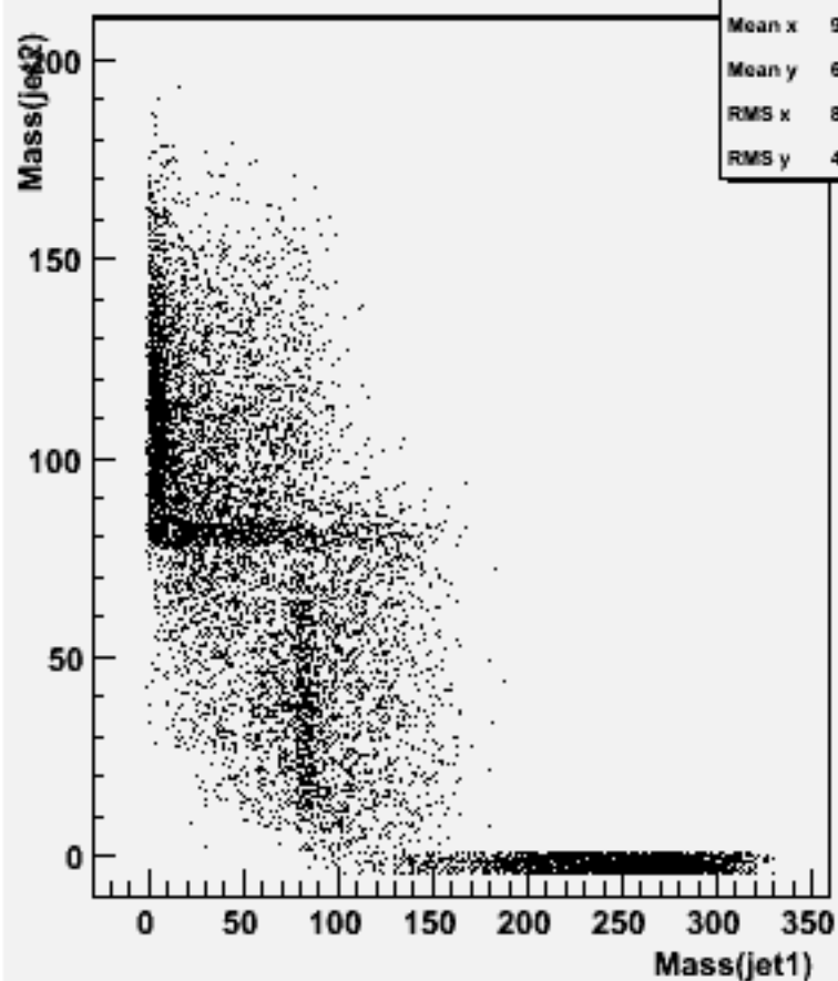
Jet mass for forced 2-jets : w100864 e2e2ude3n3_o
