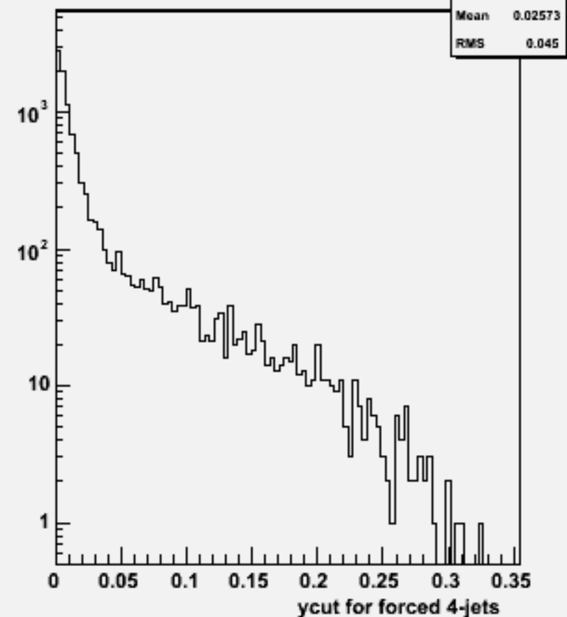
Ycut for 4-jets :w100864 e2e2ude3n3_o
