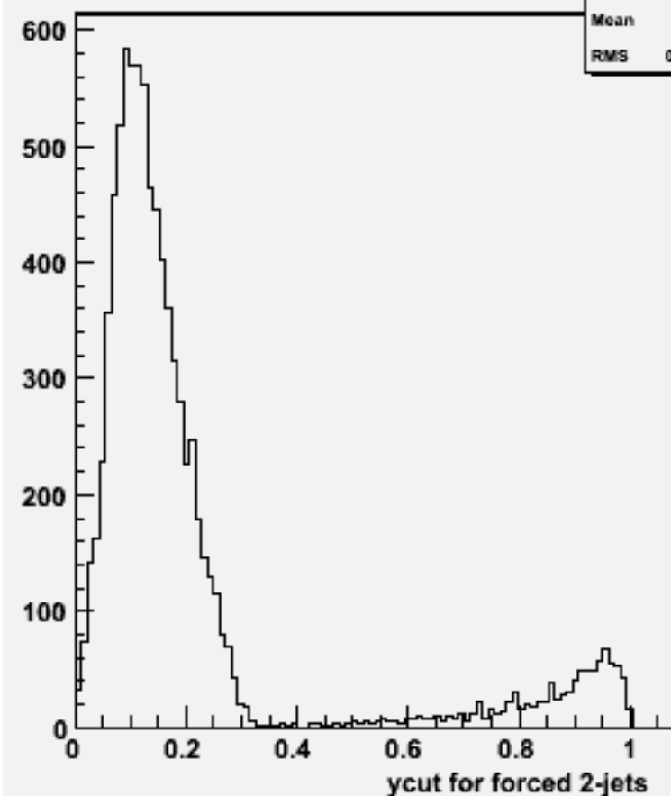
Ycut for 2-jets :w100864 e2e2ude3n3_o
