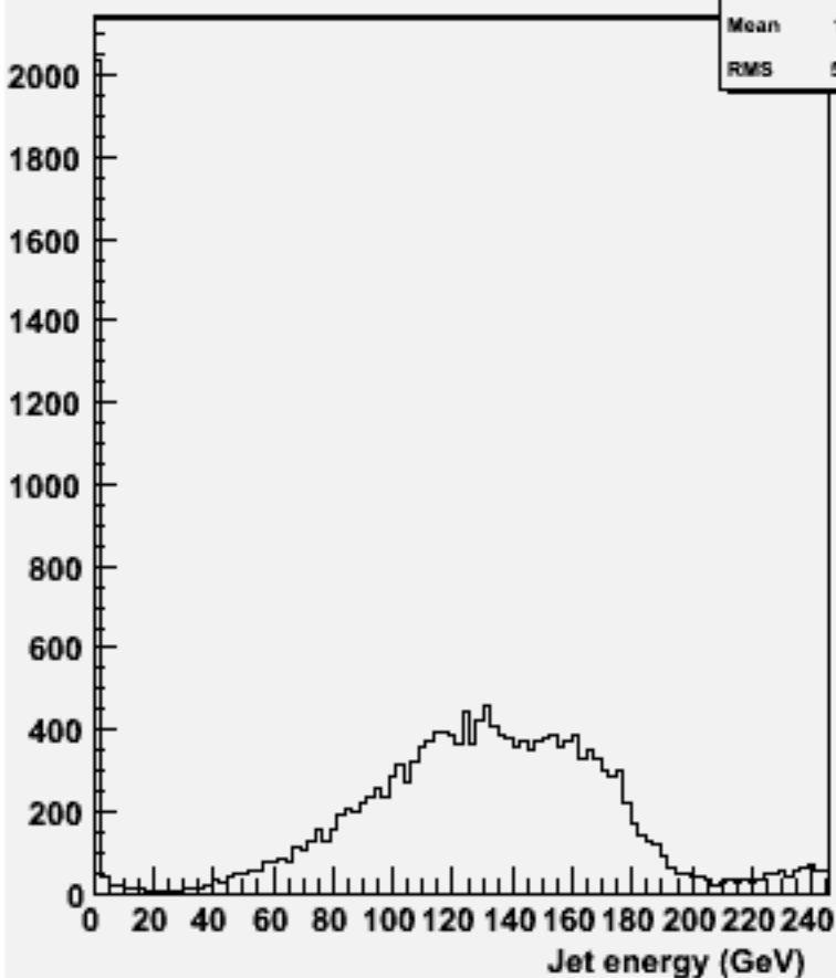
energy for 2-jets :w100864 e2e2ude3n3_o
