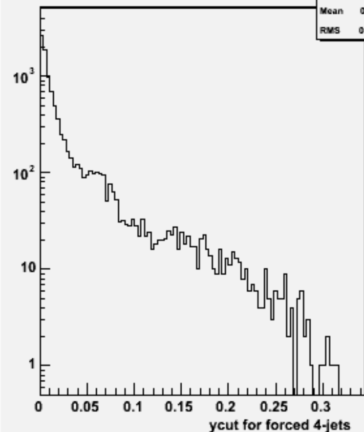
Ycut for 4-jets :w100860 e2e2ude2n2_o
