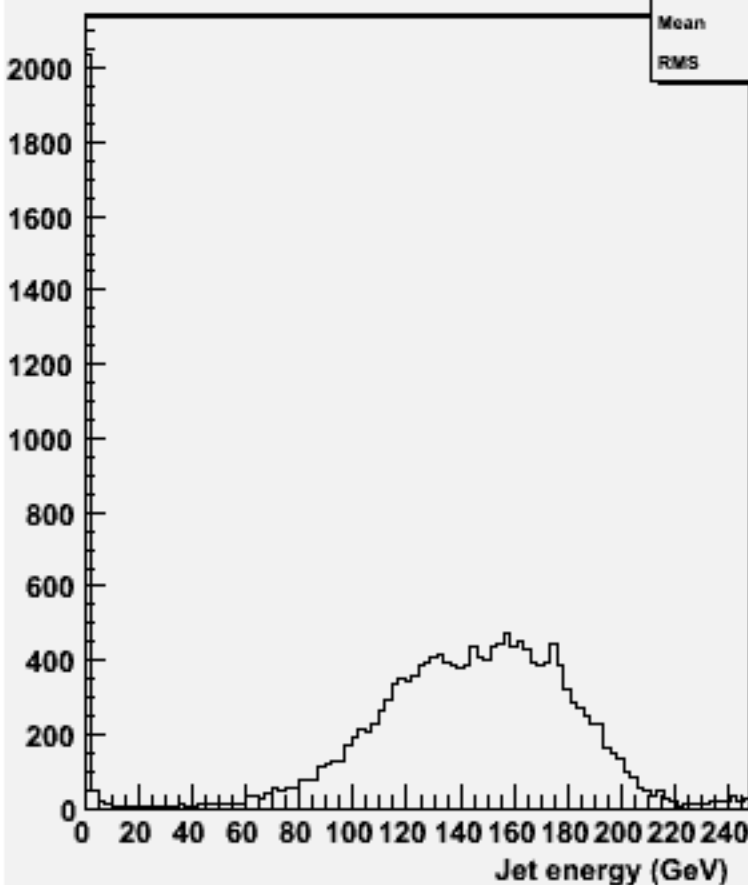
energy for 2-jets :w100860 e2e2ude2n2_o
