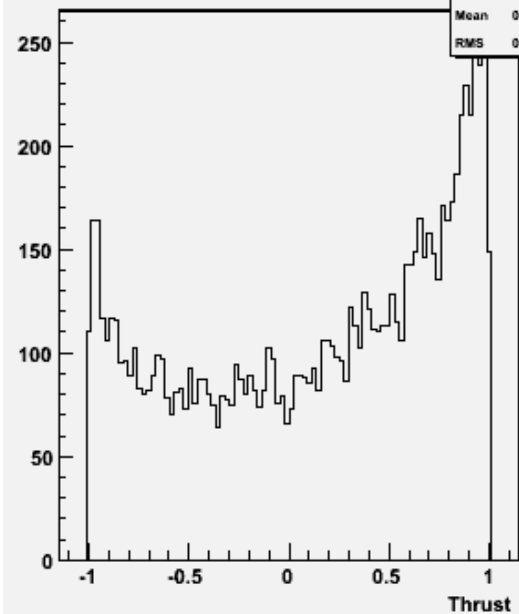
cos \Theta (thrust) w100857 e2e2ude1n1_o
