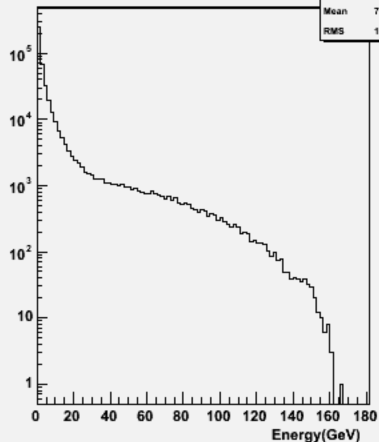
Particle Energy : w100857 e2e2ude1n1_o
