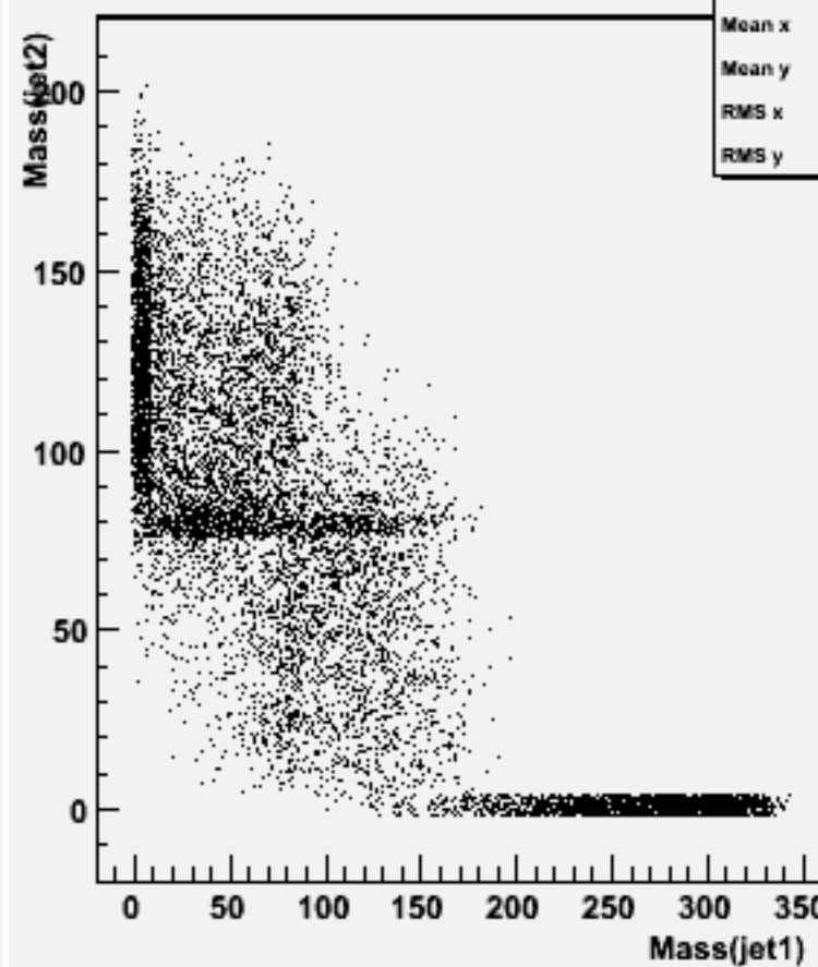
Jet mass for forced 2-jets : w100857 e2e2ude1n1_o
