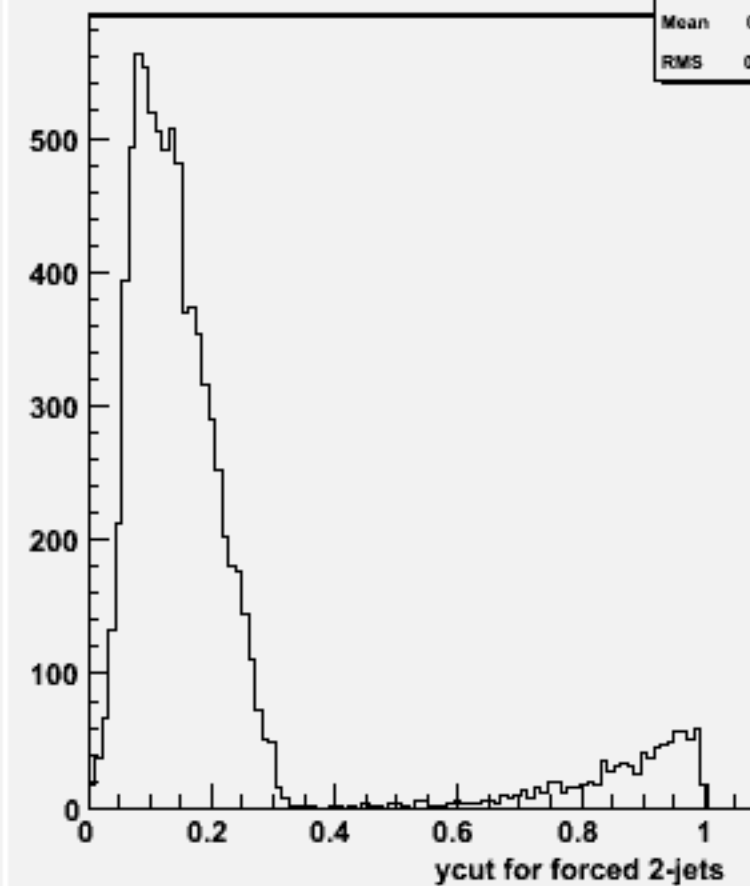
Ycut for 2-jets :w100857 e2e2ude1n1_o
