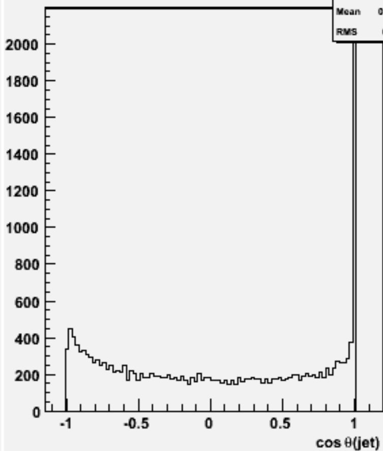
cos \theta for 2-jets :w100857 e2e2ude1n1_o
