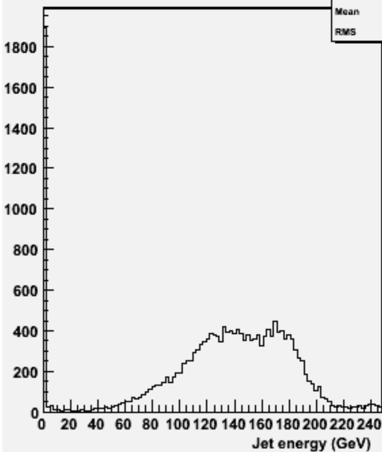
energy for 2-jets :w100857 e2e2ude1n1_o
