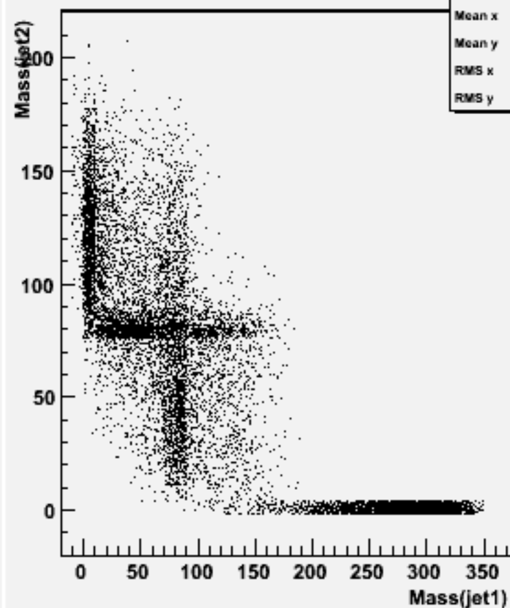
Jet mass for forced 2-jets : w100856 e2e2ude1n1_o
