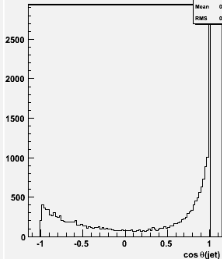
cos \theta for 2-jets :w100856 e2e2ude1n1_o
