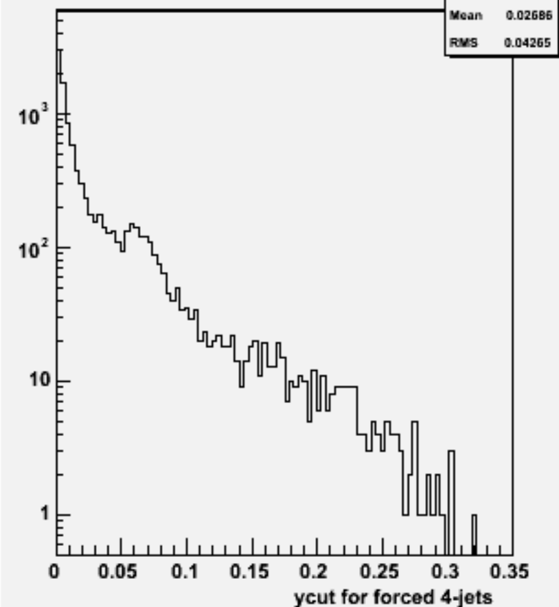
Ycut for 4-jets :w100856 e2e2ude1n1_o
