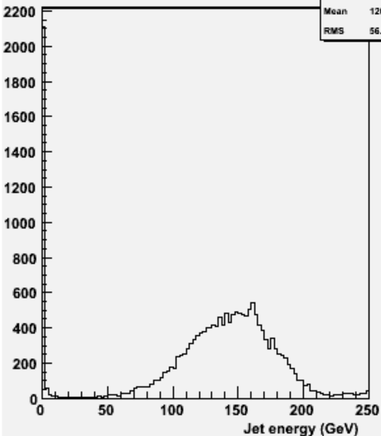
energy for 2-jets :w100856 e2e2ude1n1_o
