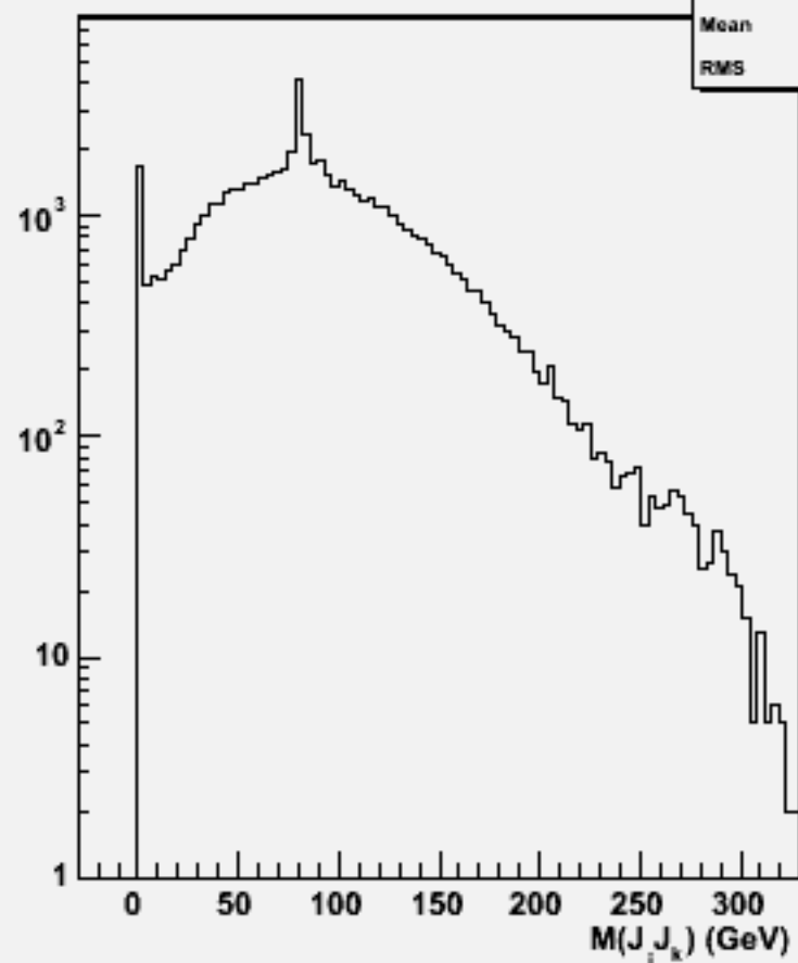
2jets mass(All comb)w100848 e2e2n3e3du_o
