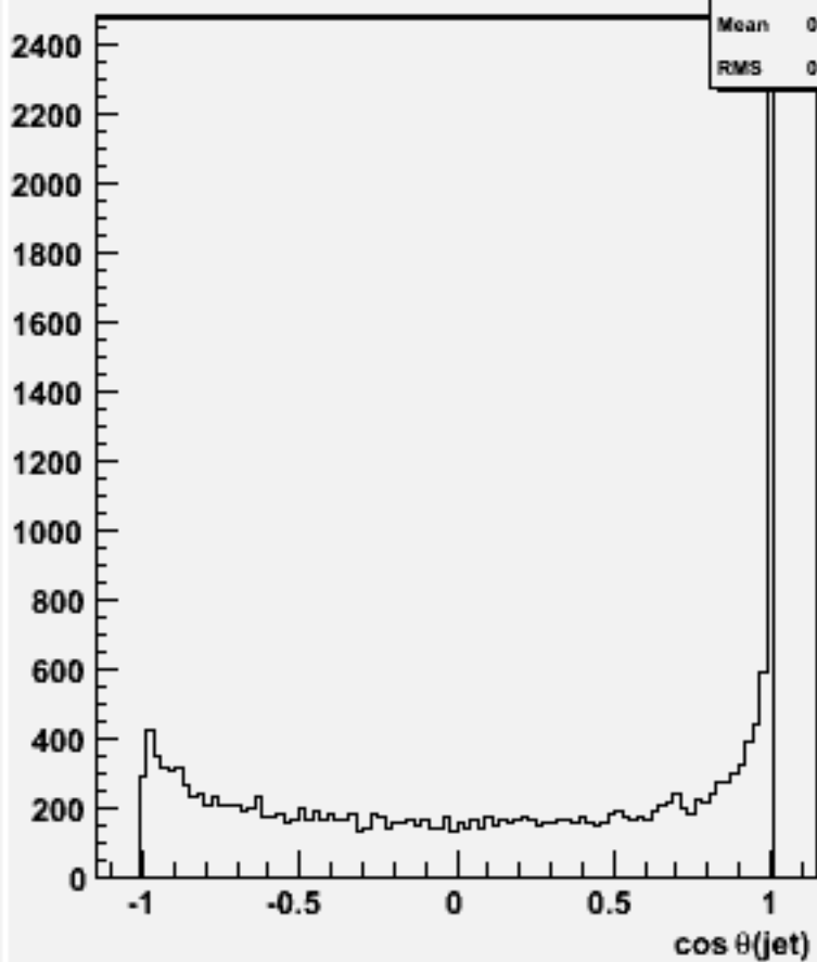
cos \theta for 2-jets :w100848 e2e2n3e3du_o
