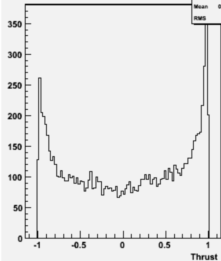
cos \Theta (thrust) w100848 e2e2n3e3du_o
