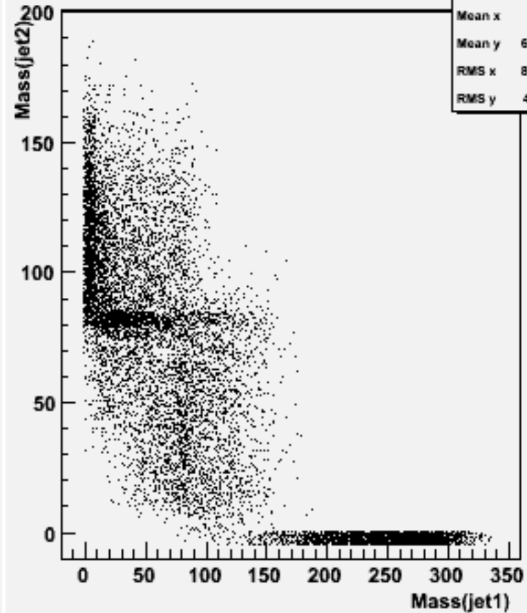
Jet mass for forced 2-jets : w100848 e2e2n3e3du_o
