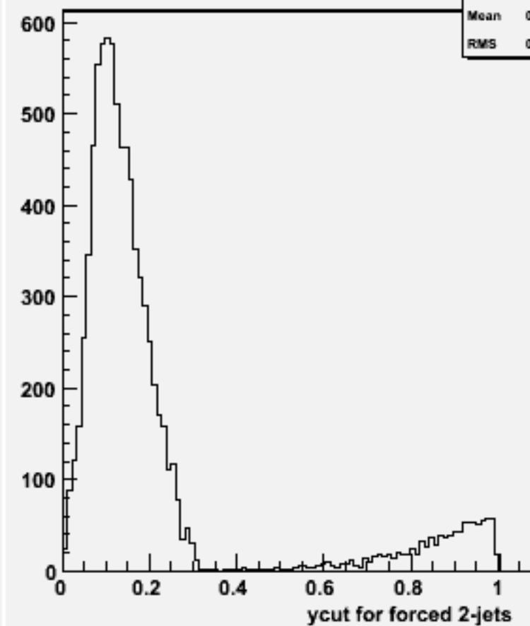
Ycut for 2-jets :w100848 e2e2n3e3du_o
