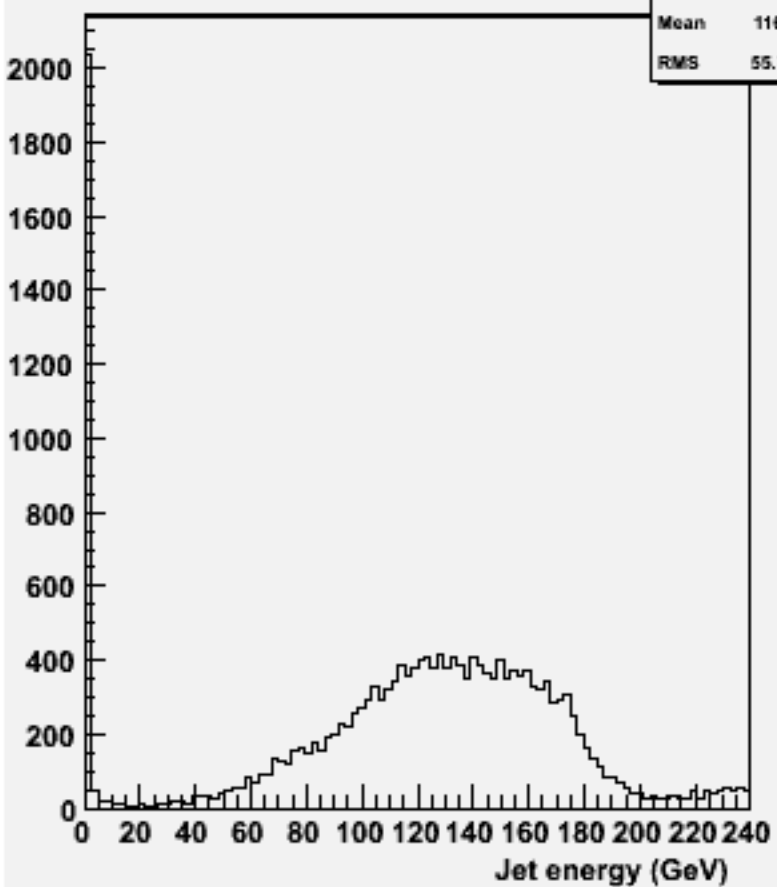
energy for 2-jets :w100848 e2e2n3e3du_o
