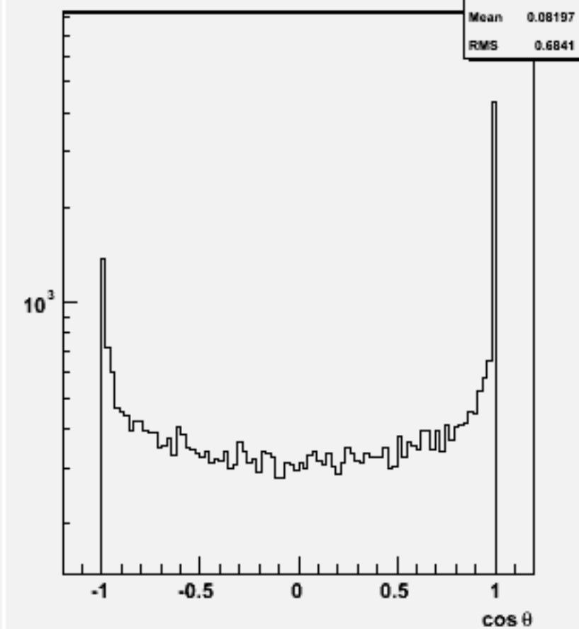
Jet cos \theta (All jets)w100841 e2e2n3e3e2n2_o
