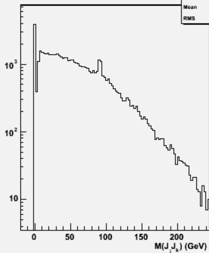
2jets mass(All comb)w100841 e2e2n3e3e2n2_o
