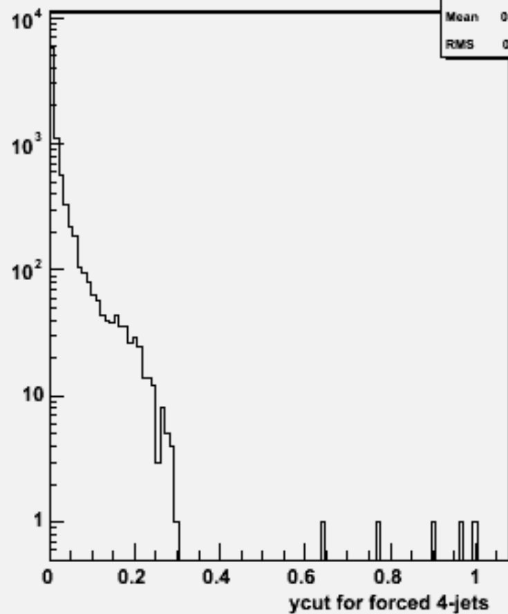
Ycut for 4-jets :w100841 e2e2n3e3e2n2_o
