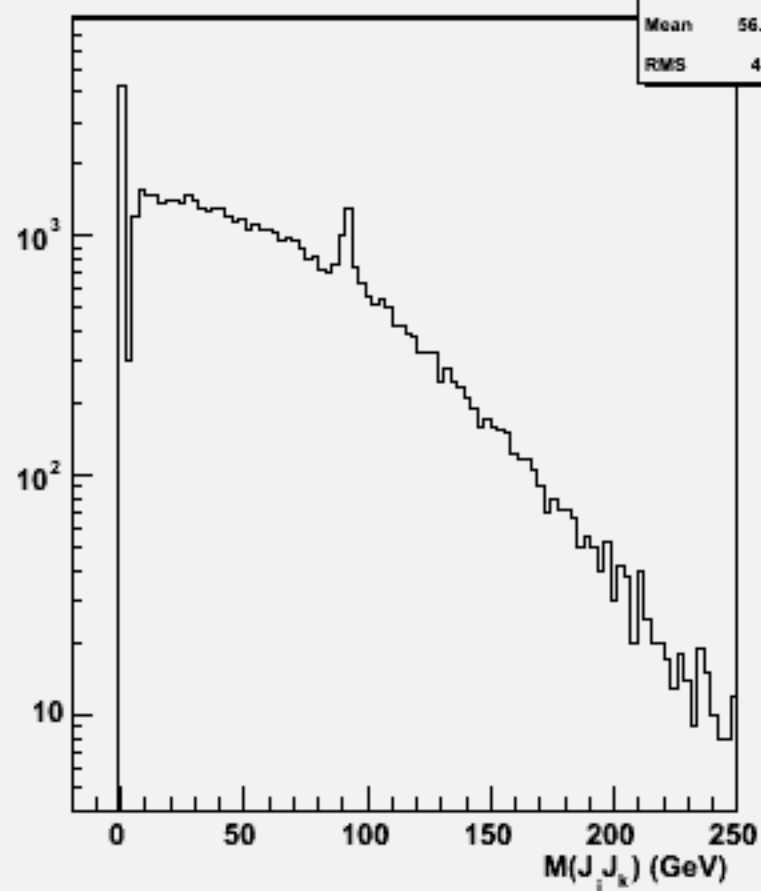
2jets mass(All comb)w100837 e2e2n3e3e1n1_o
