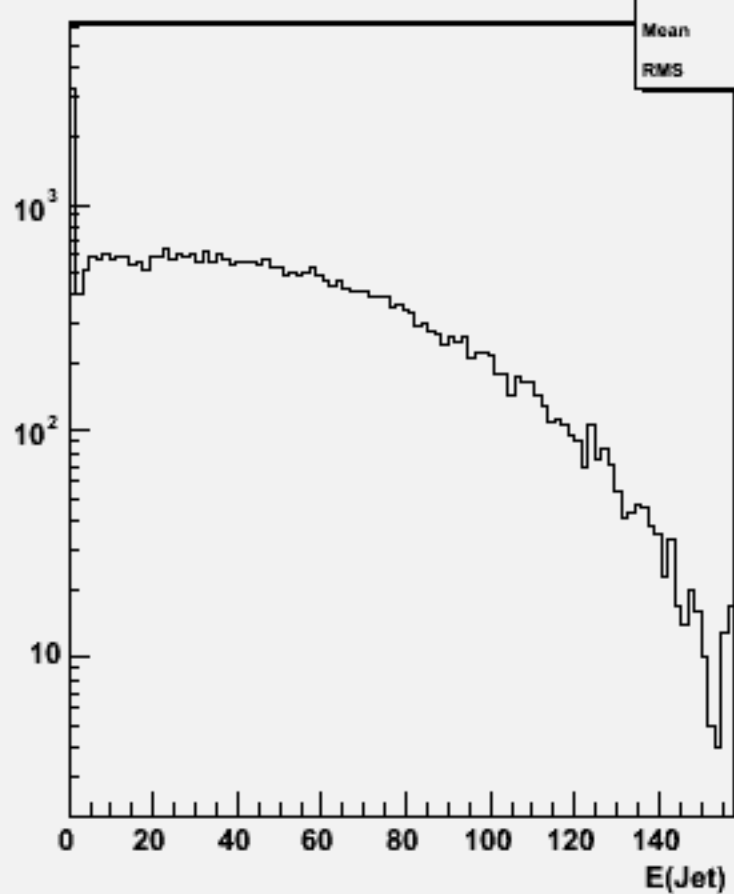
Jet energies(All jets)w100837 e2e2n3e3e1n1_o
