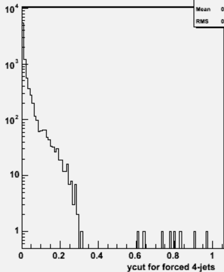
Ycut for 4-jets :w100837 e2e2n3e3e1n1_o
