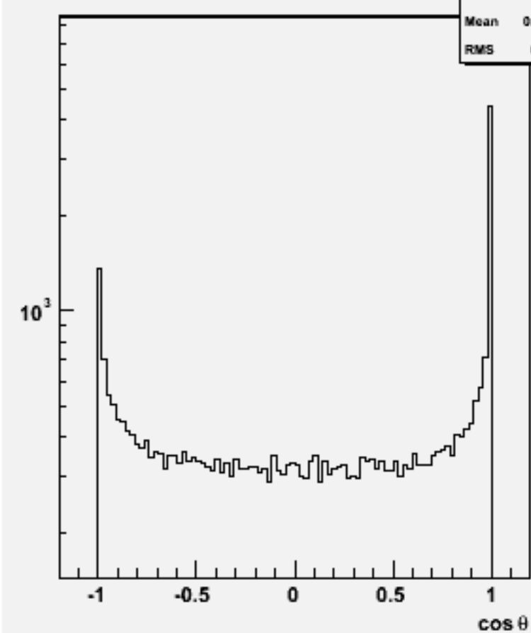
Jet cos \theta (All jets)w100837 e2e2n3e3e1n1_o
