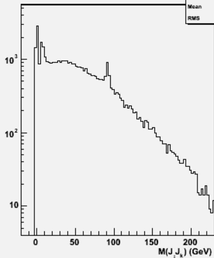
2jets mass(All comb)w100836 e2e2n3e3e1n1_o
