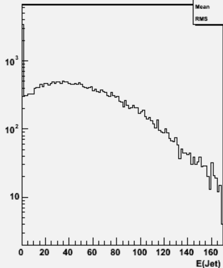
Jet energies(All jets)w100836 e2e2n3e3e1n1_o
