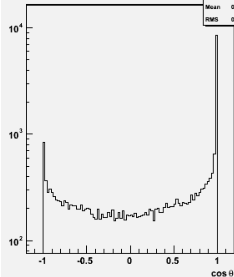
Jet cos \theta (All jets)w100836 e2e2n3e3e1n1_o
