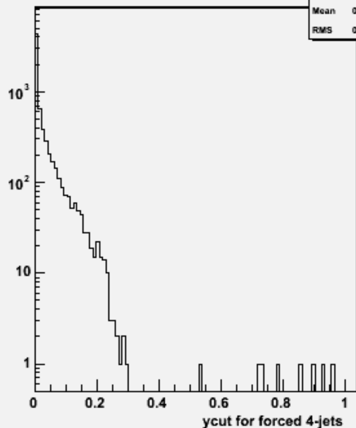
Ycut for 4-jets :w100836 e2e2n3e3e1n1_o
