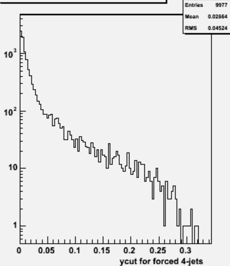
Ycut for 4-jets :w100833 e2e2n2e2sc_o
