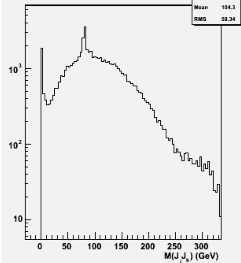
2jets mass(All comb)w100832 e2e2n2e2sc_o
