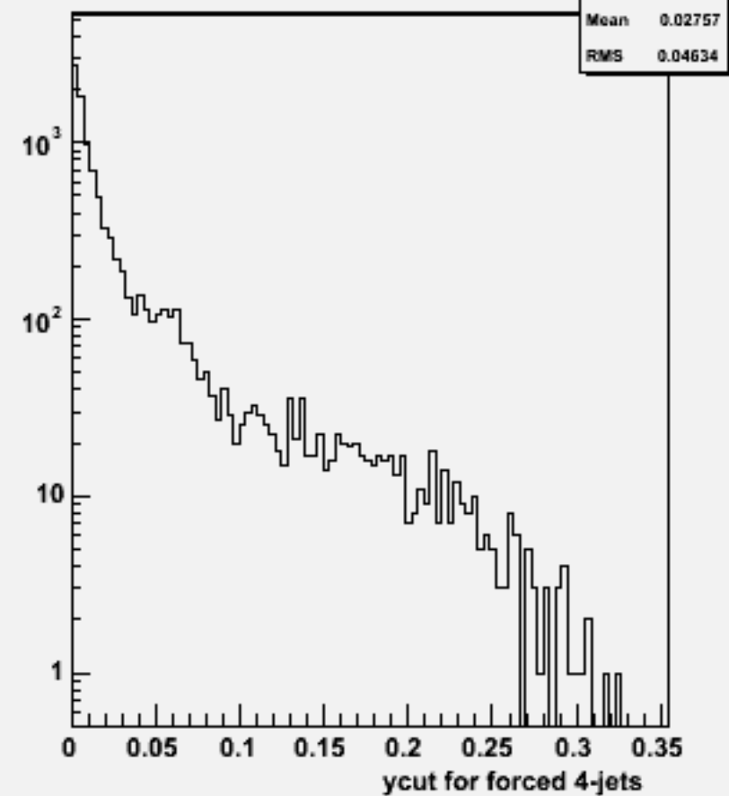
Ycut for 4-jets :w100832 e2e2n2e2sc_o
