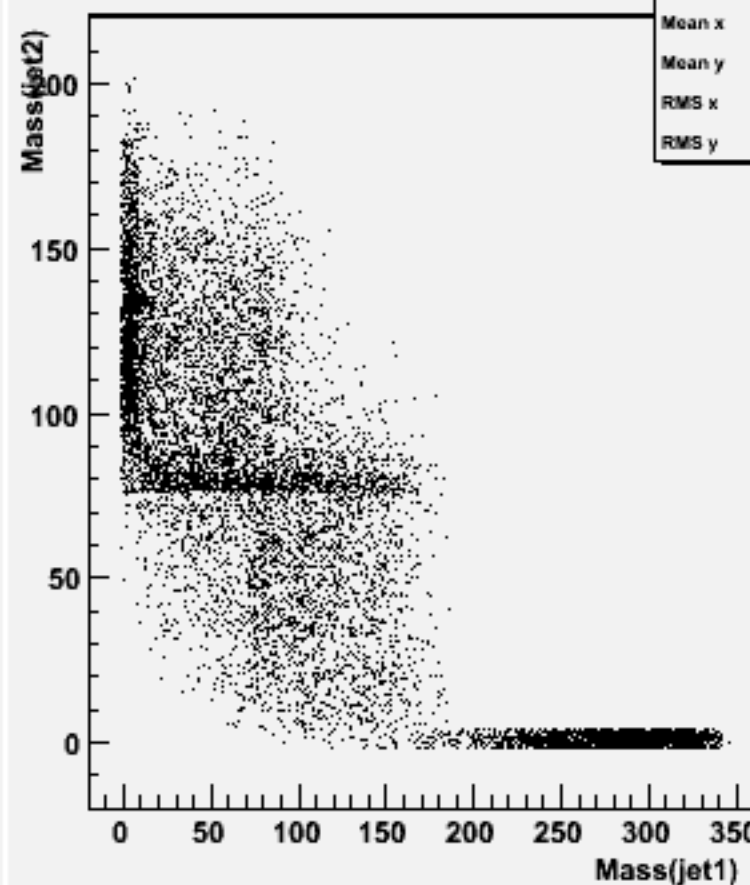
Jet mass for forced 2-jets : w100828 e2e2n2e2du_o
