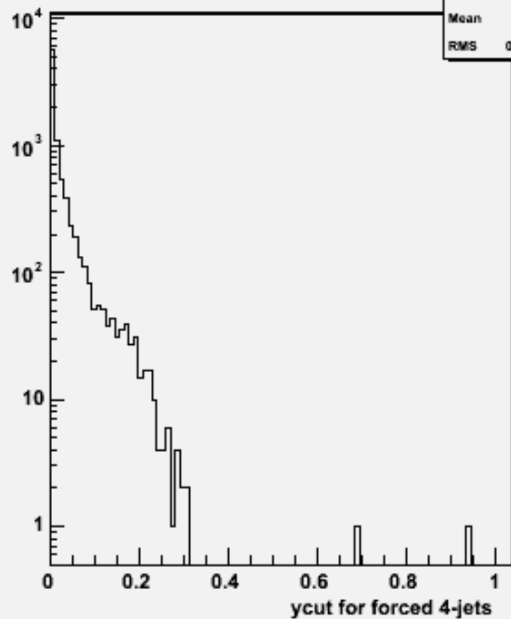
Ycut for 4-jets :w100825 e2e2n2e2e3n3_o
