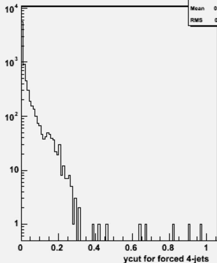
Ycut for 4-jets :w100821 e2e2n2e2e2n2_o
